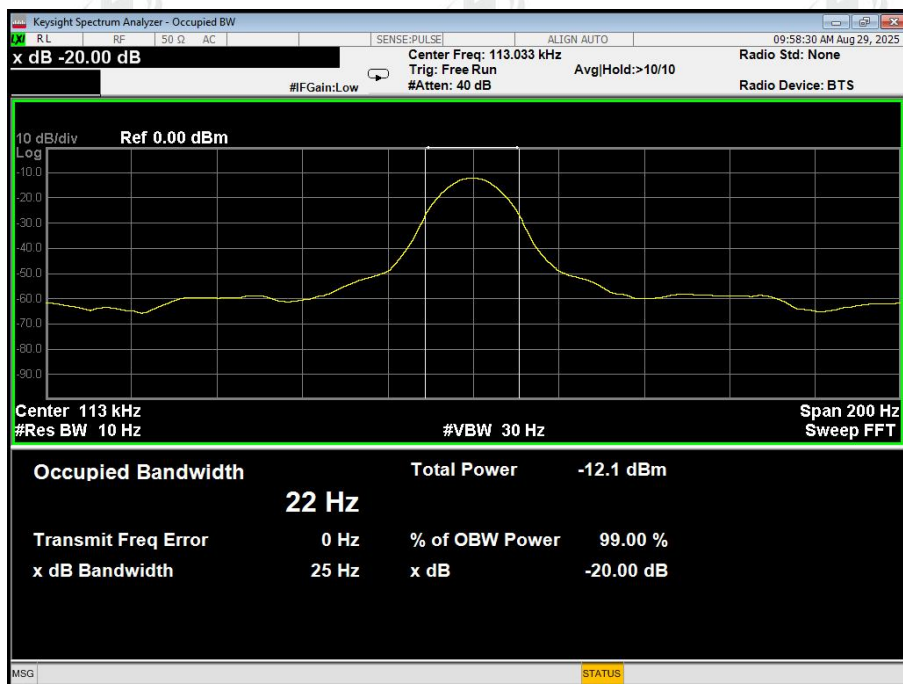
Phone coil (111-205kHz)
