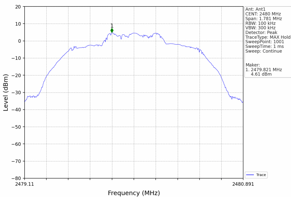
Pi/4DQPSK_2DH5_HCH_2480MHz_Ant1_NTNV
