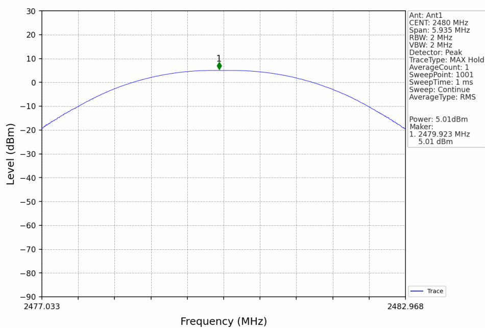
Pi/4DQPSK_2DH5_HCH_2480MHz_Ant1_NTNV
