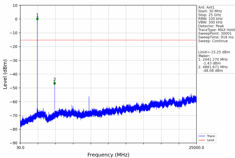
Pi/4DQPSK 2DH5_MCH_2441MHz_Ant1_NTNV
