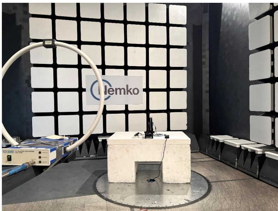
Figure Error! No text of specified style in document.-1: Radiated emissions setup photo – 150 kHz to 30 MHz
