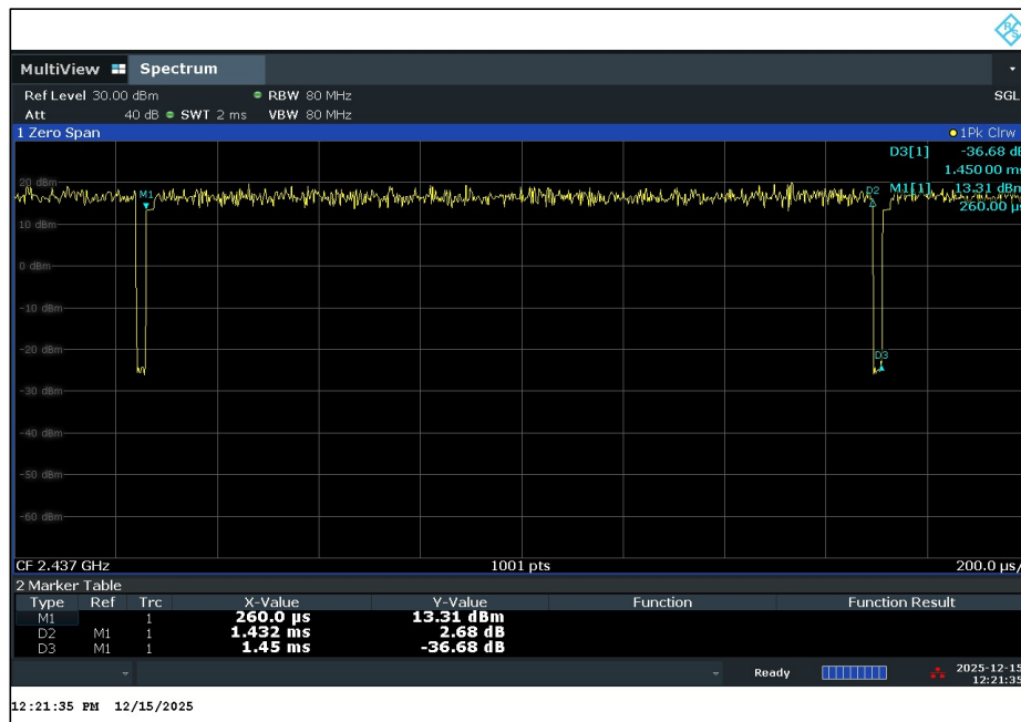
802.11g 6Mbps 2437 MHz Duty Cycle
