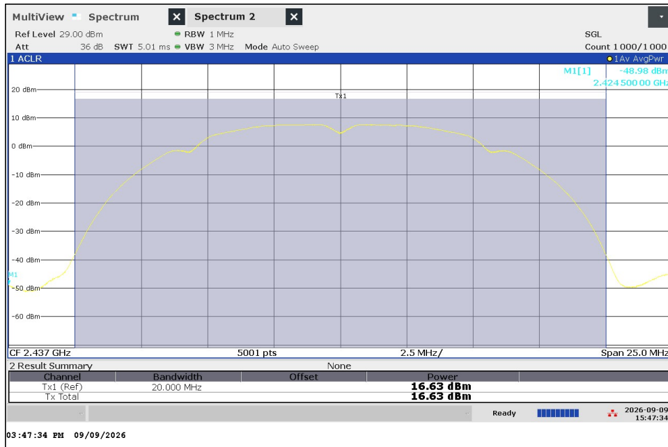
802.11b 1 Mbps 2437 MHz Output Power
