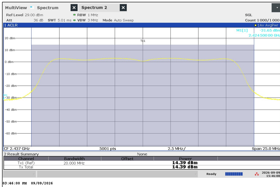
802.11g 6 Mbps 2437 MHz Output Power
