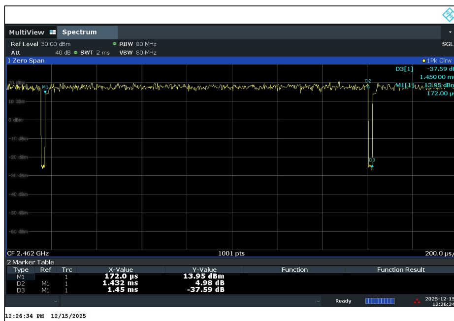
802.11g 6Mbps 2462 MHz Duty Cycle
