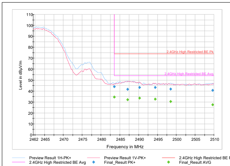
802.11b 1Mbps 2462 MHz – Restricted Band-edge
