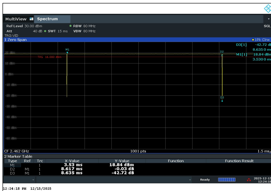
802.11b 1Mbps 2462 MHz Duty Cycle
