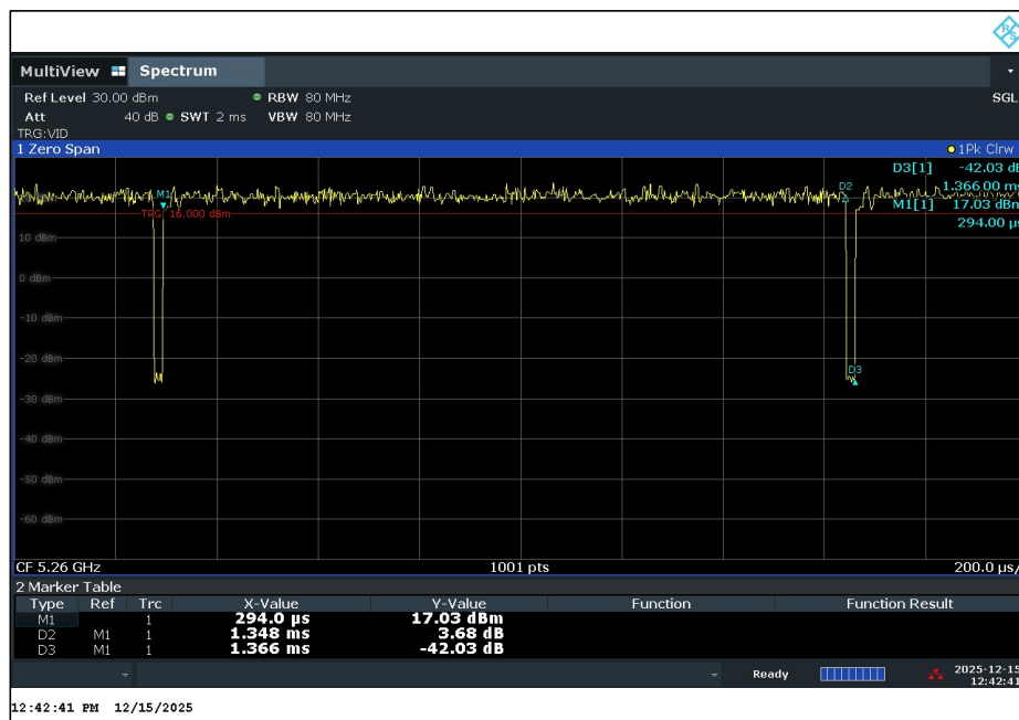
802.11n HT0 5260 MHz Duty Cycle
