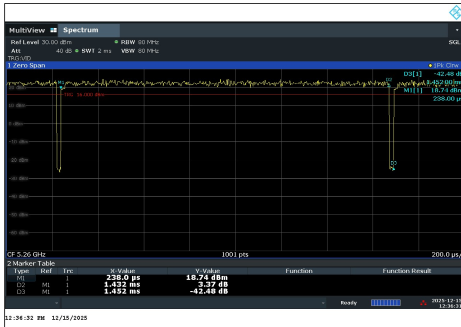
802.11a 6 Mbps 5260 MHz Duty Cycle
