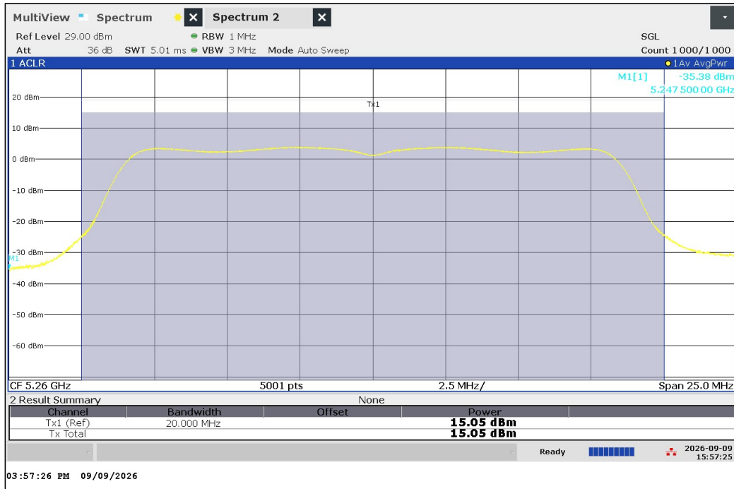
802.11a 6 Mbps 5260 MHz Output Power
