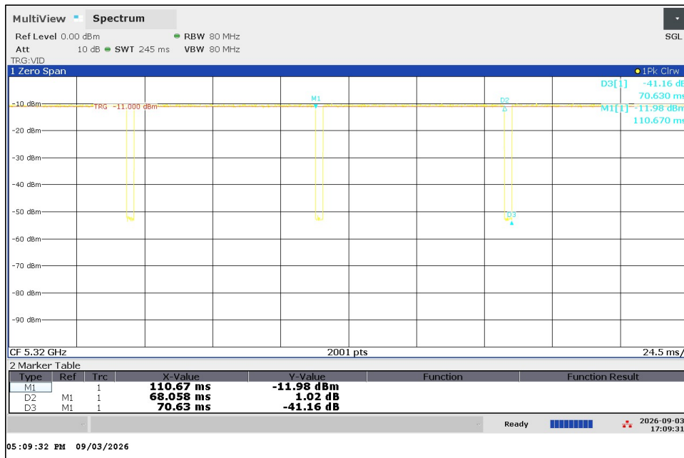
802.11a 6Mbps 5320 MHz Duty Cycle
