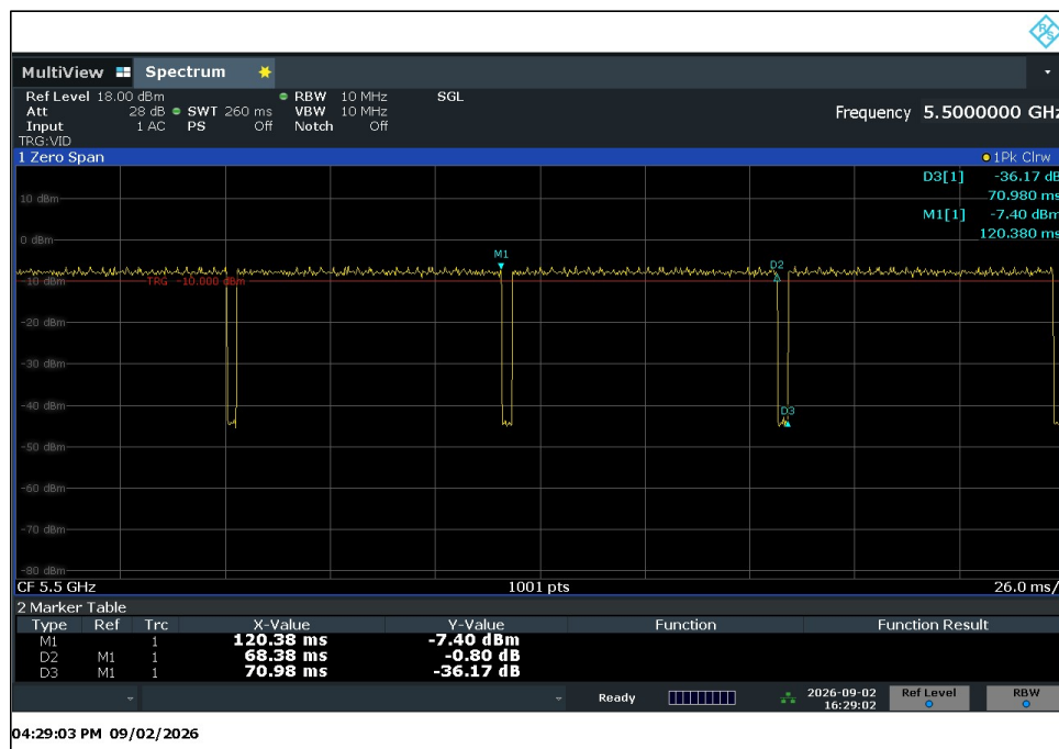
802.11a 6Mbps 5500 MHz Duty Cycle
