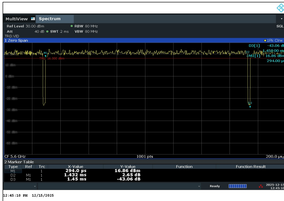
802.11a 6 Mbps 5600 MHz Duty Cycle
