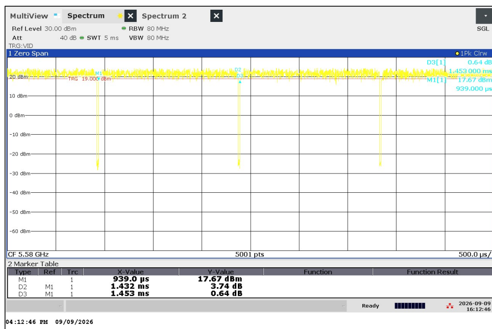
802.11a 6Mbps 5580 MHz Duty Cycle
