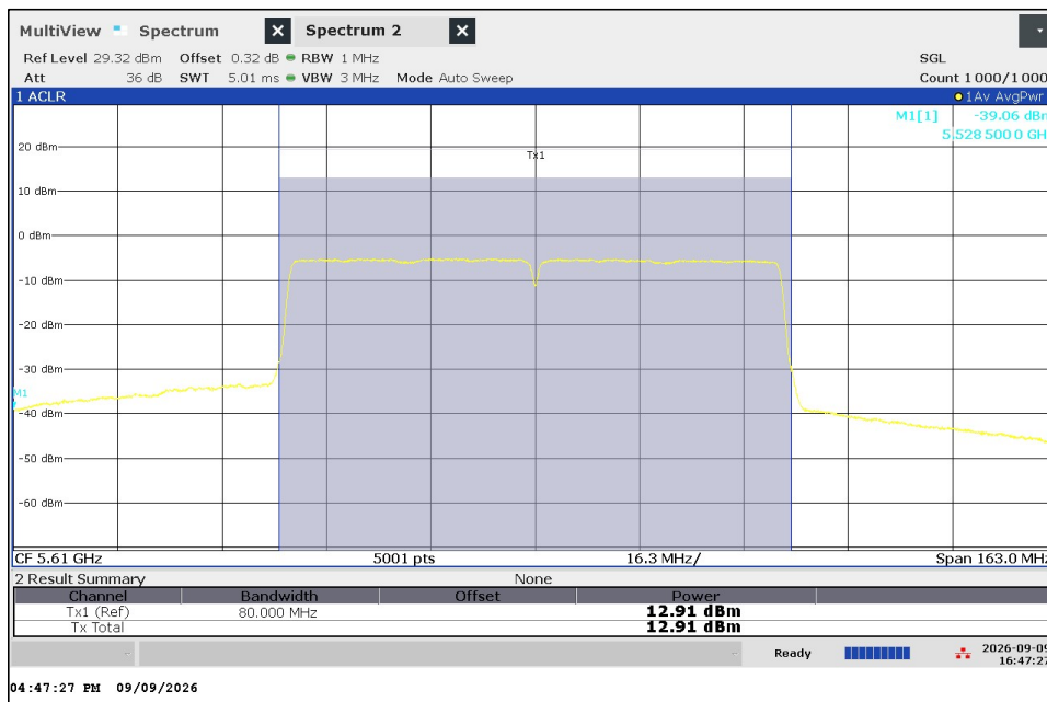
802.11ac (80 MHz) VHT0 5610 MHz Output Power
