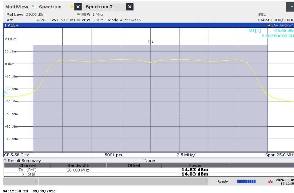
802.11a 6 Mbps 5580 MHz Output Power
