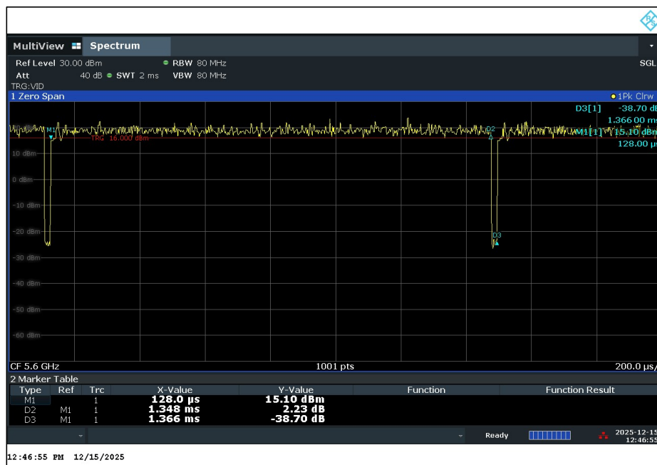
802.11ac HT0 5600 MHz Duty Cycle
