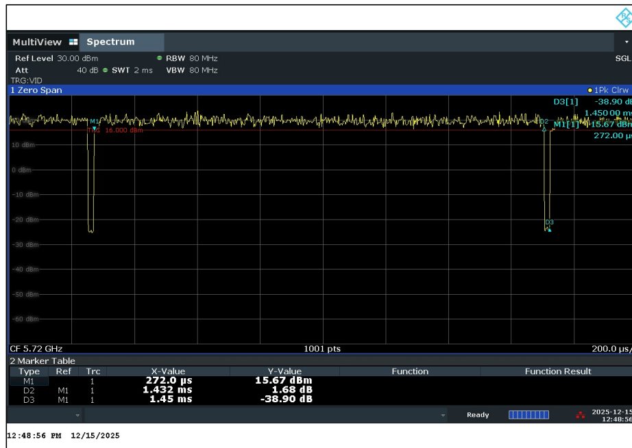
802.11a 6 Mbps 5720 MHz Duty Cycle
