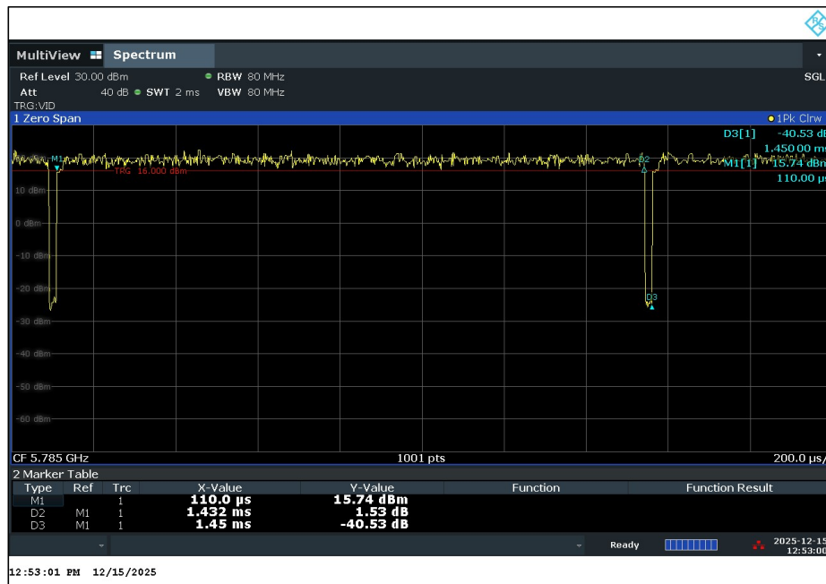
802.11a 6 Mbps 5785 MHz Duty Cycle
