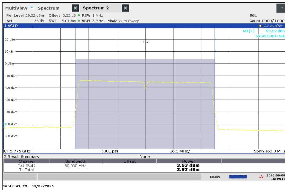
802.11ac (80 MHz) VHT0 5775 MHz Output Power
