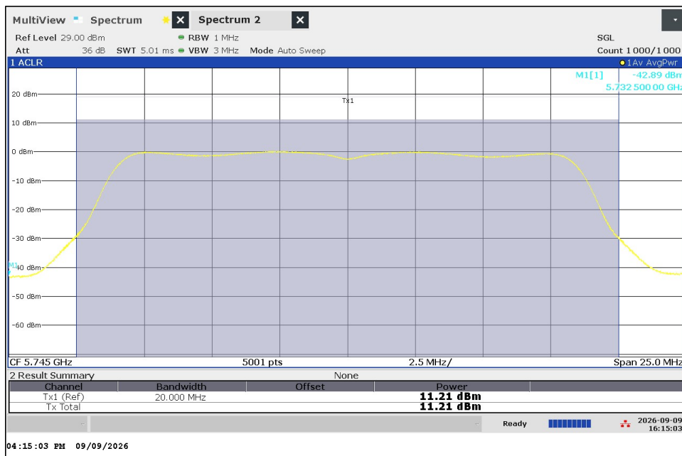
802.11a 6 Mbps 5745 MHz Output Power
