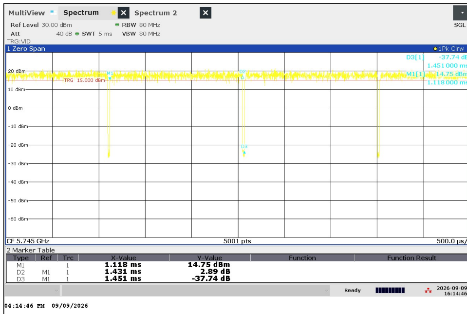
802.11a 6Mbps 5745 MHz Duty Cycle
