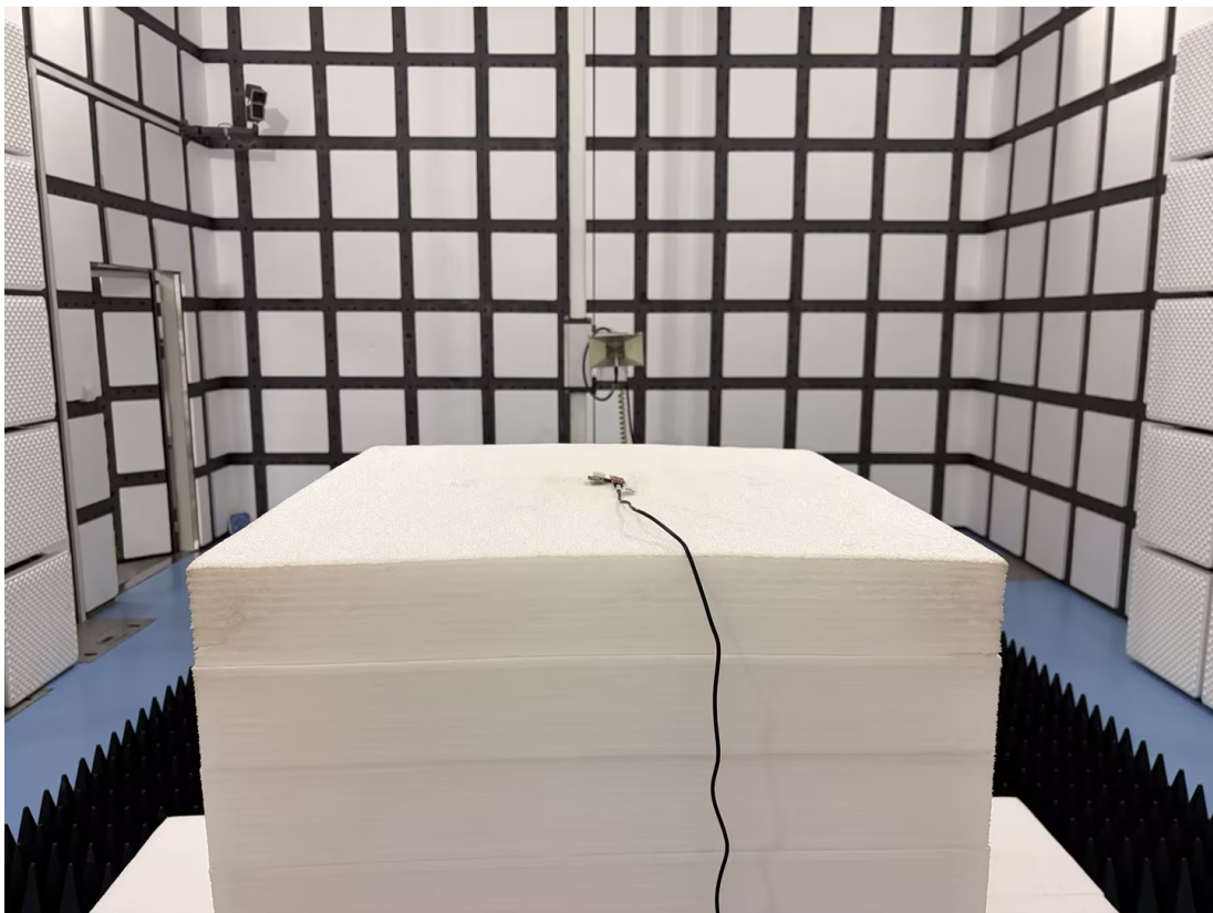
Radiation Emission - Front View (1GHz-18GHz)
