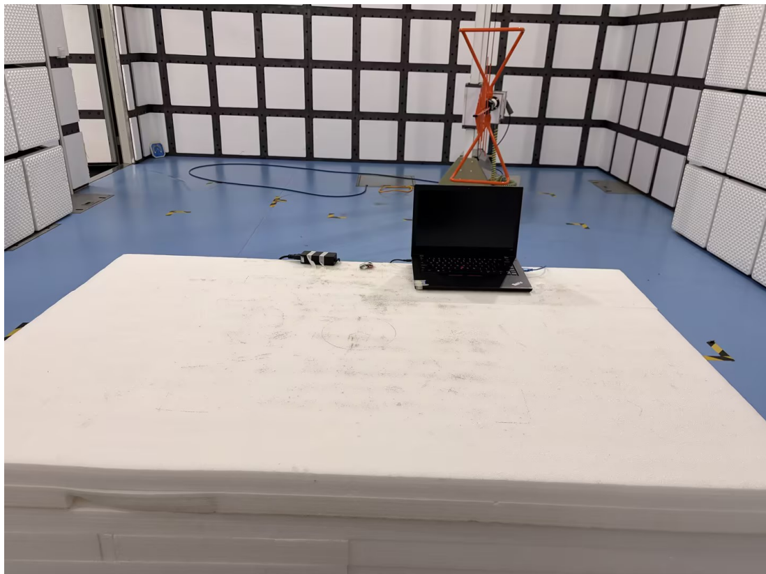
Radiation Emission - Front View (Below 1GHz)
