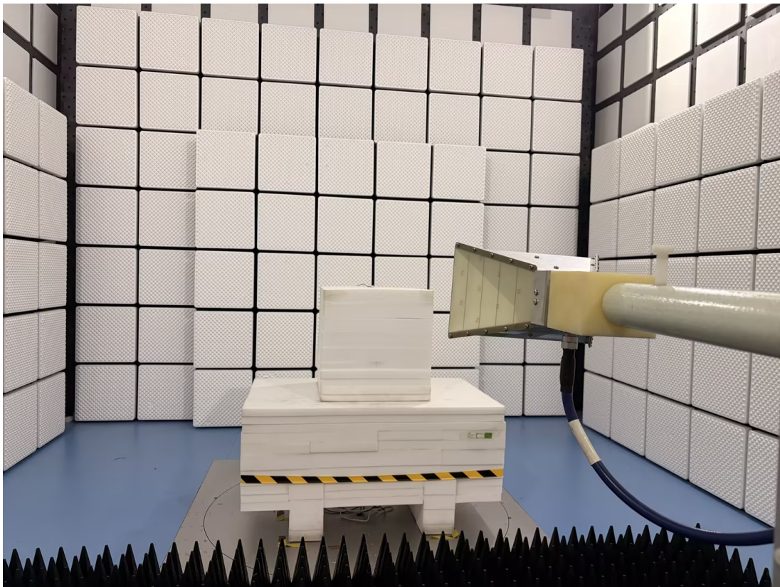
Radiation Emission - Front View (Above 18GHz)
