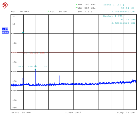
BLE_1M_Middle_Channel
