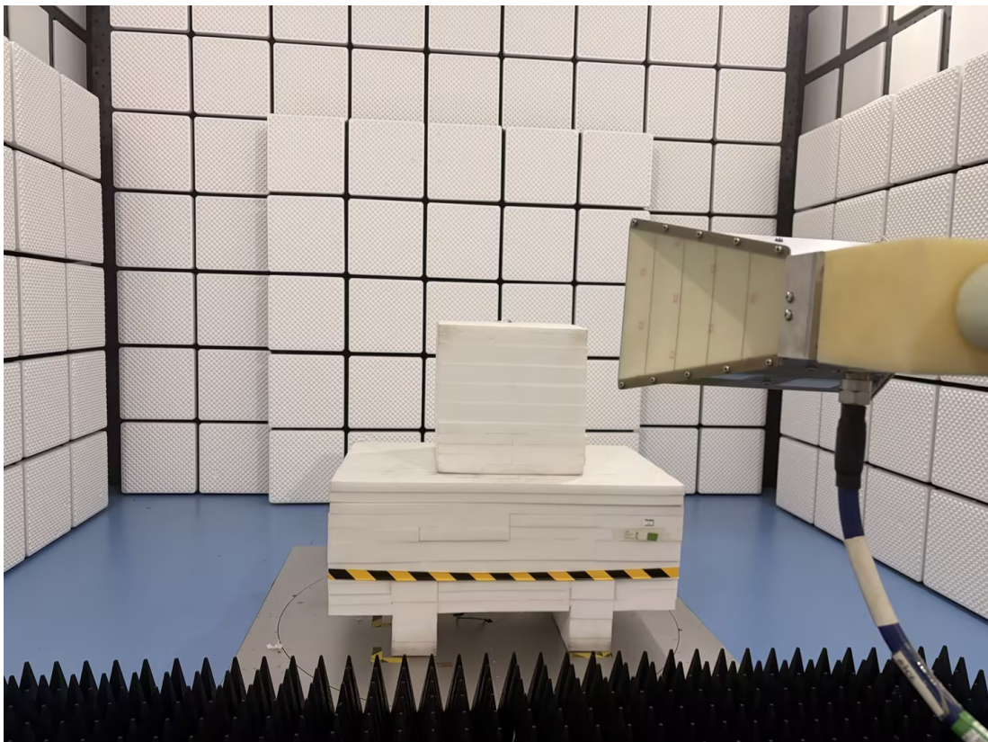
Radiation Emission - Front View (1GHz-18GHz)
