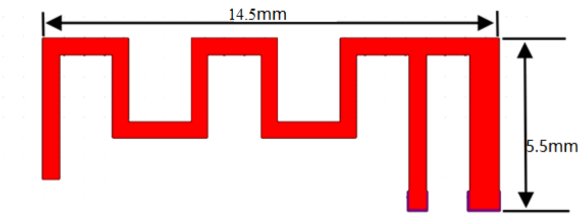
Antenna Length
