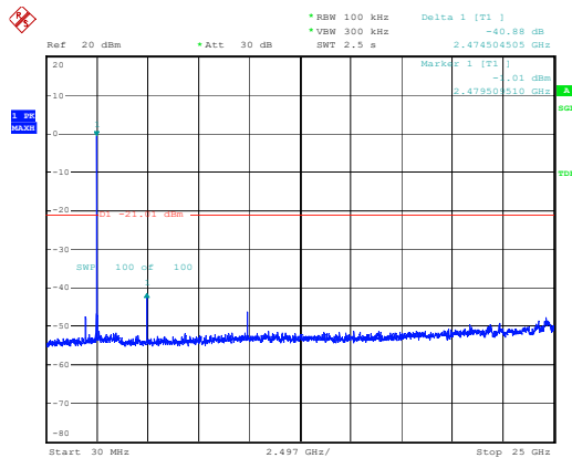
DH5_High
