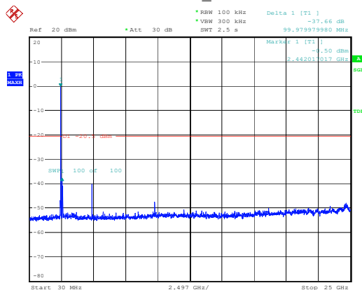
2DH5_Middle
