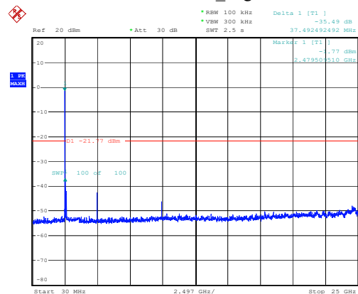
2DH5_High
