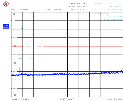
DH5_Middle
