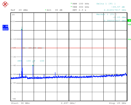
DH5_Low
