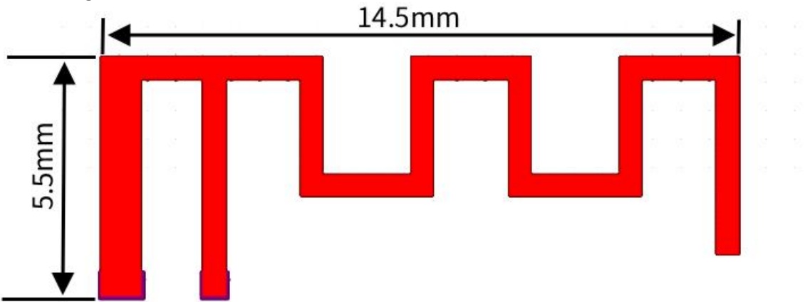
Antenna Length
