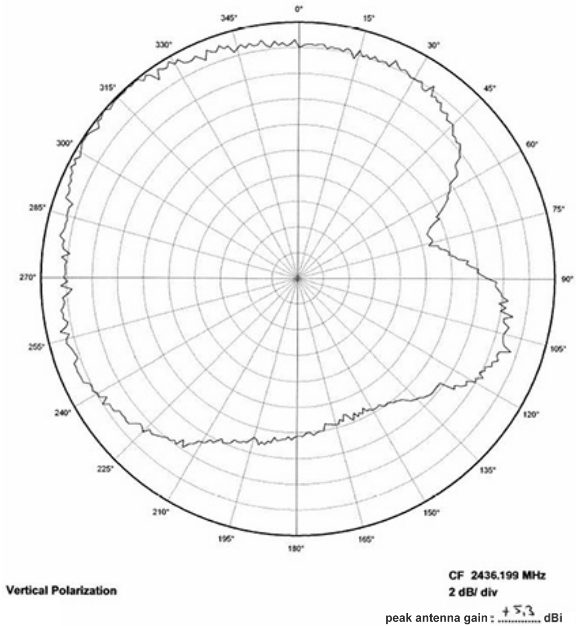
Figure 11: YZ Plane
