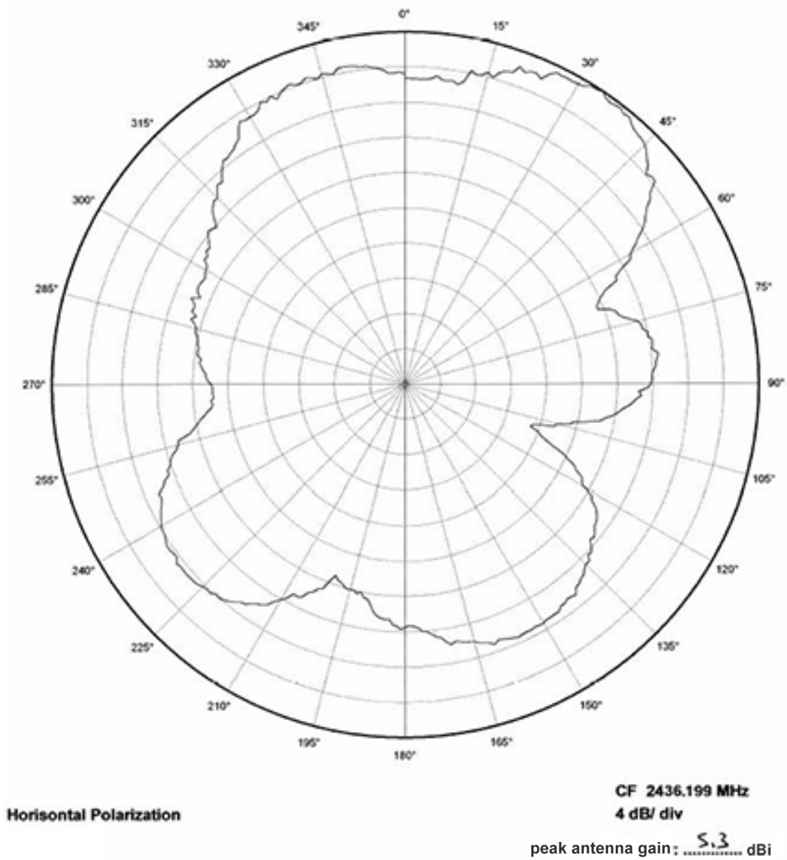
Figure 10: XZ Plane
