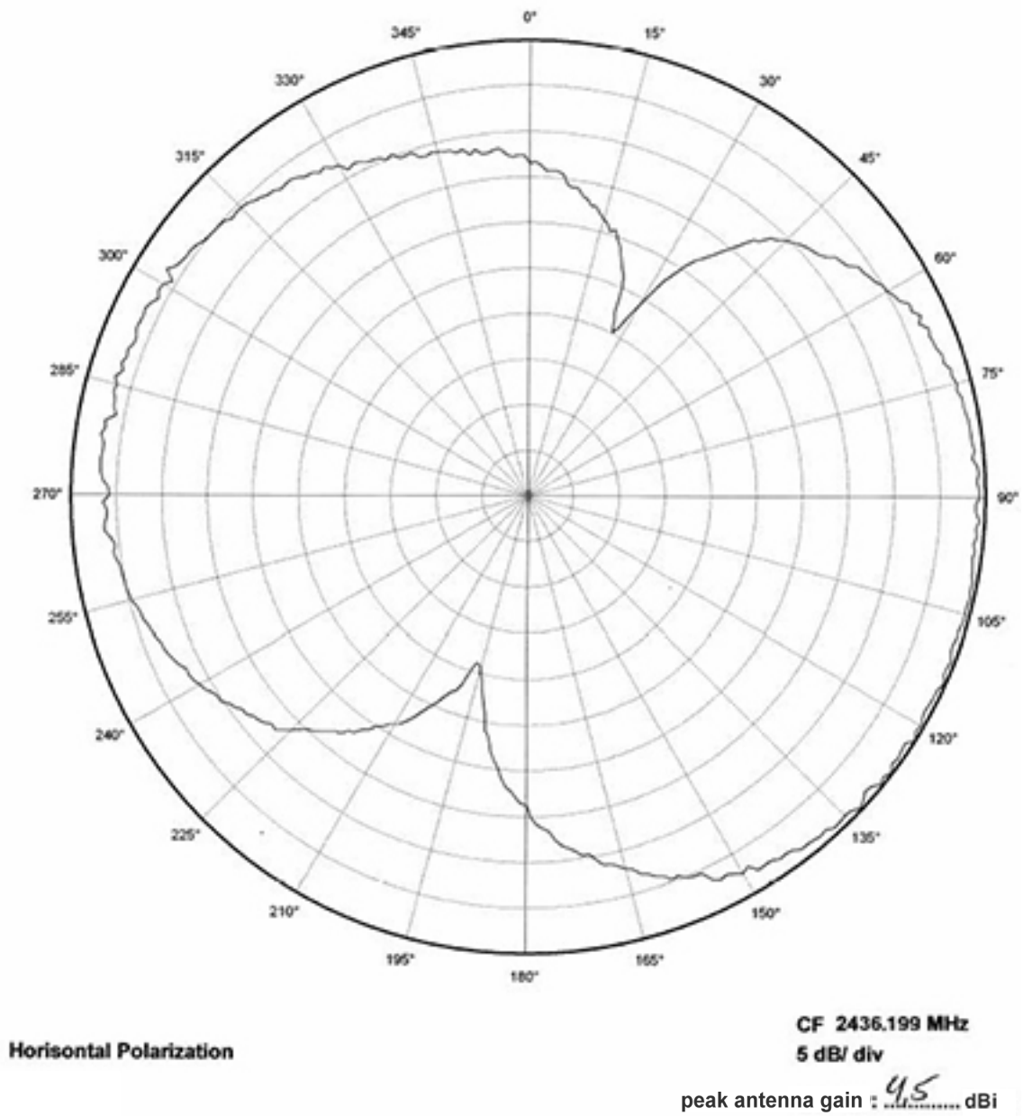
Figure 8: XY Plane
