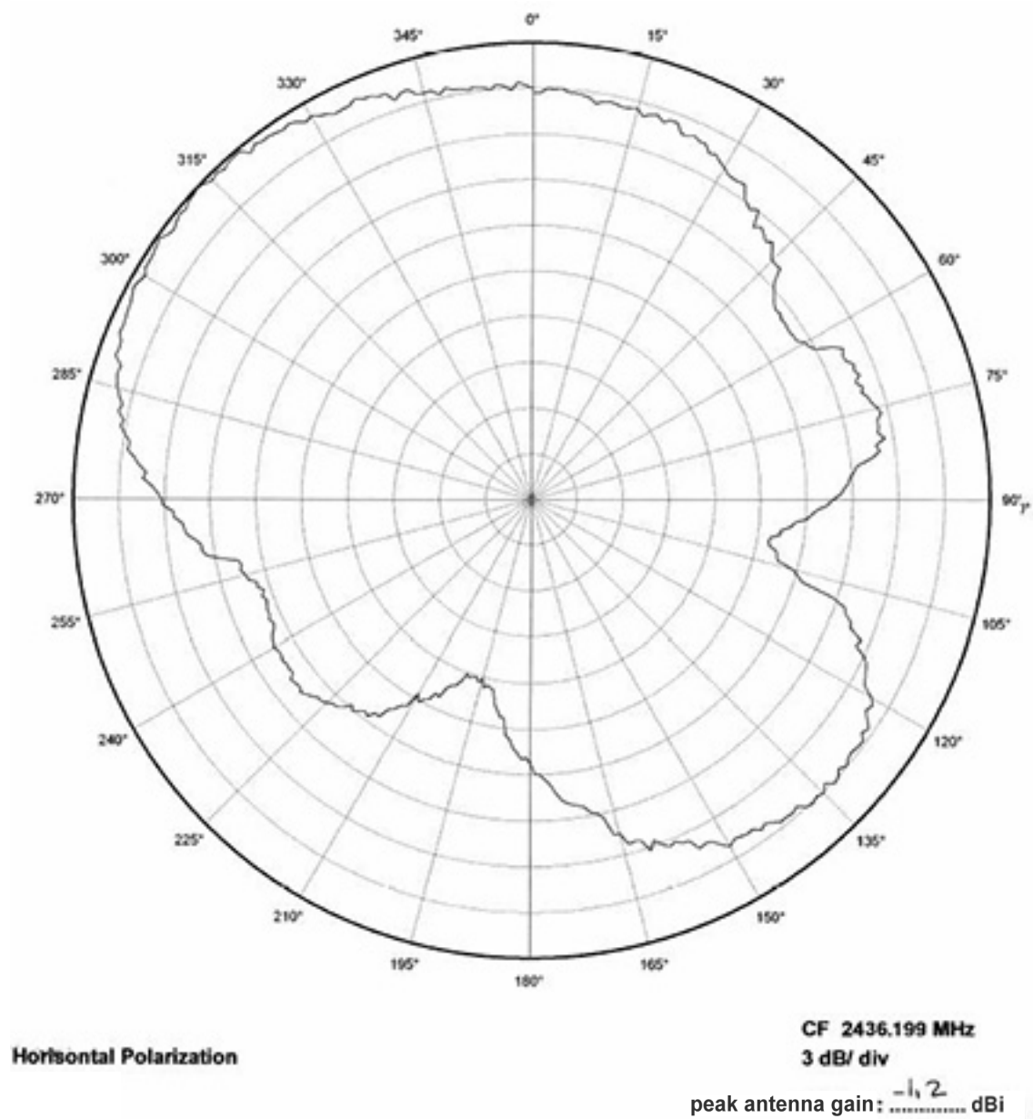
Figure 12:YZ Plane
