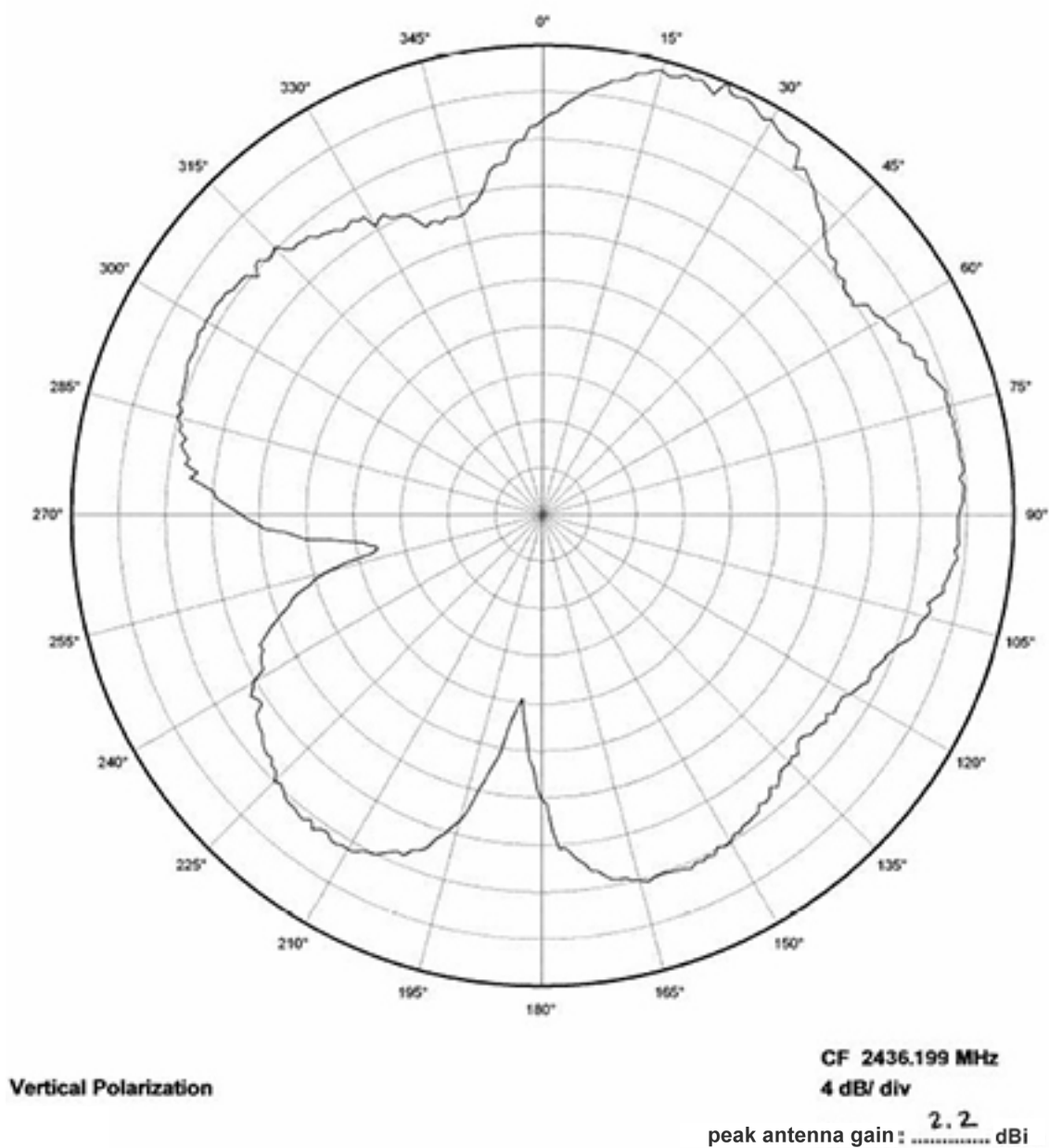
Figure 9: XZ Plane
