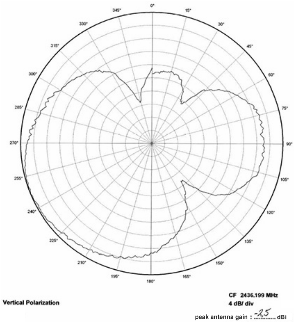
Figure 7: XY Plane
