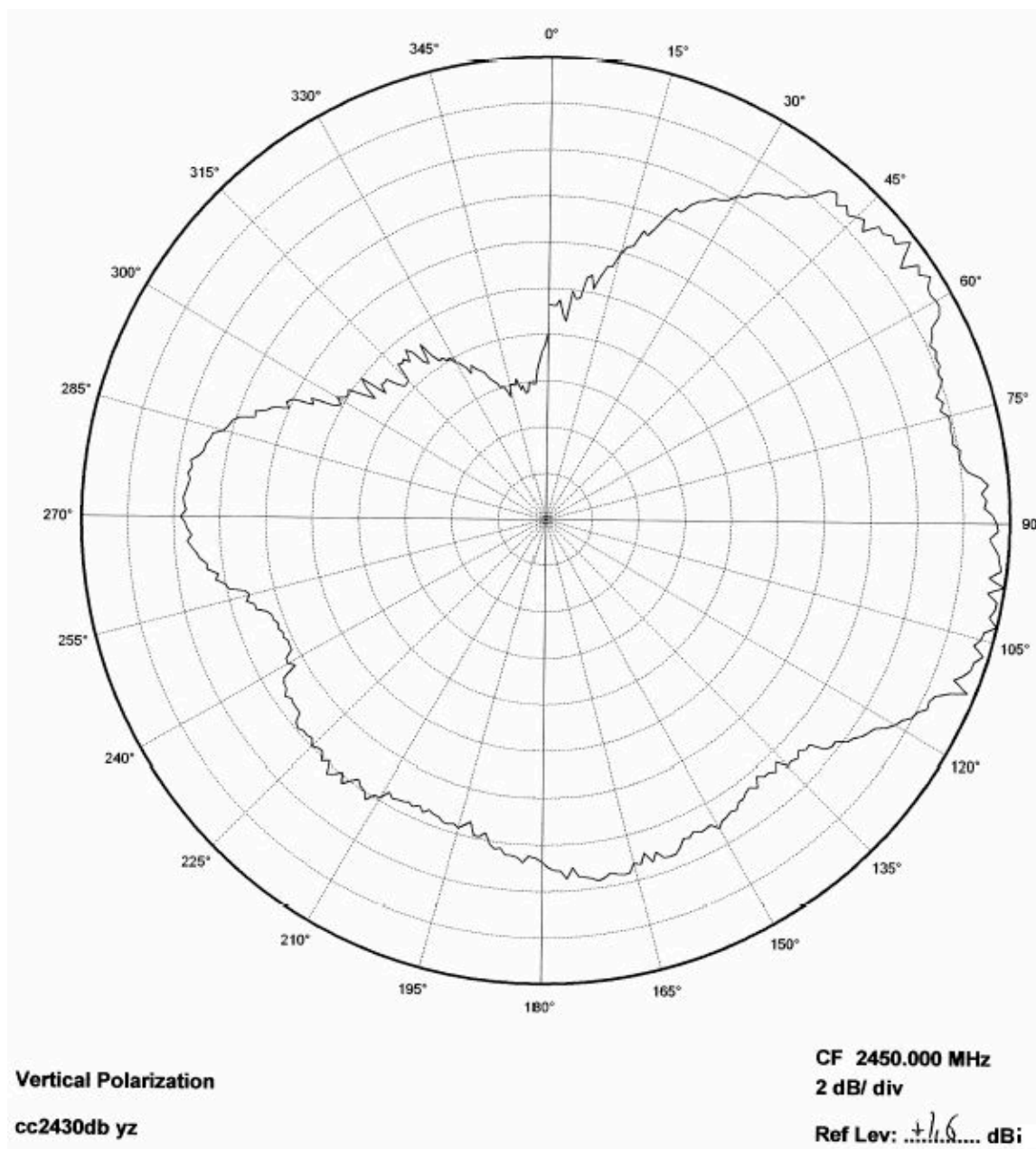
Figure 2-6. YZ Plane–Vertical Polarization
