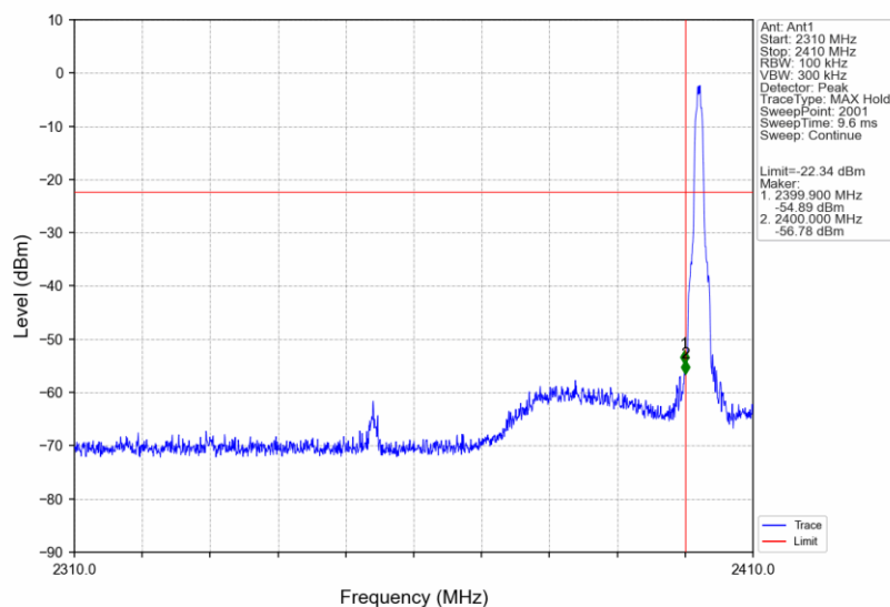
Pi/4DQPSK_2DH5_LCH_2402MHz_Ant1_NTNV
