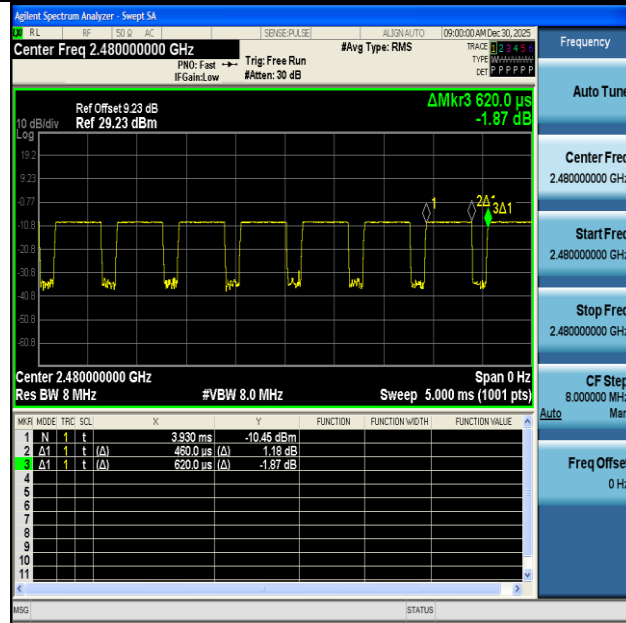
NTNV-BLE_1M-Ant1-2480
