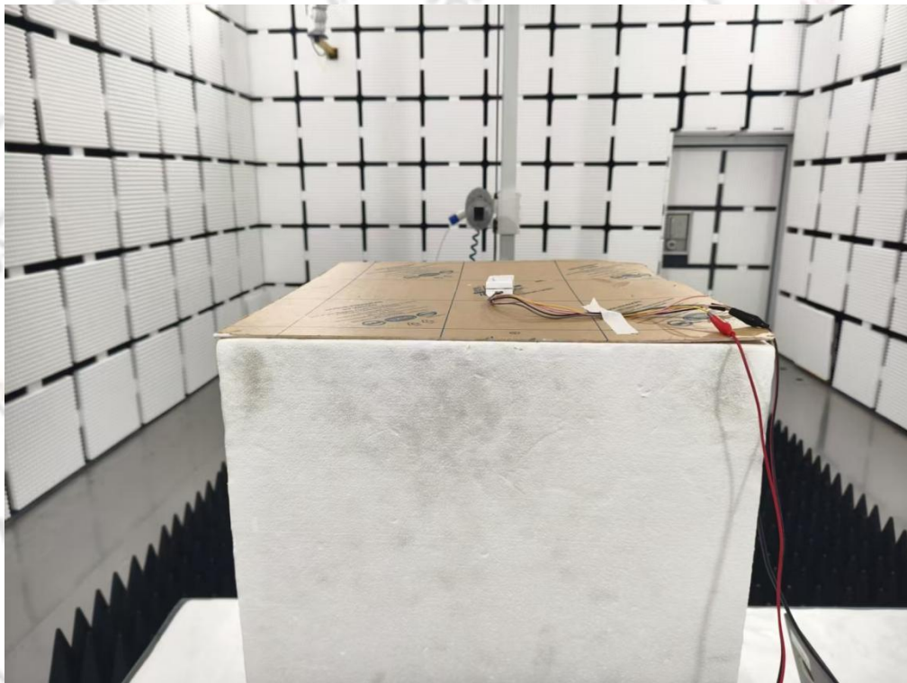
Radiated Emissions for 18GHz~40GHz
