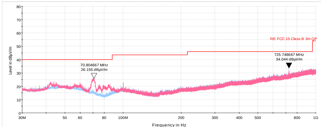
Plot 7.4.3 Unwanted emission test results at low carrier frequency in 30 – 1000 MHz range
