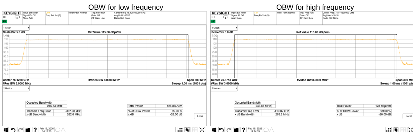
Plot 7.2.1 Occupied bandwidth measurements in normal conditions
