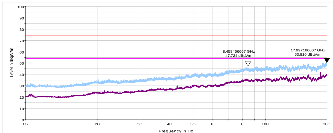
Plot 7.4.6 Unwanted emission test results at high carrier frequency in 1.0 – 18 GHz range
