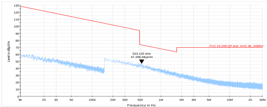
Plot 7.4.2 Unwanted emission test results at high carrier frequency in 0.009 – 30 MHz range
