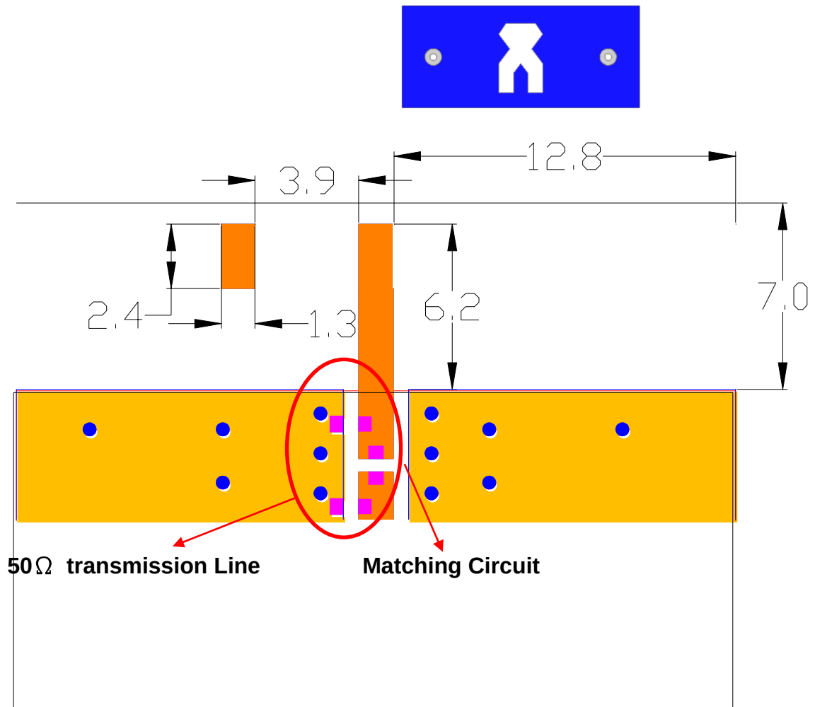
FootPrint (Unit : mm)
