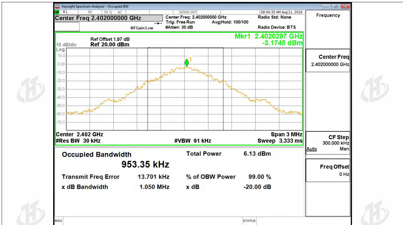
OBW NVNT 1-DH5 2402MHz Ant1
