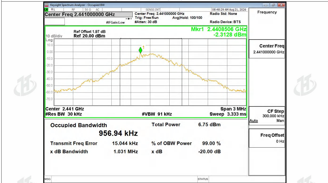
OBW NVNT 1-DH5 2441MHz Ant1
