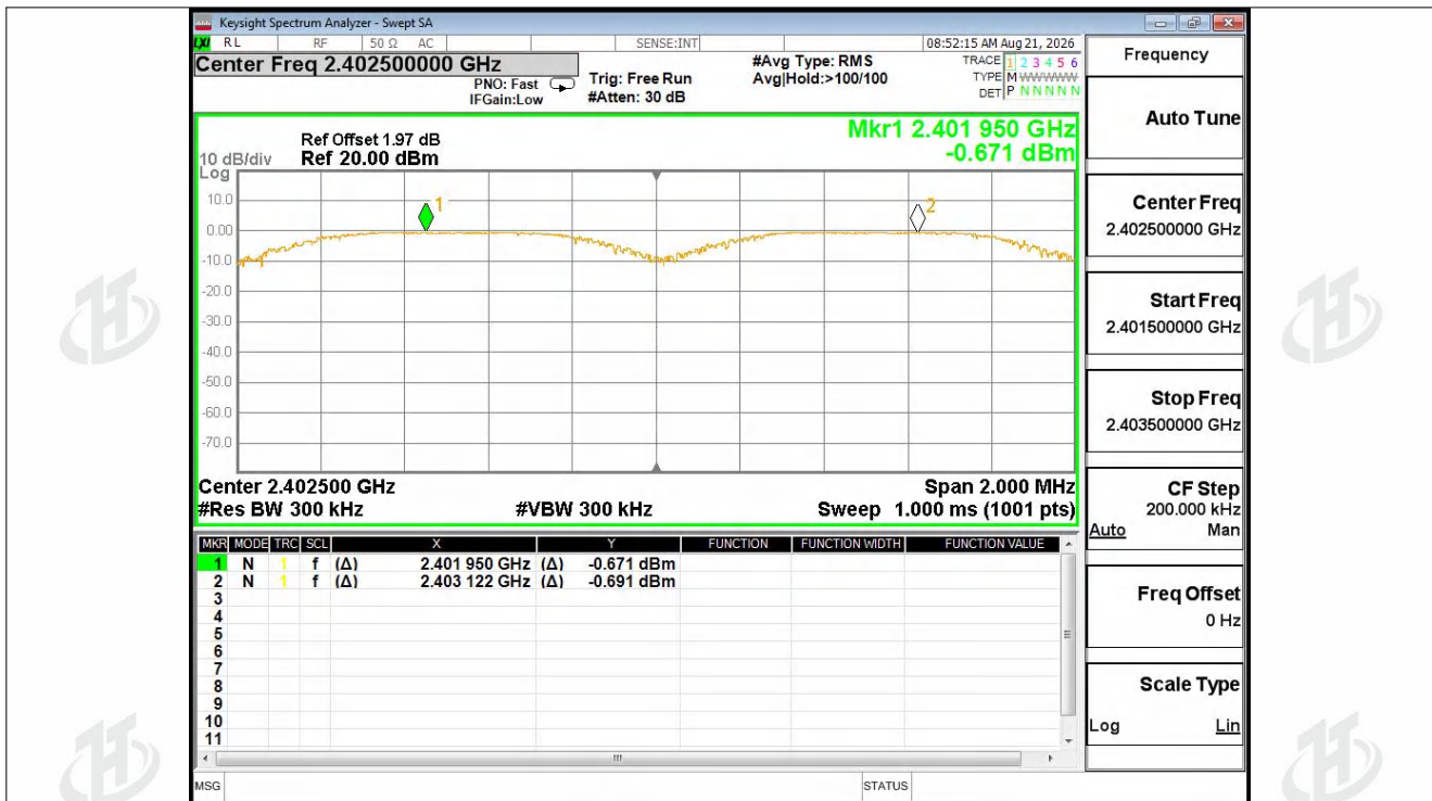
CFS NVNT 1-DH5 2402MHz Ant1
