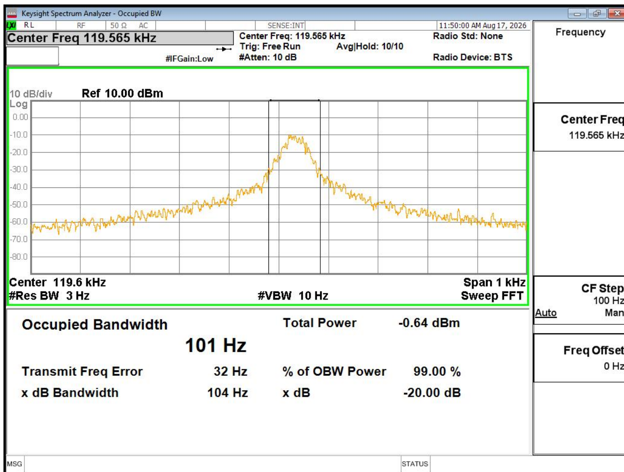
Phone coil
