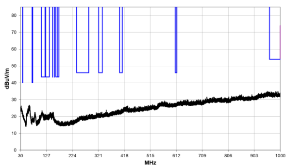
30 MHz – 1 GHz
