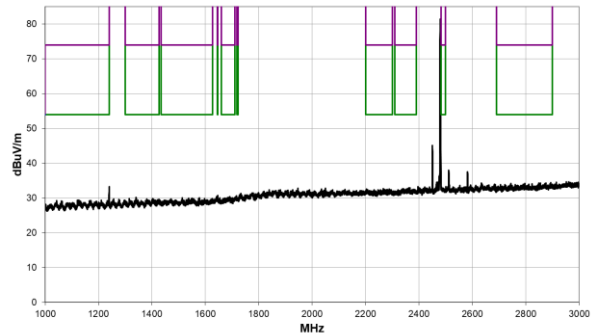
1 GHz – 3 GHz
