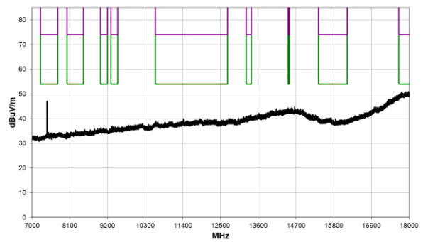
7 GHz – 18 GHz
