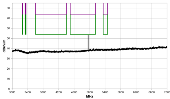
3 GHz – 7 GHz
