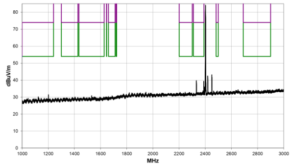
1 GHz – 3 GHz
