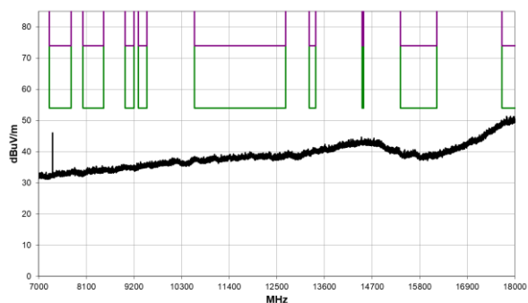
7 GHz – 18 GHz
