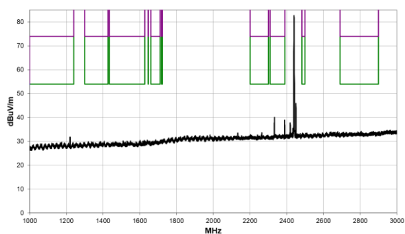
1 GHz – 3 GHz
