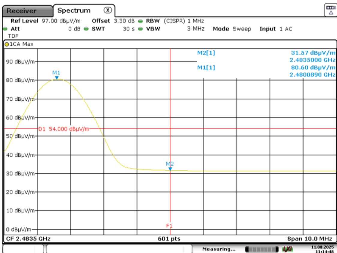
Upper Radiated Band edge Compliance – Average (with Duty cycle correction)
