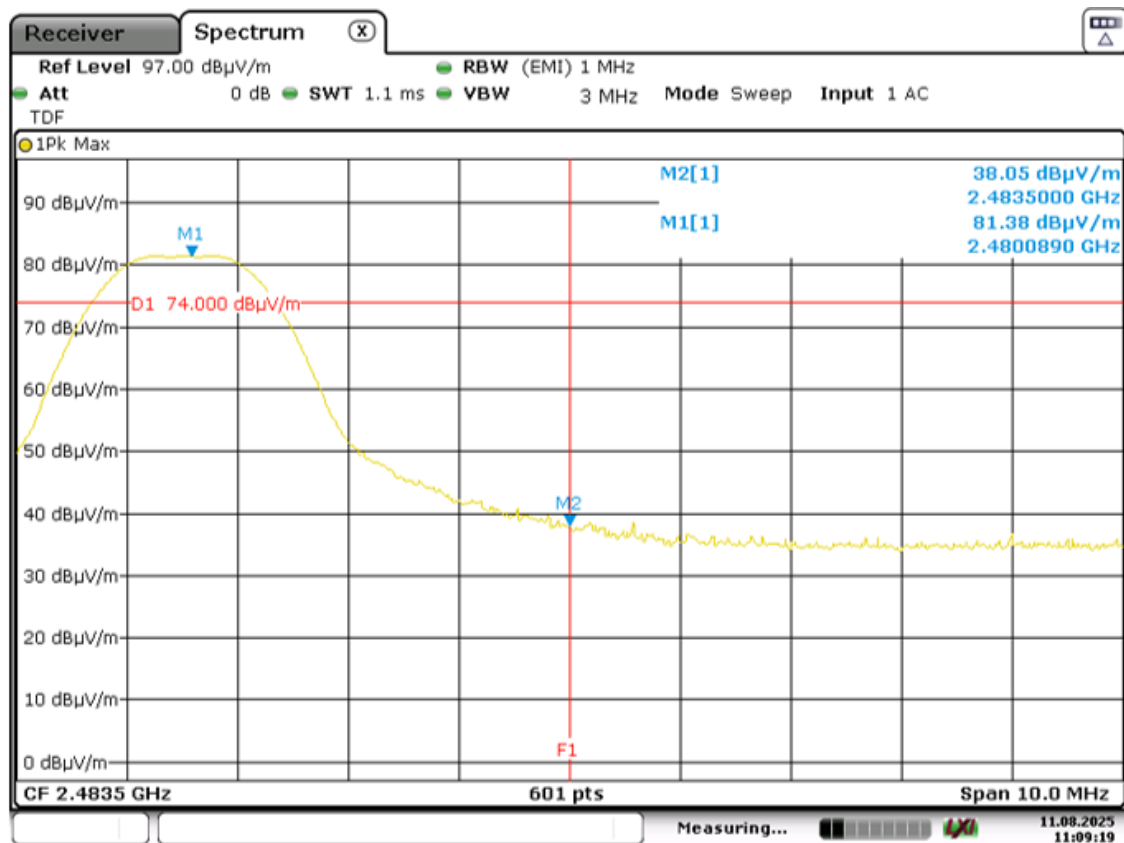
Upper Radiated Band edge Compliance – Peak
