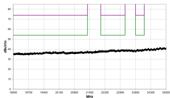
18 GHz – 25 GHz
