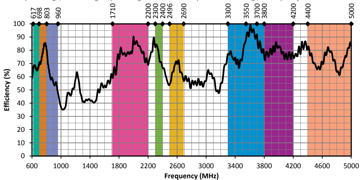
Figure 8. ANT-5GW-IPW1-NP Antenna Efficiency, Free Space
