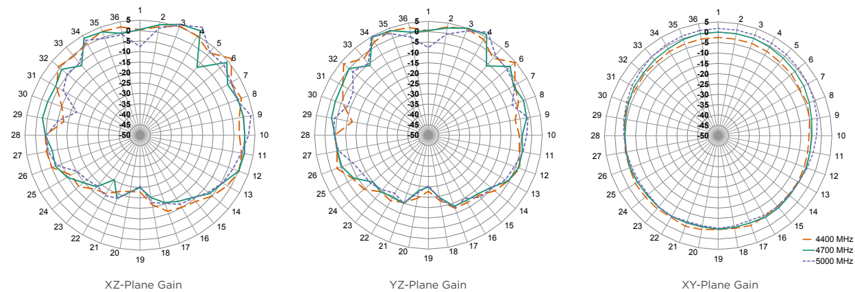
Figure 16. Radiation Patterns for ANT-5GW-IPW1-NP, Center of Ground Plane
