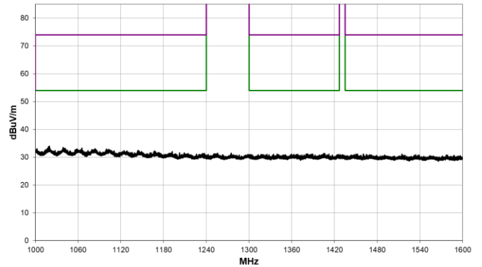
1 GHz – 1.6 GHz
