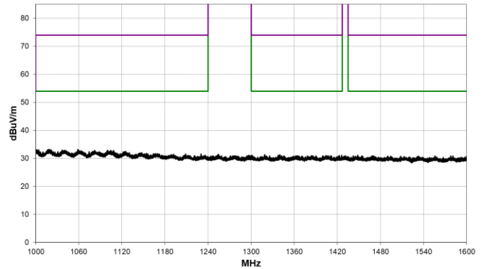
1 GHz – 1.6 GHz
