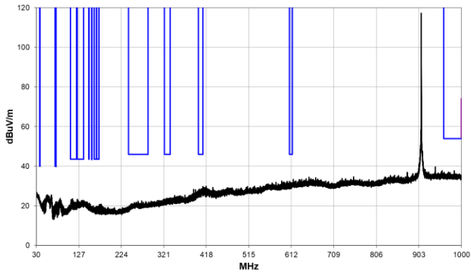
30 MHz – 1 GHz
