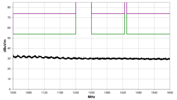
1 GHz – 1.6 GHz
