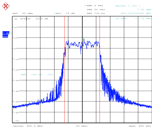
902.3 MHz
