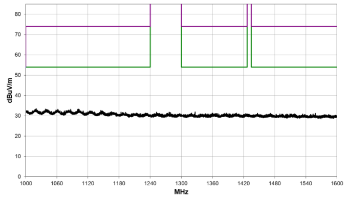
1 GHz – 1.6 GHz
