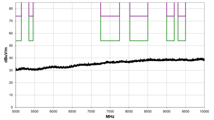
5 GHz – 10 GHz
