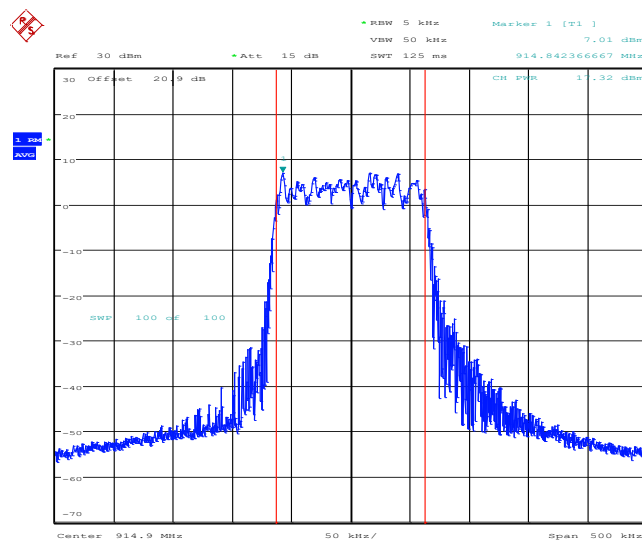
914.9 MHz
