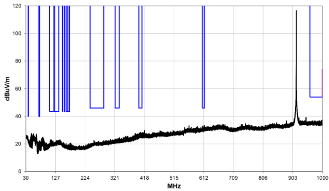
30 MHz – 1 GHz
