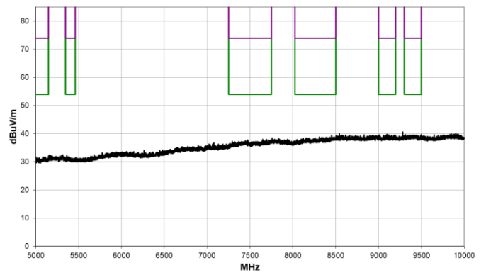
5 GHz – 10 GHz
