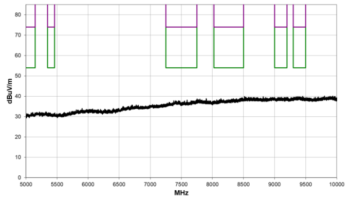
5 GHz – 10 GHz
