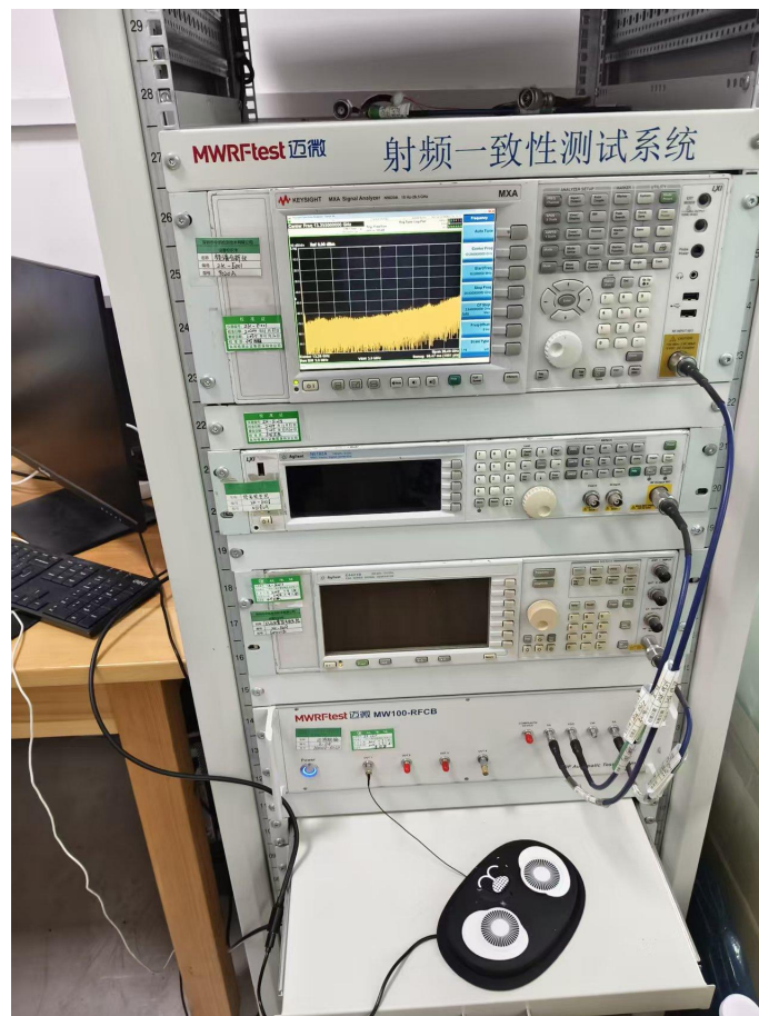
RF Conduction
