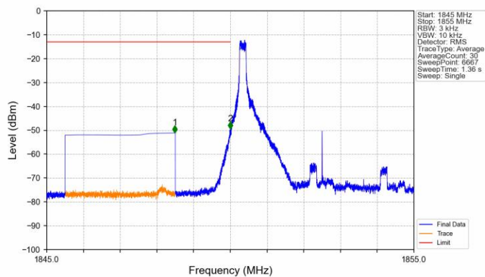
Band2_5MHz_QPSK_LCH_1852.5MHz_RB_1_0_NTNV
