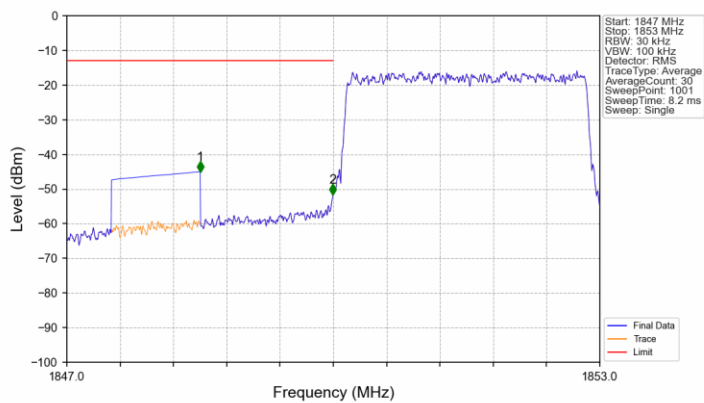
Band2_3MHz_16QAM_LCH_1851.5MHz_RB_15_0_NTNV
