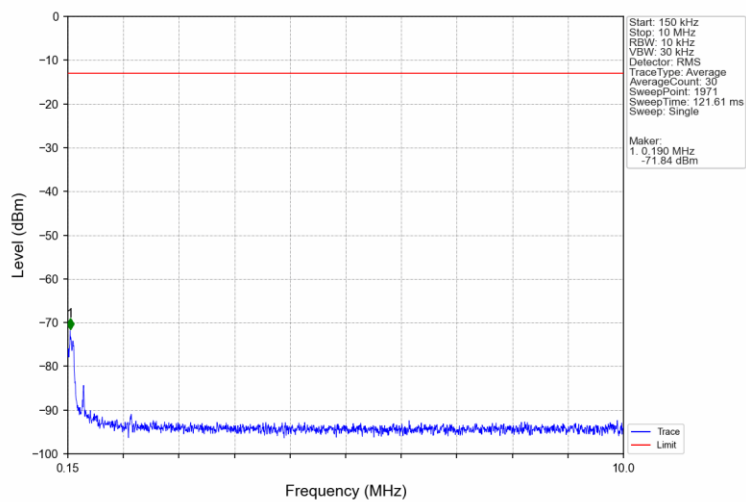
Band4_3MHz_QPSK_LCH_1711.5MHz_RB_1_0_NTNV
