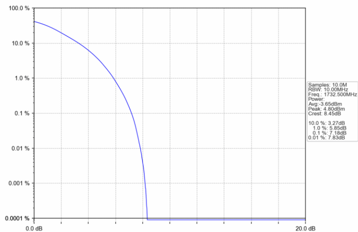
Band4_20MHz_16QAM_MCH_1732.5MHz_RB_27_0_NTNV
