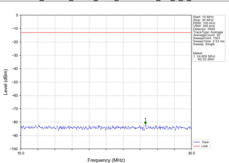
Band4_1.4MHz_QPSK_MCH_1732.5MHz_RB_1_0_NTNV
