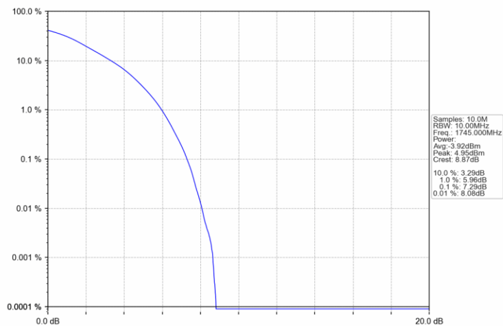
Band4_20MHz_16QAM_HCH_1745MHz_RB_27_73_NTNV
