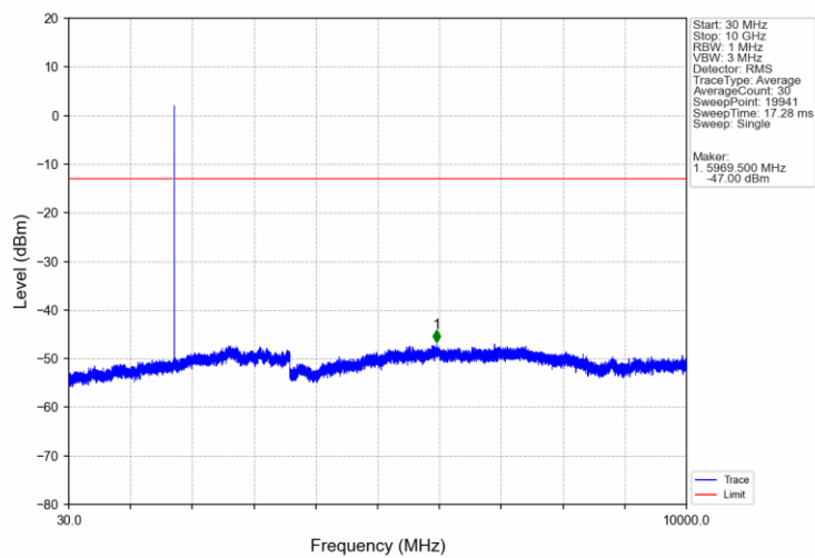
Band4_1.4MHz_QPSK_MCH_1732.5MHz_RB_1_0_NTNV
