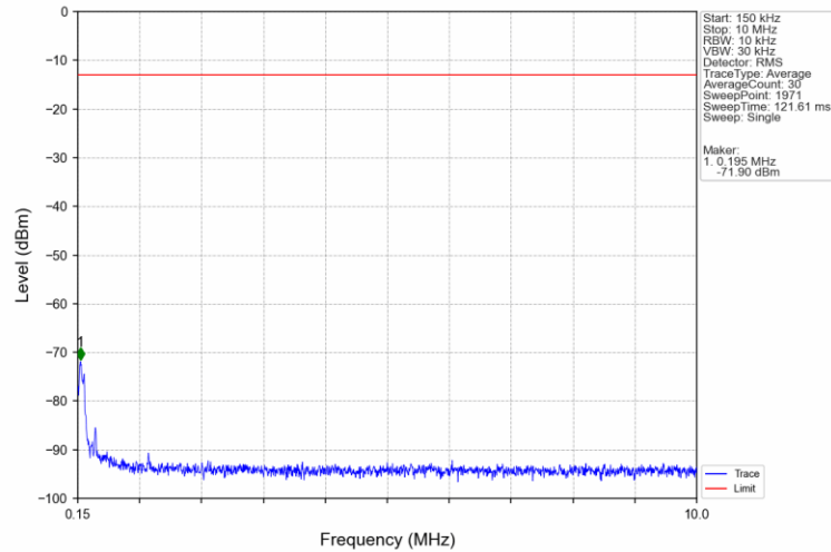
Band4_1.4MHz_16QAM_MCH_1732.5MHz_RB_1_0_NTNV
