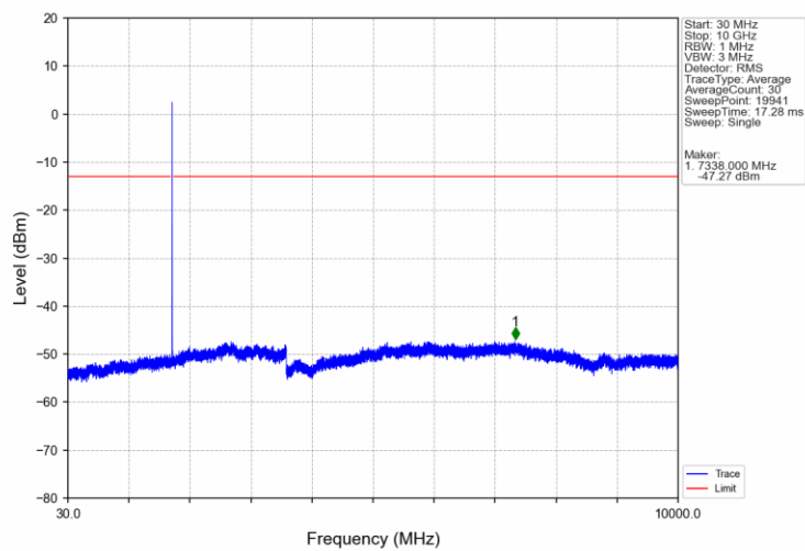
Band4_3MHz_QPSK_MCH_1732.5MHz_RB_1_0_NTNV
