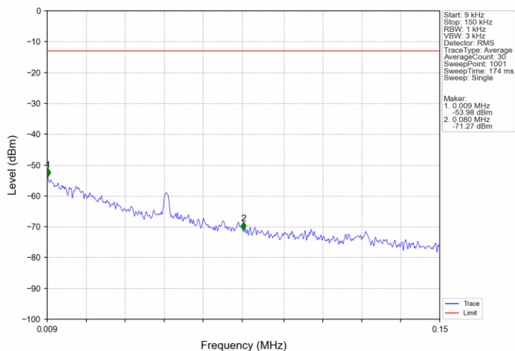
Band4_3MHz_QPSK_LCH_1711.5MHz_RB_1_0_NTNV
