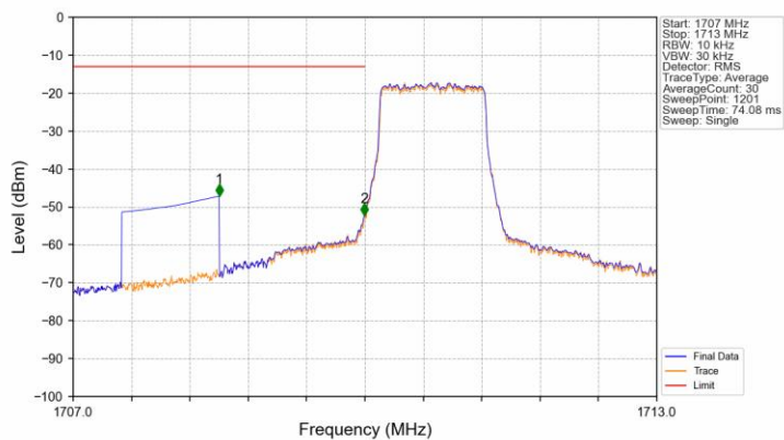
Band4_1.4MHz_16QAM_LCH_1710.7MHz_RB_6_0_NTNV
