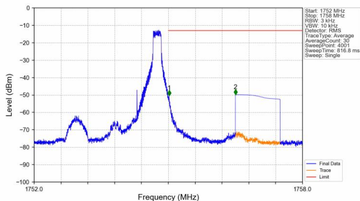
Band4_1.4MHz_QPSK_HCH_1754.3MHz_RB_1_5_NTNV
