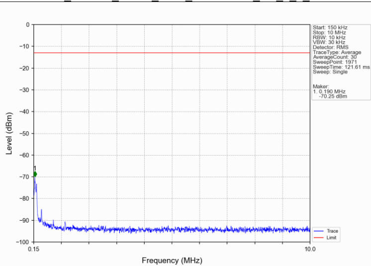
Band4_1.4MHz_QPSK_MCH_1732.5MHz_RB_1_0_NTNV
