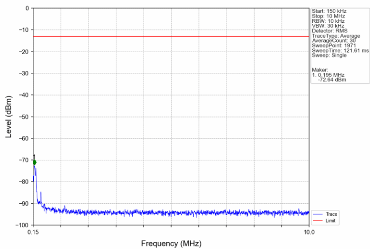
Band4_5MHz_QPSK_MCH_1732.5MHz_RB_1_0_NTNV
