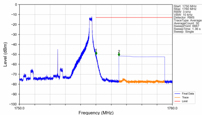
Band4_5MHz_QPSK_HCH_1752.5MHz_RB_1_24_NTNV
