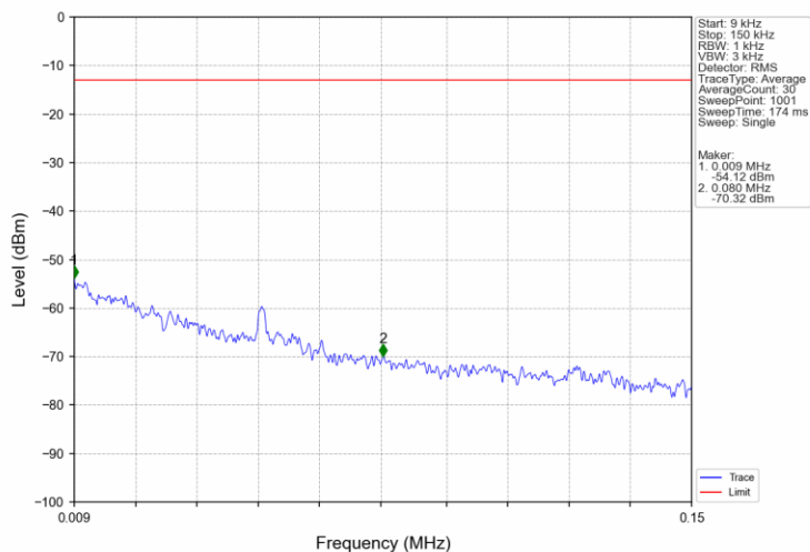
Band4_5MHz_QPSK_LCH_1712.5MHz_RB_1_0_NTNV
