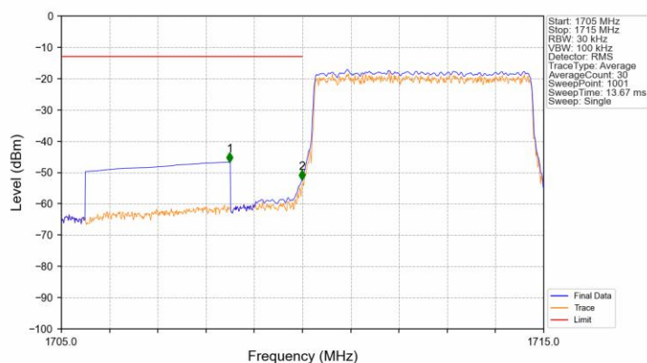
Band4_5MHz_16QAM_LCH_1712.5MHz_RB_25_0_NTNV
