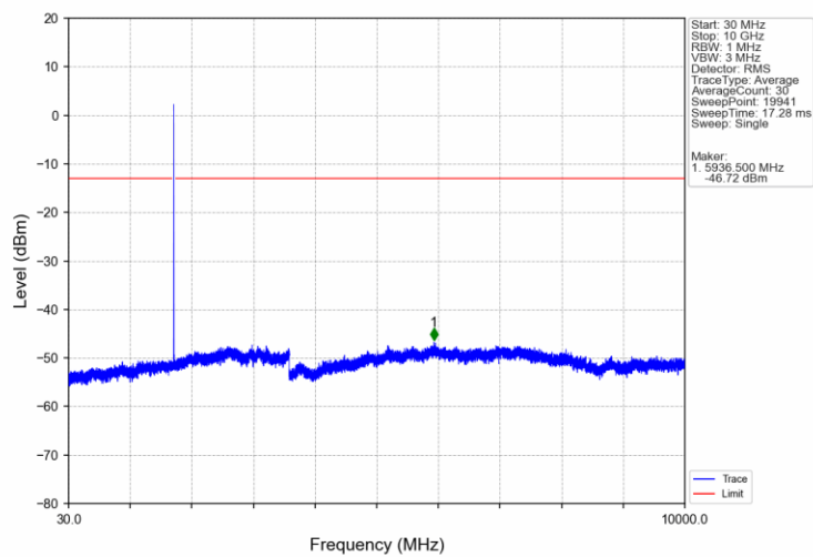
Band4_5MHz_QPSK_MCH_1732.5MHz_RB_1_0_NTNV
