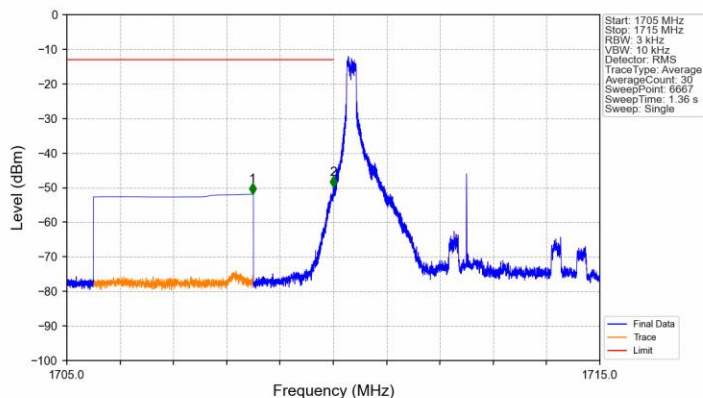
Band4_5MHz_QPSK_LCH_1712.5MHz_RB_1_0_NTNV
