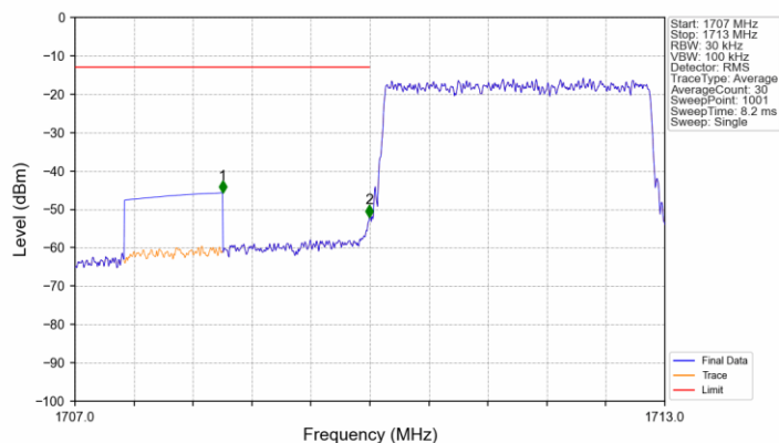
Band4_3MHz_16QAM_LCH_1711.5MHz_RB_15_0_NTNV
