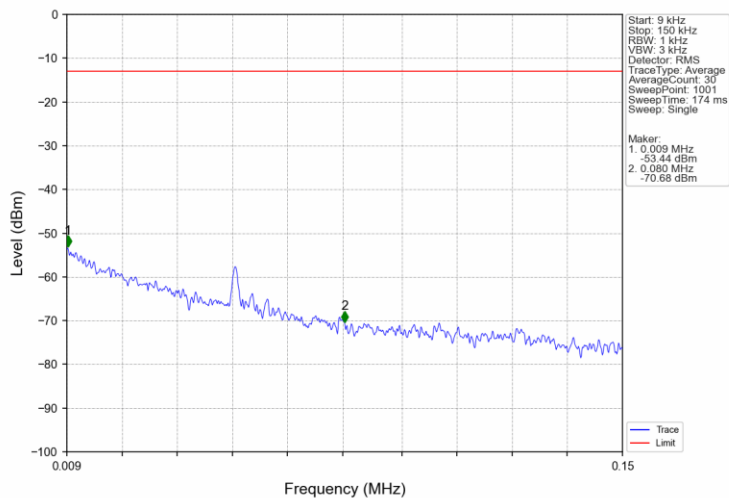
Band4_5MHz_16QAM_HCH_1752.5MHz_RB_1_0_NTNV
