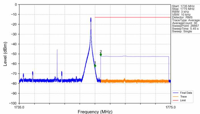
Band4_20MHz_16QAM_HCH_1745MHz_RB_1_99_NTNV
