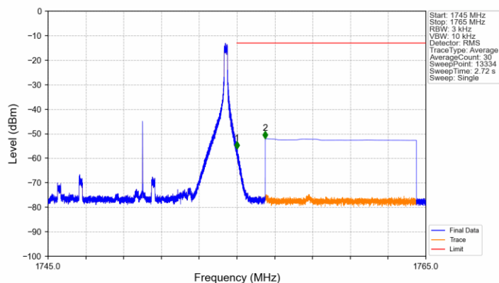
Band4_10MHz_16QAM_HCH_1750MHz_RB_1_49_NTNV
