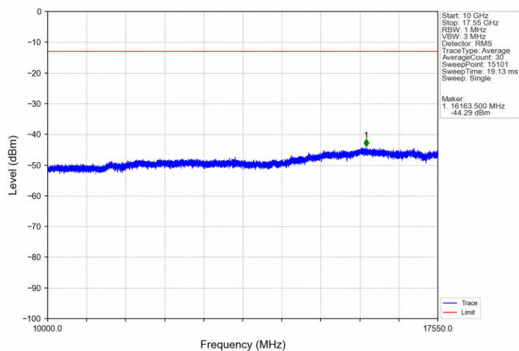
Band4_20MHz_16QAM_HCH_1745MHz_RB_1_99_NTNV
