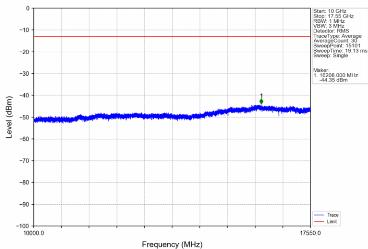
Band4_15MHz_16QAM_HCH_1747.5MHz_RB_1_74_NTNV
