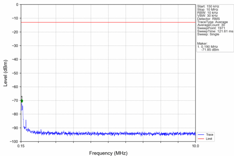
Band4_15MHz_QPSK_HCH_1747.5MHz_RB_1_0_NTNV
