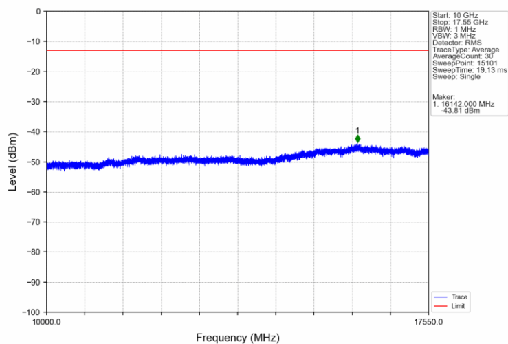
Band4_10MHz_16QAM_HCH_1750MHz_RB_1_49_NTNV
