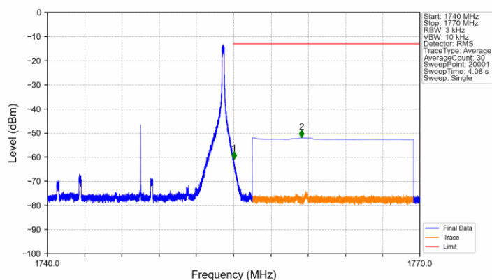
Band4_15MHz_16QAM_HCH_1747.5MHz_RB_1_74_NTNV
