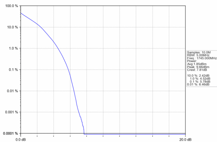
Band66_5MHz_QPSK_MCH_1745MHz_RB_25_0_NTNV
