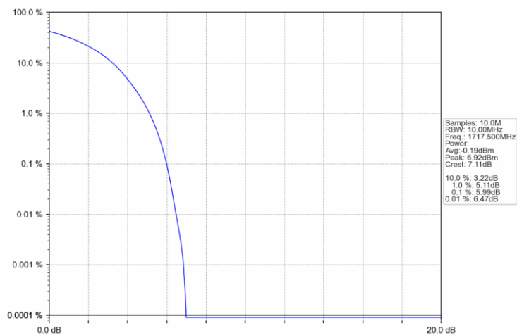
Band66_15MHz_16QAM_LCH_1717.5MHz_RB_27_0_NTNV
