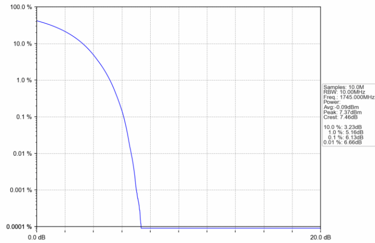
Band66_15MHz_16QAM_MCH_1745MHz_RB_27_0_NTNV
