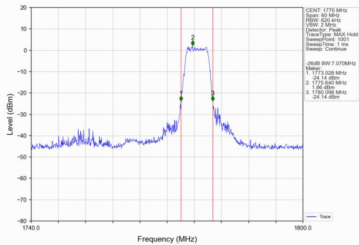
Band66_20MHz_16QAM_HCH_1770MHz_RB_27_73_NTNV
