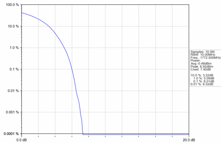
Band66_15MHz_16QAM_HCH_1772.5MHz_RB_27_48_NTNV
