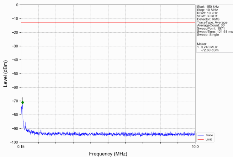
Band66_1.4MHz_QPSK_HCH_1779.3MHz_RB_1_0_NTNV
