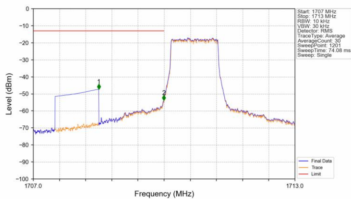
Band66_1.4MHz_16QAM_LCH_1710.7MHz_RB_6_0_NTNV
