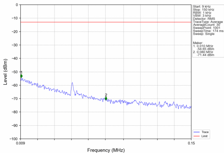
Band66_1.4MHz_QPSK_HCH_1779.3MHz_RB_1_0_NTNV
