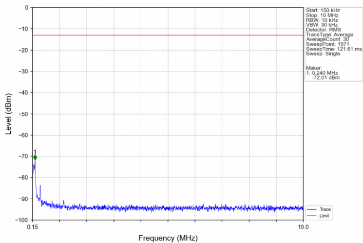
Band66_1.4MHz_16QAM_LCH_1710.7MHz_RB_1_0_NTNV
