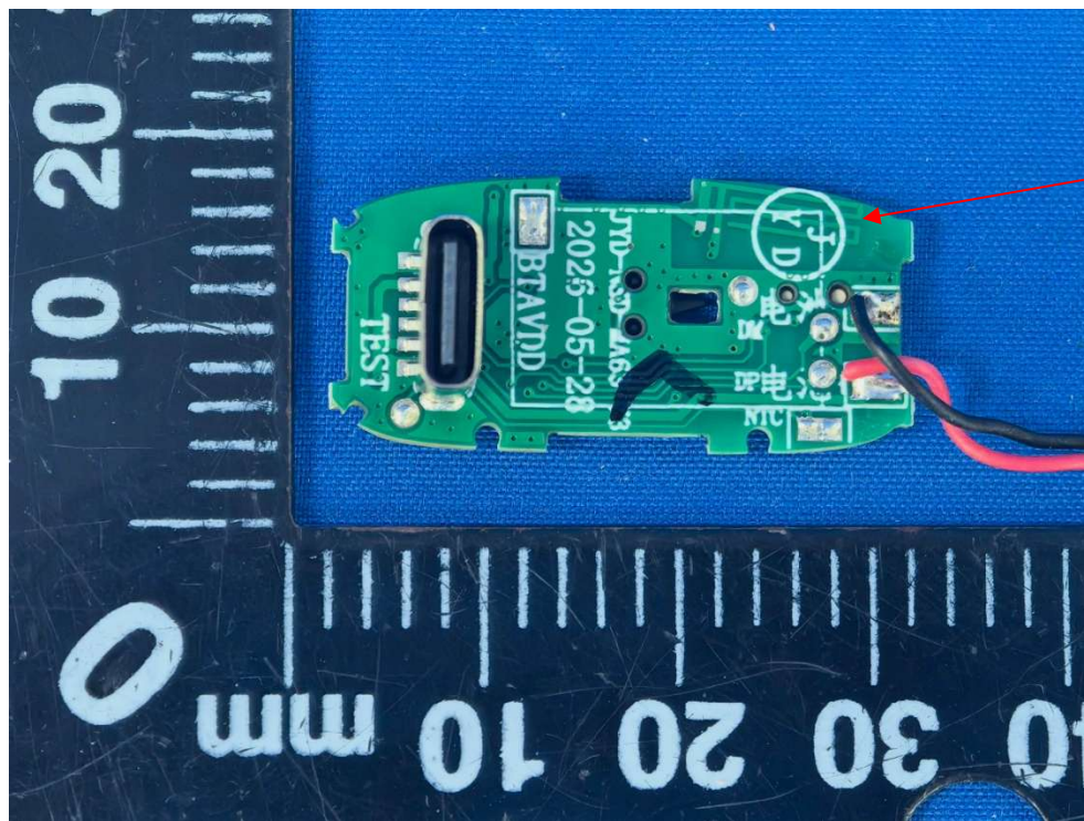
Bluetooth Antenna
