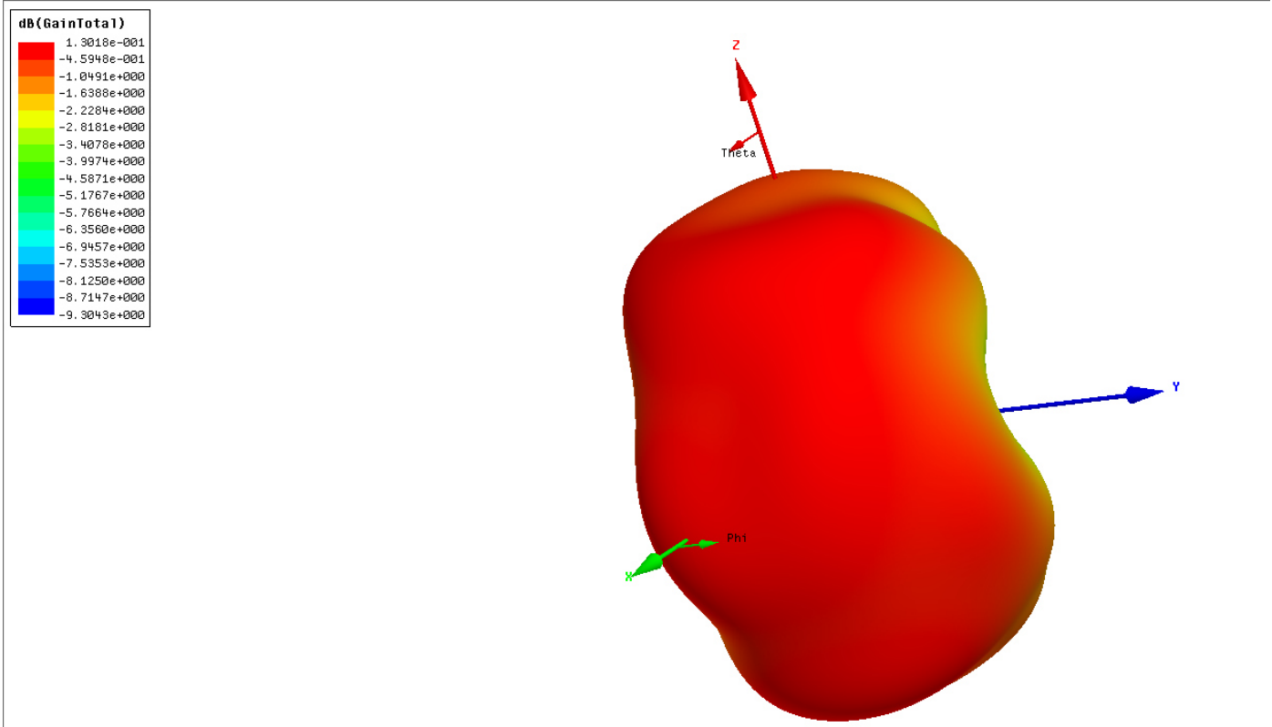
2.402G 3D Directional Chart
