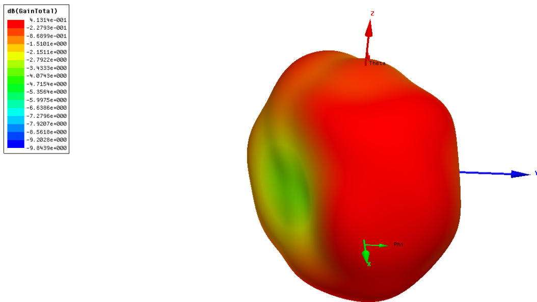
2.440G 3D Directional Chart
