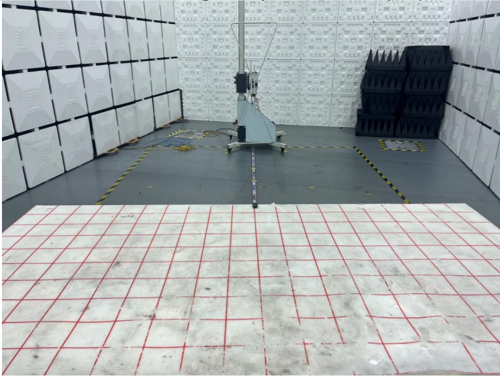
Radiated Band edge and Spurious Emission (BLE)
