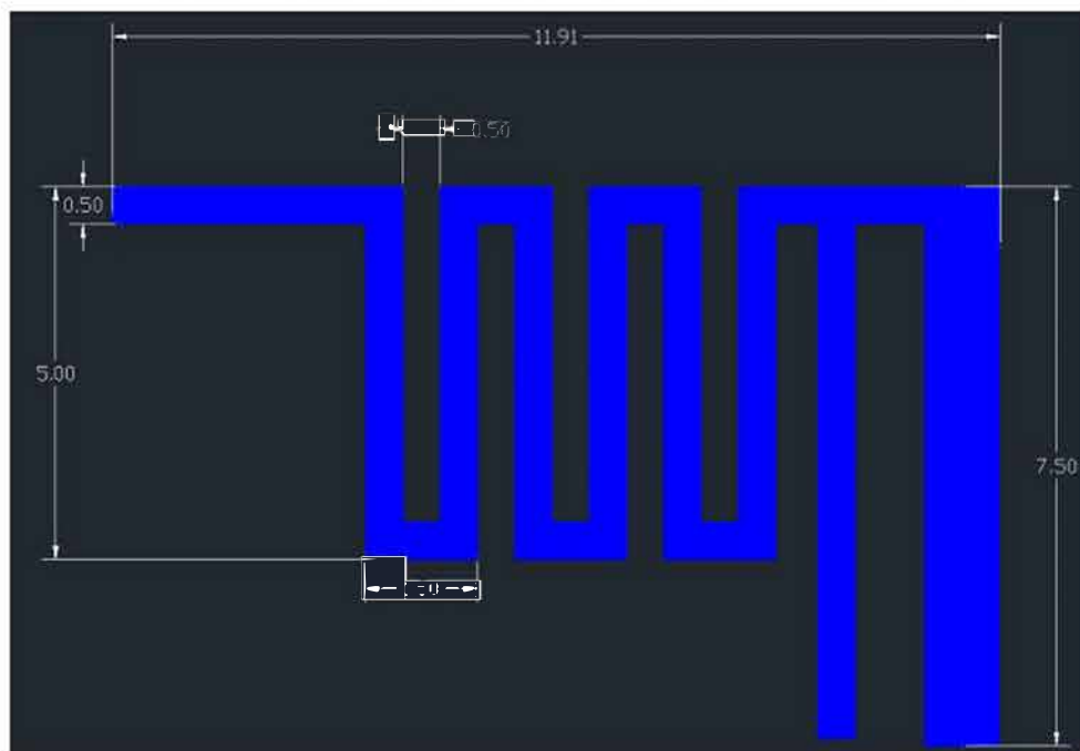
Physical object and physical size of the antenna (unit:mm)
