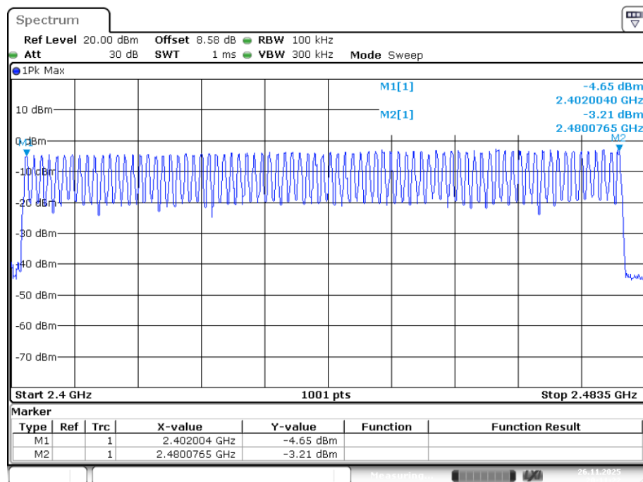
Hopping No. NVNT GFSK 2441MHz Ant1
