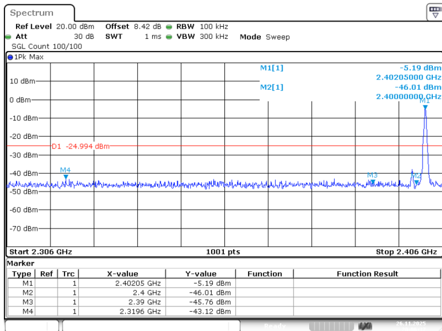
Band Edge NVNT GFSK 2402MHz Ant1 No-Hopping Emission
