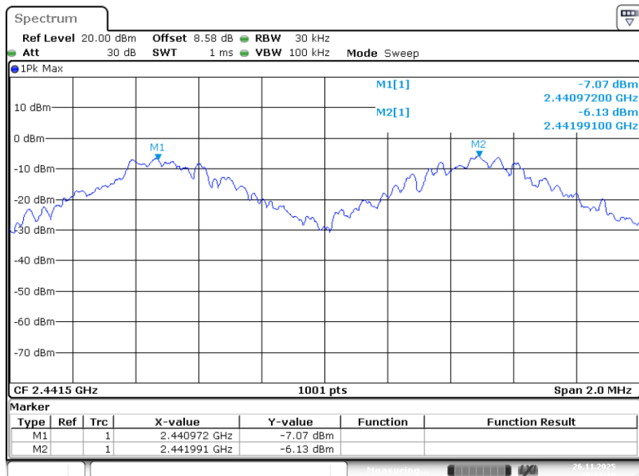
CFS NVNT GFSK 2441MHz Ant1
