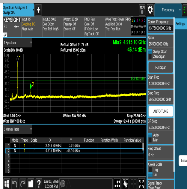
11N40SISO-Ant1-2452-1000~26500-PASS
