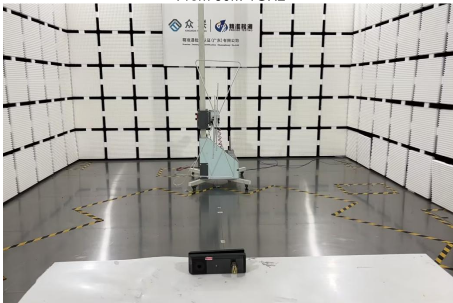
Radiated Emissions From 30M-1GHz
