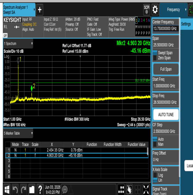
11AX40SISO-Ant1-2452-1000~26500-PASS
