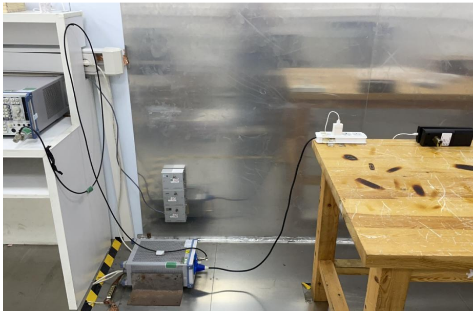
Conducted Emissions
