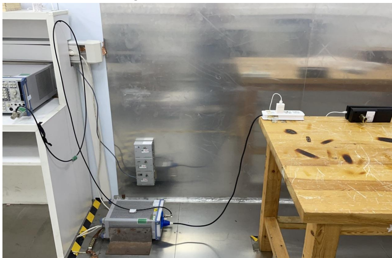
Conducted Emissions
