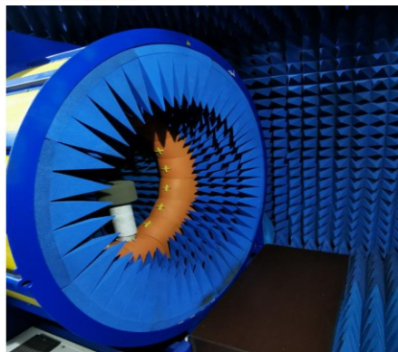
SATIMO-16
