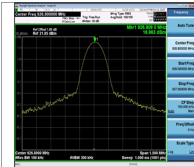
TURMASS-Ant1-926.8-0~Reference-PASS
