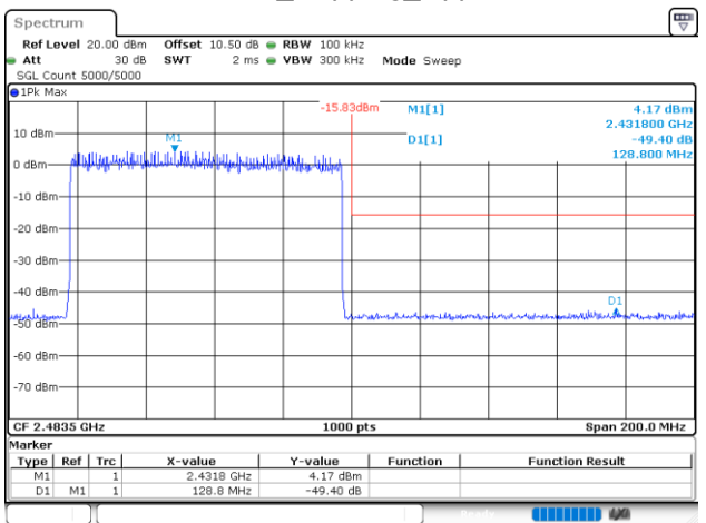
2DH5_Hopping_Upper
