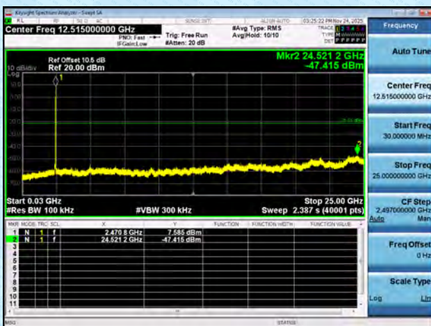
11AX20MIMO-Ant7-2462-26Tone-RU8-30~25000-PASS
