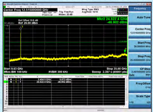
11AX20MIMO-Ant6-2412-26Tone-RU0-30~25000-PASS
