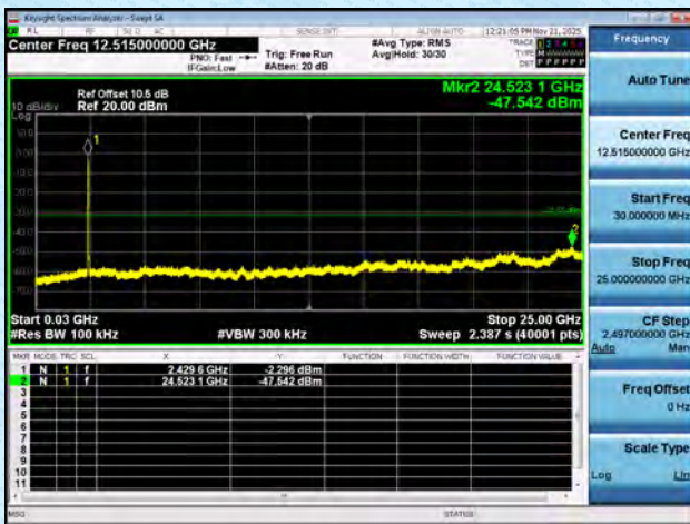
11N40MIMO-Ant7-2437-0~Reference-PASS
