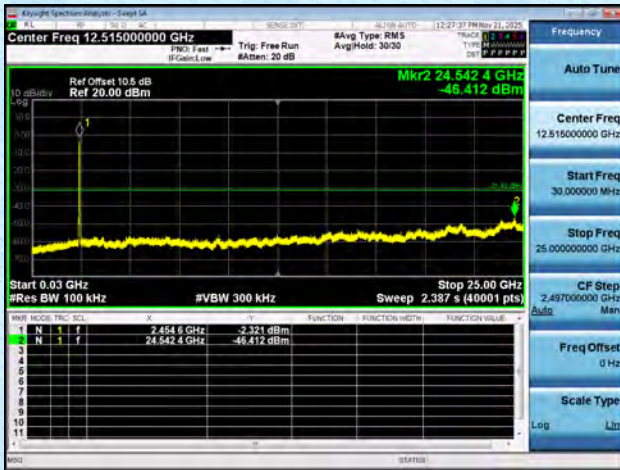
11N40MIMO-Ant7-2452-0~Reference-PASS
