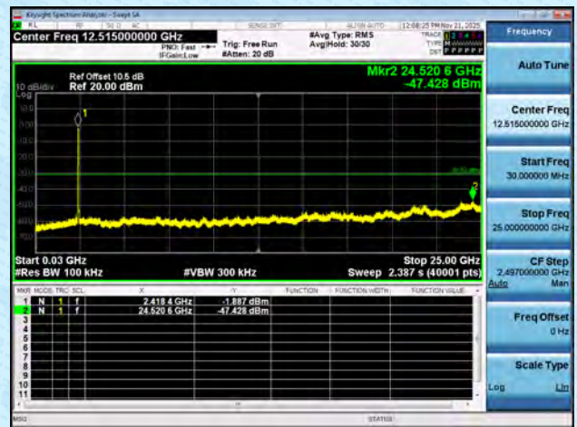
11AX40MIMO-Ant6-2437-0-Reference-PASS
