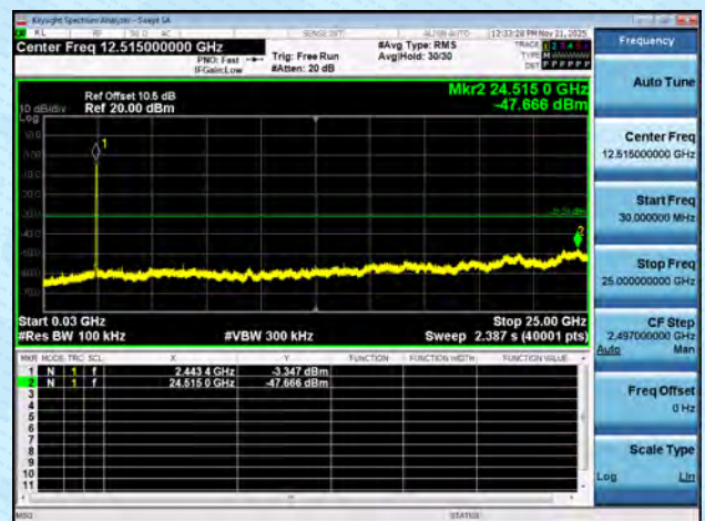
11N40MIMO-Ant6-2452-30~25000-PASS
