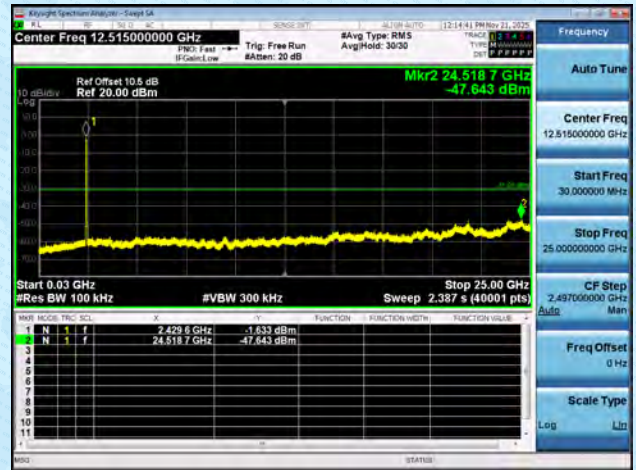
11AX40MIMO-Ant6-2452-0-Reference-PASS
