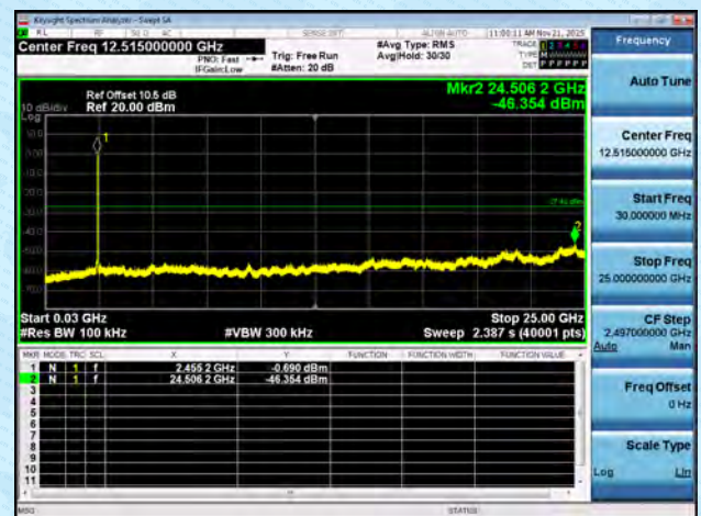
11N20MIMO-Ant6-2462-30~25000-PASS
