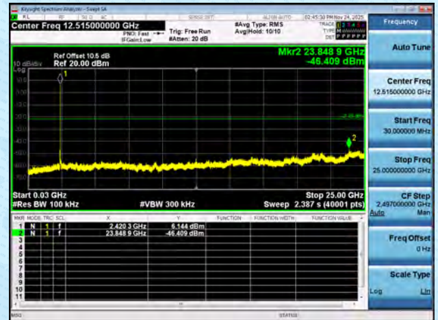
11AX20MIMO-Ant6-2437-26Tone-RU0-0~Reference-PASS
