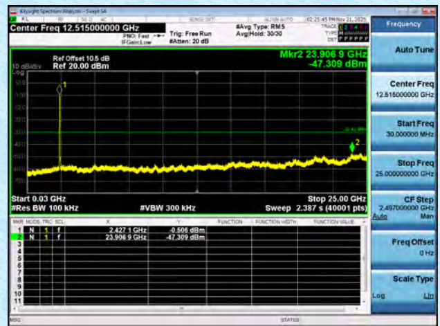
11N40MIMO-Ant6-2437-0~Reference-PASS
