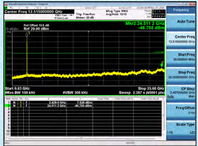
11AX20MIMO-Ant6-2437-26Tone-RU8-30~25000-PASS
