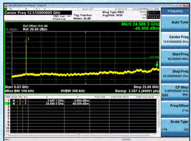
11AX40MIMO-Ant6-2452-30~25000-PASS
