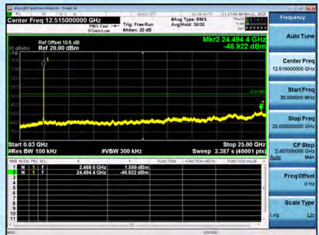
11AX20MIMO-Ant6-2462-30~25000-PASS
