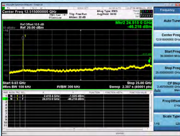
11AX40MIMO-Ant7-2437-0-Reference-PASS
