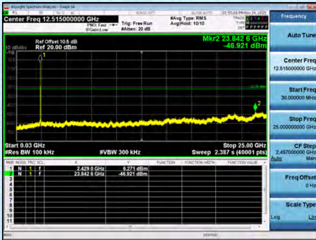
11AX20MIMO-Ant7-2437-26Tone-RU8-30~25000-PASS
