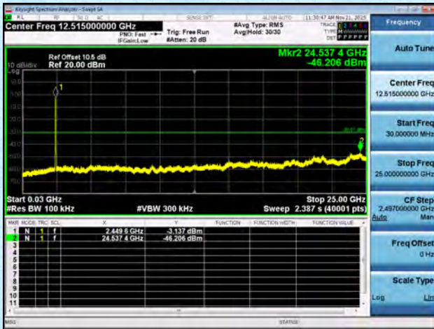
11AX40MIMO-Ant7-2452-0-Reference-PASS
