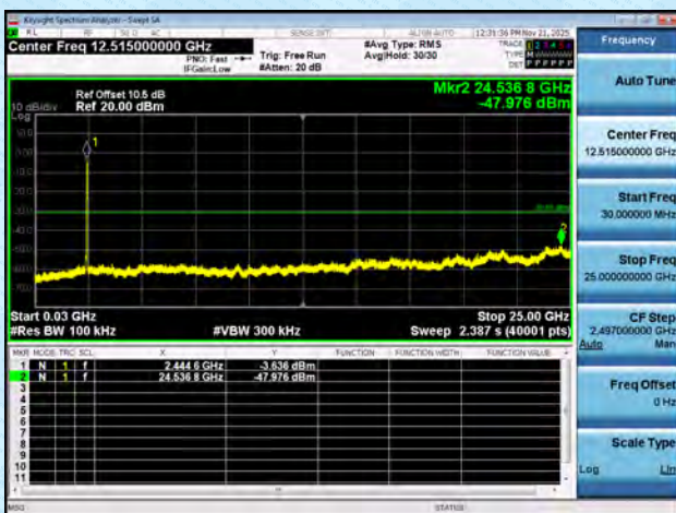
11N40MIMO-Ant7-2452-30~25000-PASS
