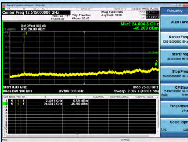
11AX20MIMO-Ant7-2412-26Tone-RU0-30~25000-PASS
