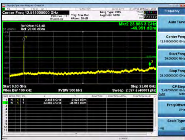
11AX40MIMO-Ant7-2452-30~25000-PASS
