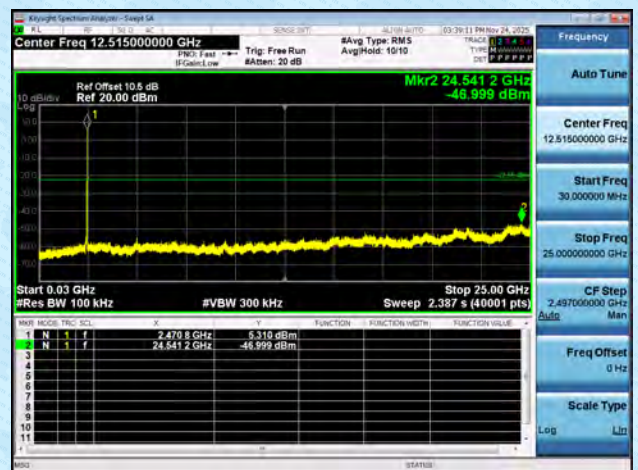
11AX20MIMO-Ant6-2462-26Tone-RU8-30~25000-PASS
