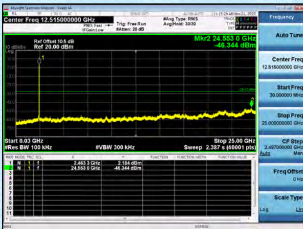
11AX20MIMO-Ant7-2462-30~25000-PASS
