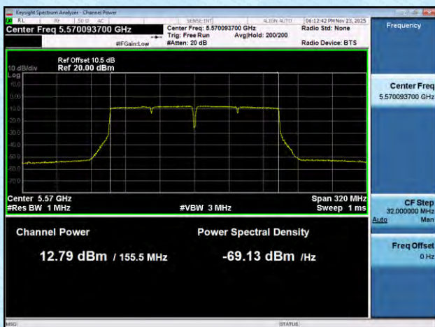
11AC160MIMO-Ant6-5570-PASS
