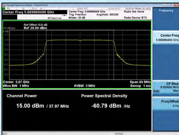
11AX40SISO-Ant6-5670-PASS
