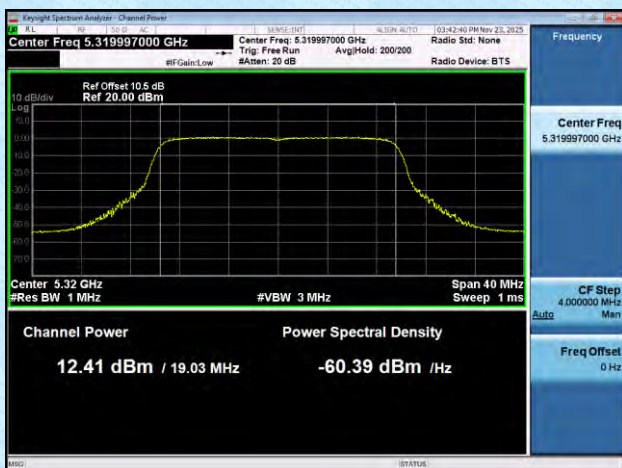
11AX20MIMO-Ant6-5320-PASS
