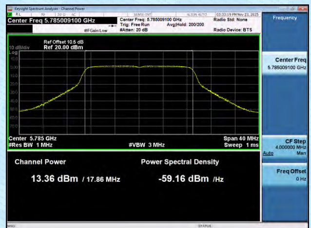
11AC20MIMO-Ant8-5785-PASS
