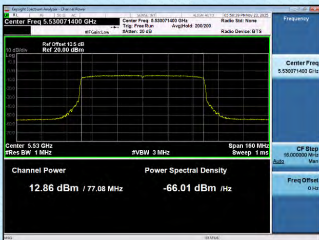
11AX80MIMO-Ant6-5530-PASS
