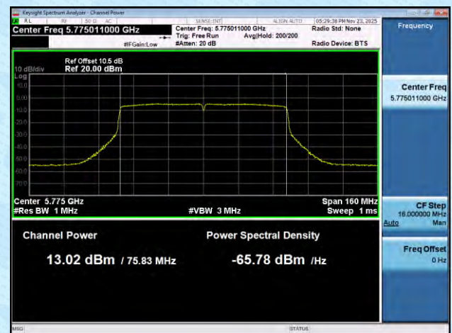
11AC80MIMO-Ant8-5775-PASS
