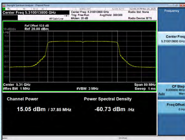
11AX40SISO-Ant6-5310-PASS
