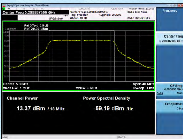
11N20MIMO-Ant6-5300-PASS
