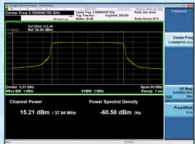
11AX40SISO-Ant8-5310-PASS
