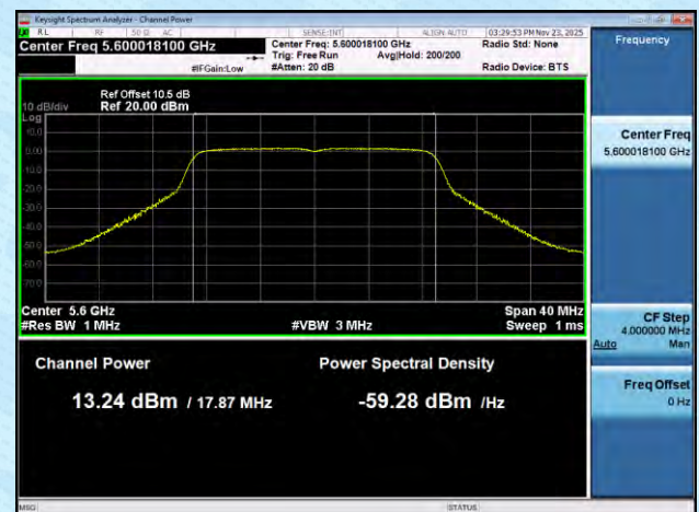
11AC20MIMO-Ant8-5600-PASS
