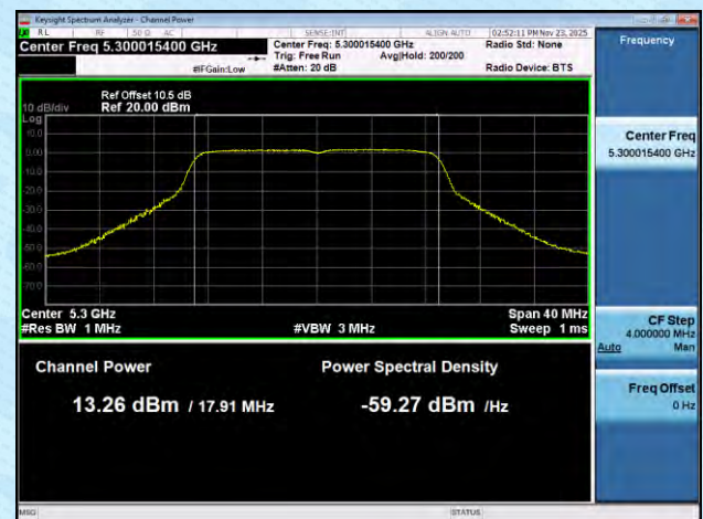
11N20MIMO-Ant8-5300-PASS
