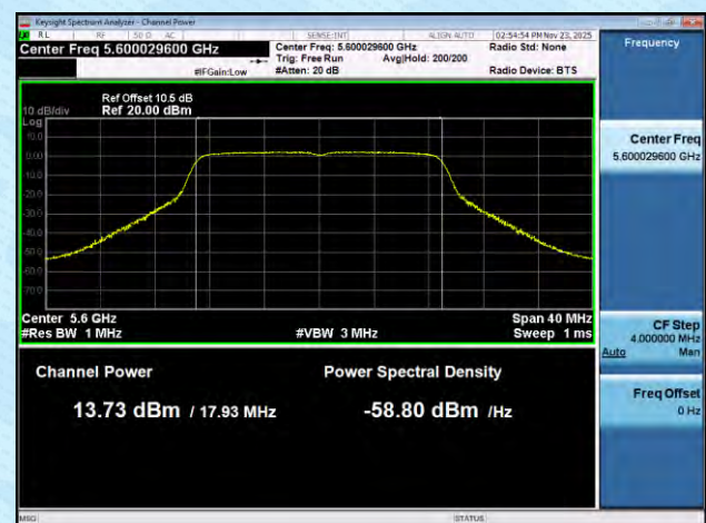
11N20MIMO-Ant8-5600-PASS
