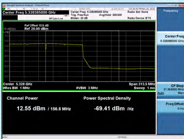
11AX160SISO-Ant6-5250_UNII-2A-PASS
