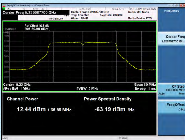
11AC40MIMO-Ant6-5230-PASS
