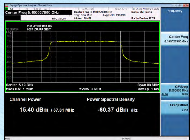
11AX40SISO-Ant8-5190-PASS
