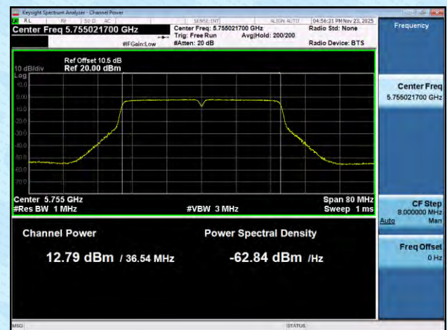
11AC40MIMO-Ant8-5755-PASS
