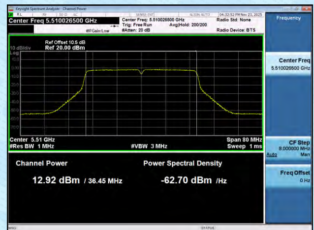
11N40MIMO-Ant8-5510-PASS
