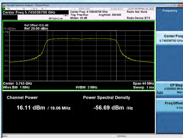
11AX20SISO-Ant6-5745-PASS
