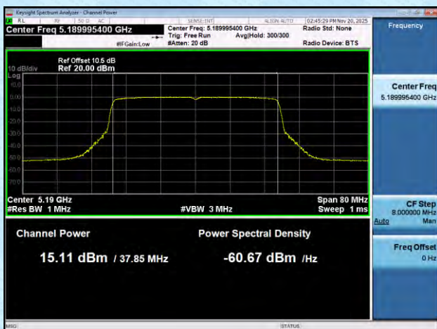
11AX40SISO-Ant6-5190-PASS
