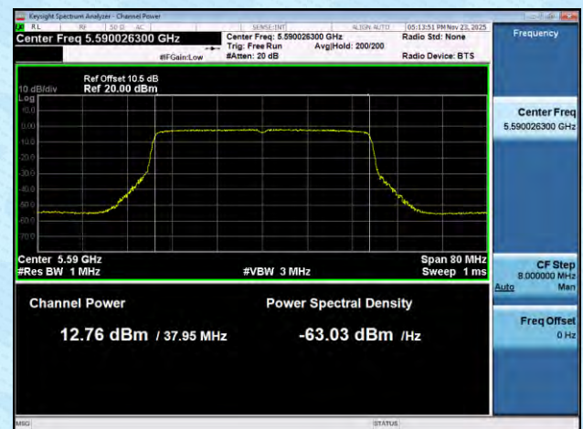
11AX40MIMO-Ant8-5590-PASS
