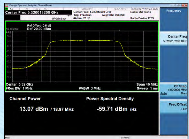
11AX20MIMO-Ant8-5320-PASS
