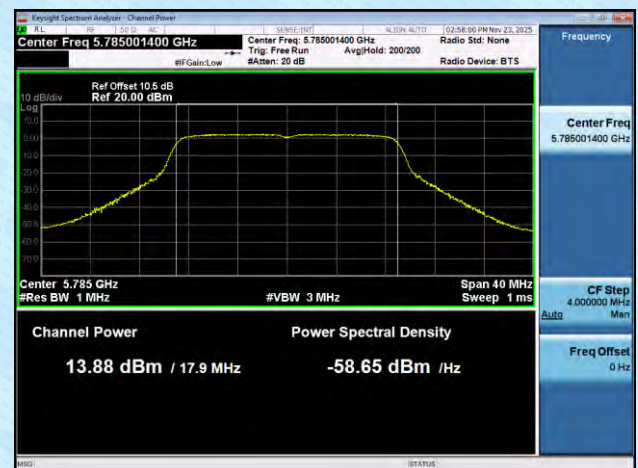
11N20MIMO-Ant8-5785-PASS
