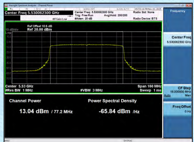
11AX80MIMO-Ant8-5530-PASS
