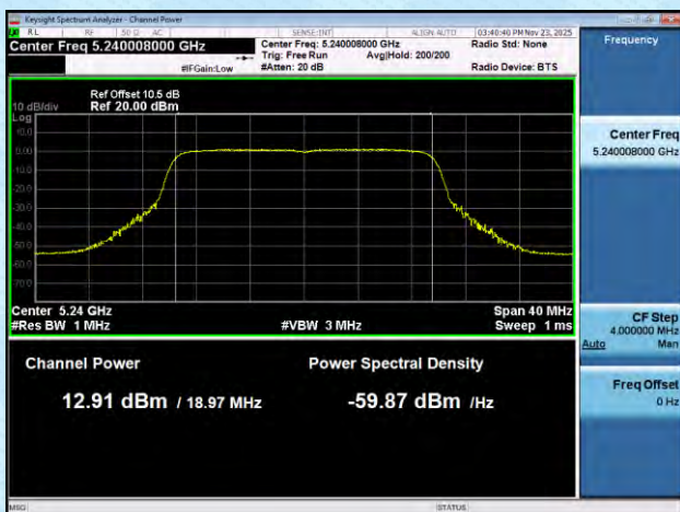
11AX20MIMO-Ant6-5240-PASS
