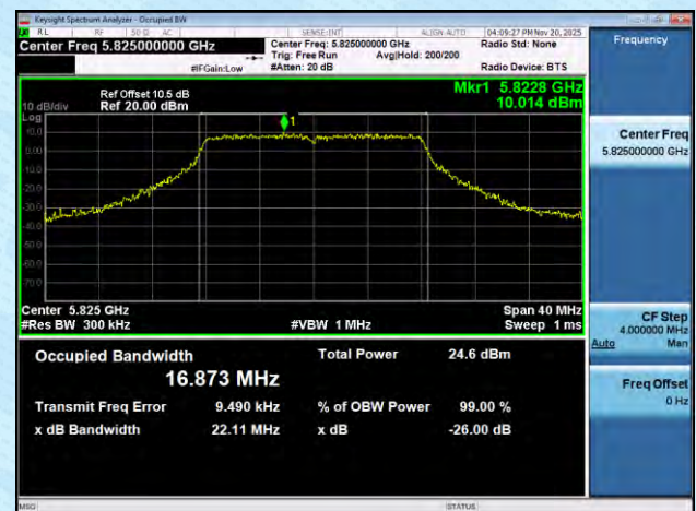
11A-Ant8-5825
