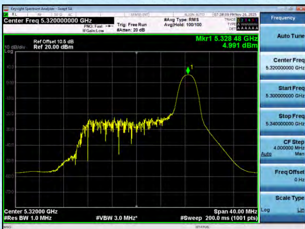
11AX20MIMO-Ant6-5320-26Tone-RU8-PASS
