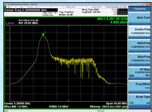
11AX20MIMO-Ant8-5300-26Tone-RU0-PASS
