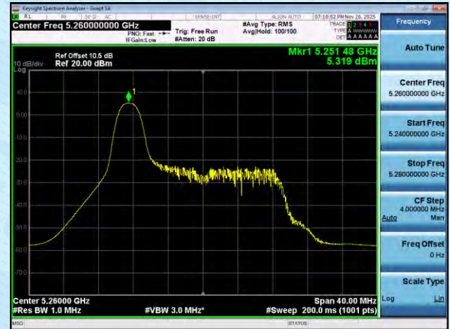
11AX20MIMO-Ant8-5260-26Tone-RU8-PASS
