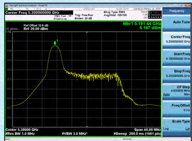
11AX20MIMO-Ant8-5200-26Tone-RU0-PASS
