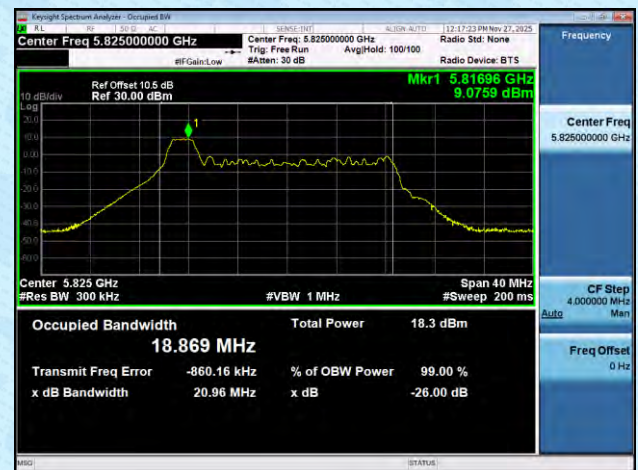
11AX20MIMO-Ant8-5825-26Tone-RU8
