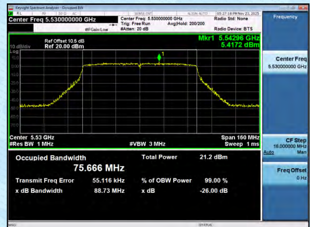
11AC80MIMO-Ant8-5530
