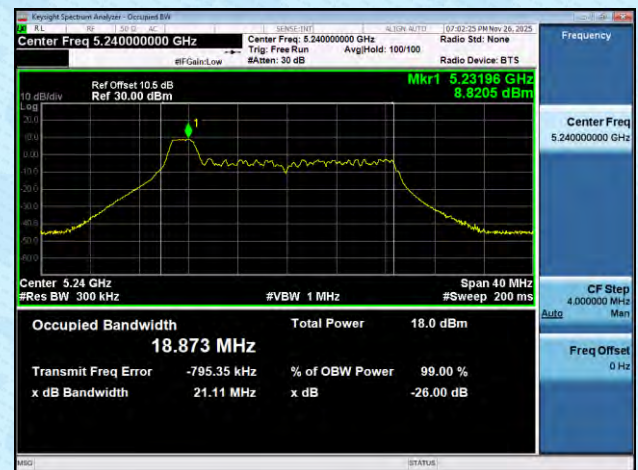
11AX20MIMO-Ant8-5240-26Tone-RU8
