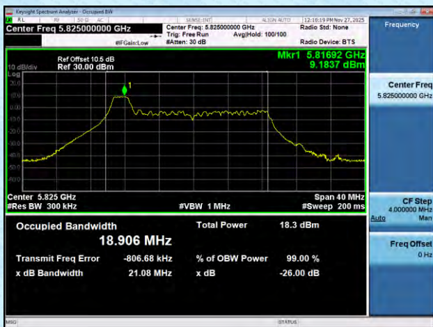
11AX20MIMO-Ant6-5825-26Tone-RU8
