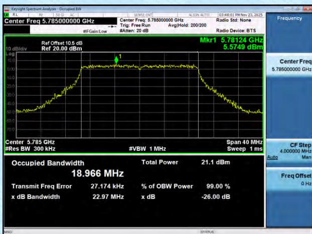
11AX20MIMO-Ant6-5785
