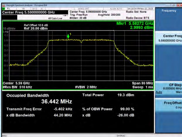
11N40MIMO-Ant6-5590
