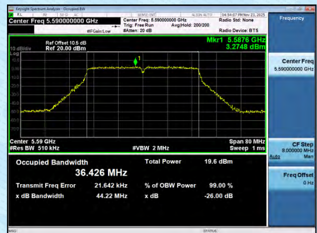
11AC40MIMO-Ant8-5590
