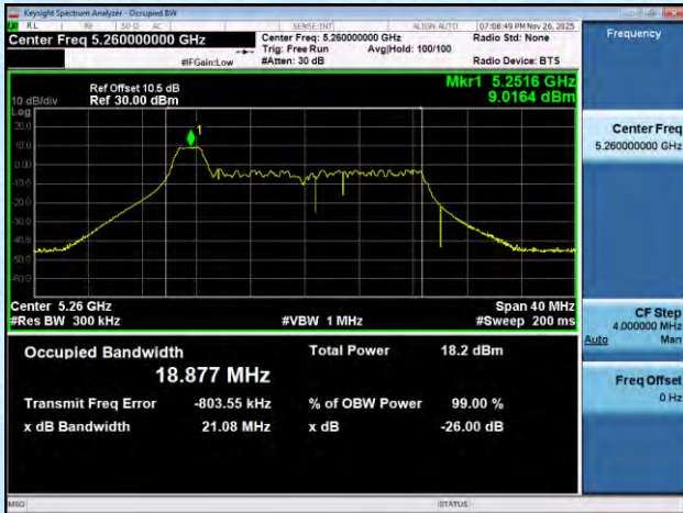
11AX20MIMO-Ant6-5260-26Tone-RU8
