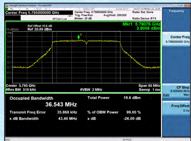
11AC40MIMO-Ant8-5795
