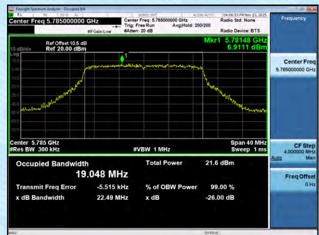
11AX20MIMO-Ant8-5785
