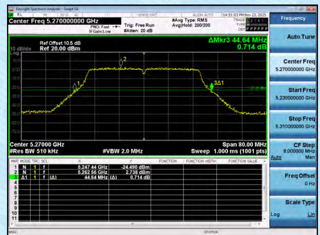
11AC40MIMO-Ant8-5270
