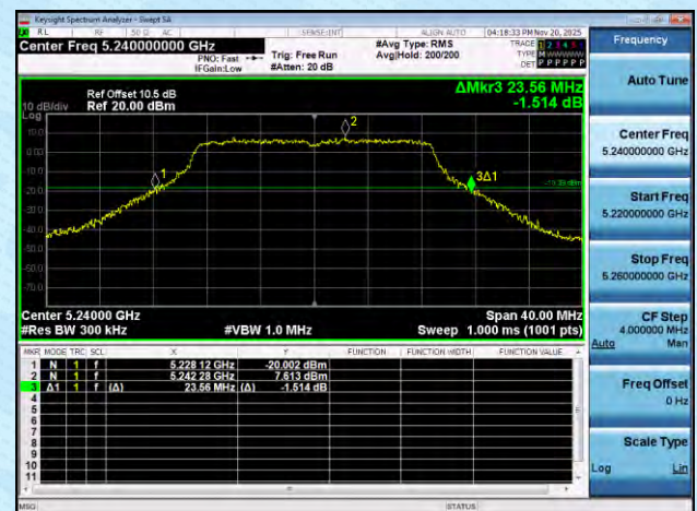
11N20SISO-Ant8-5240
