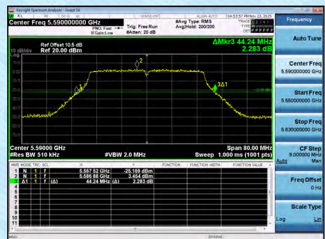
11AC40MIMO-Ant8-5590
