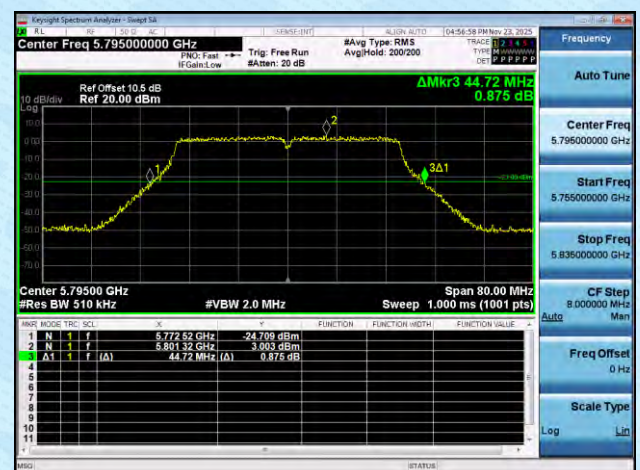
11AC40MIMO-Ant8-5795
