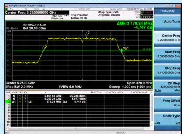
11AC160MIMO-Ant8-5250
