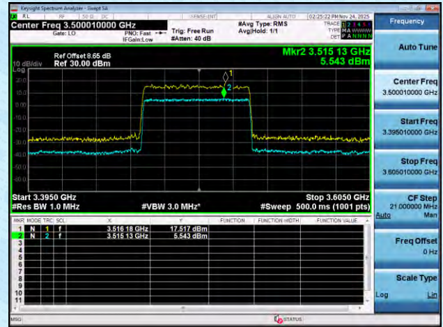
NTNT-n78(3450-3550)-PC2-30-80-M-DFT-256QAM-Outer_Full-Ant1-PASS
