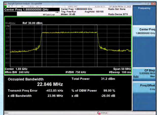
NTNV-n2-PC3-15-30-M-DFT-BPSK-Outer_Full-Ant1-PASS
