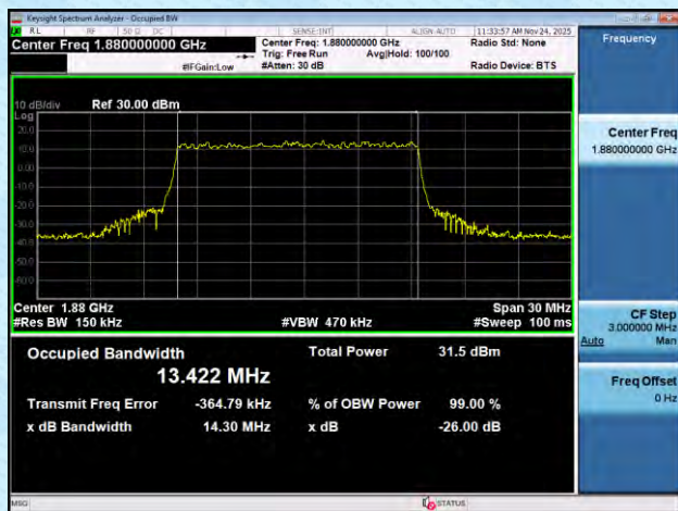
NTNV-n2-PC3-15-20-M-DFT-QPSK-Outer_Full-Ant1-PASS
