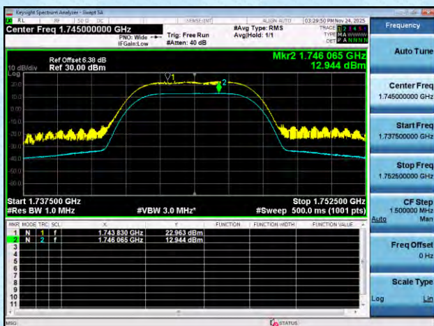
NTNT-n66-PC3-15-5-M-CP-256QAM-Outer_Full-Ant1-PASS
