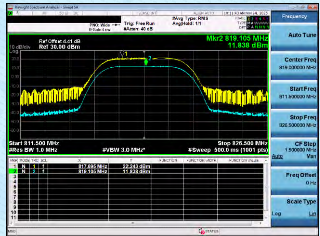
NTNT-n26(814-824)-PC3-15-10-M-DFT-QPSK-Outer_Full-Ant1-
