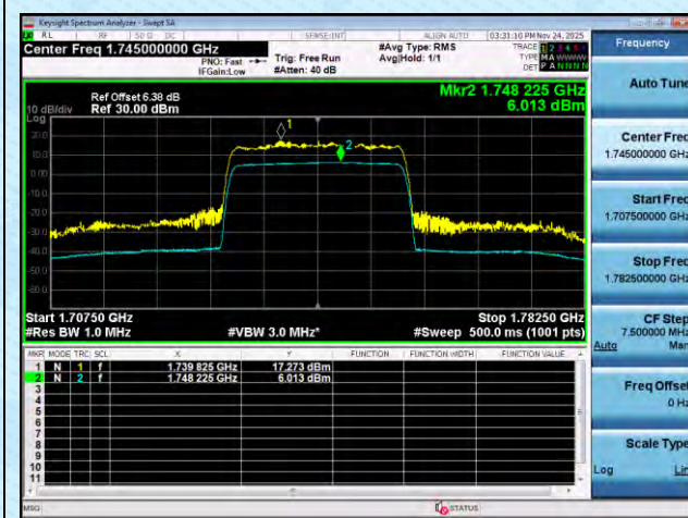
NTNT-n66-PC3-15-30-M-CP-256QAM-Outer_Full-Ant1-P ASS
