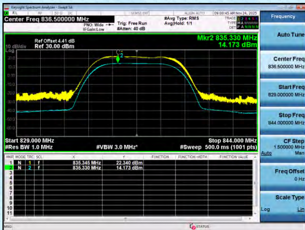
NTNT-n5-PC3-15-10-M-DFT-256QAM-Outer_Full-Ant1-PASS
