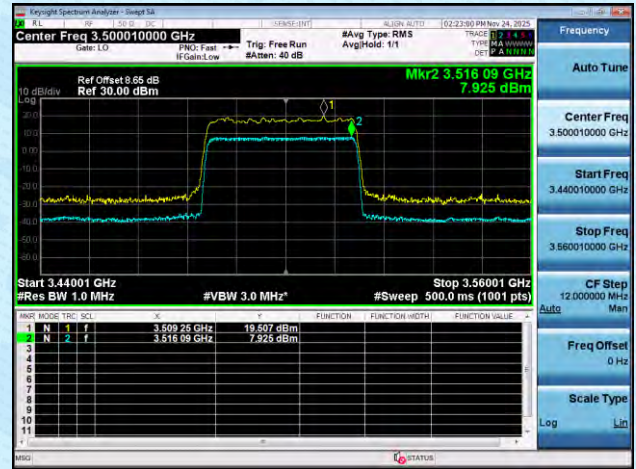
NTNT-n78(3450-3550)-PC2-30-50-M-DFT-256QAM-Outer_Full-Ant1-PASS
