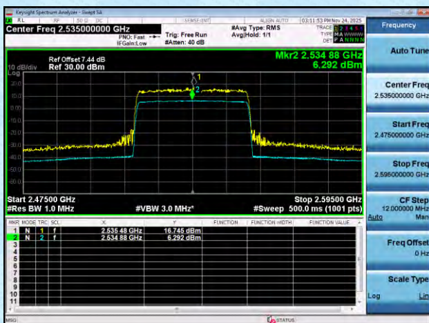
NTNT-n7-PC3-15-40-M-DFT-256QAM-Outer_Full-Ant1-PASS
