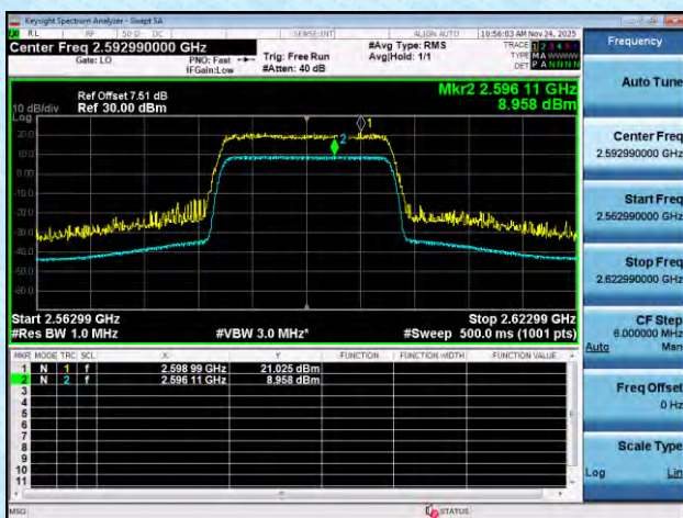
NTNT-n41-PC2-30-20-M-CP-256QAM-Outer_Full-Ant1-PASS
