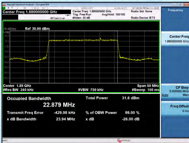
NTNV-n2-PC3-15-25-M-DFT-16QAM-Outer_Full-Ant1-PASS
