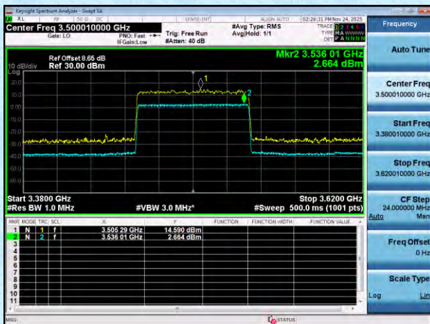
NTNT-n78(3450-3550)-PC2-30-80-M-CP-256QAM-Outer_Full-Ant1-PASS
