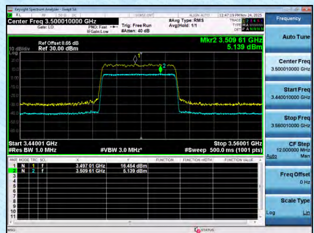
NTNT-n77(3450-3550)-PC2-30-40-M-DFT-256QAM-Outer_Full-Ant1-PASS
