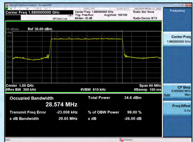
NTNV-n2-PC3-15-30-M-DFT-16QAM-Outer_Full-Ant1-PASS
