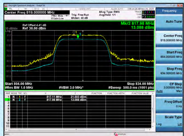
NTNT-n26(814-824)-PC3-15-10-M-DFT-64QAM-Outer_Full-Ant
