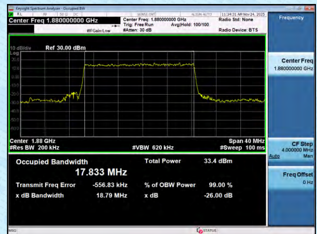
NTNV-n2-PC3-15-20-M-DFT-16QAM-Outer_Full-Ant1-PASS
