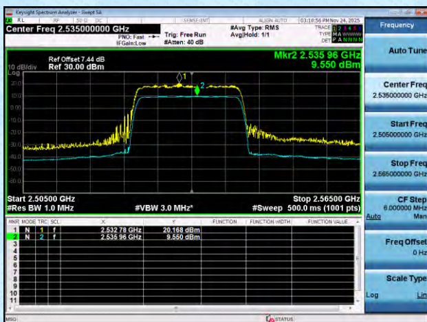
NTNT-n7-PC3-15-20-M-DFT-256QAM-Outer_Full-Ant1-PASS
