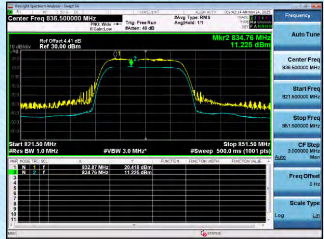
NTNT-n26(824-849)-PC3-15-15-M-DFT-256QAM-Outer_Full-Ant 1-PASS
