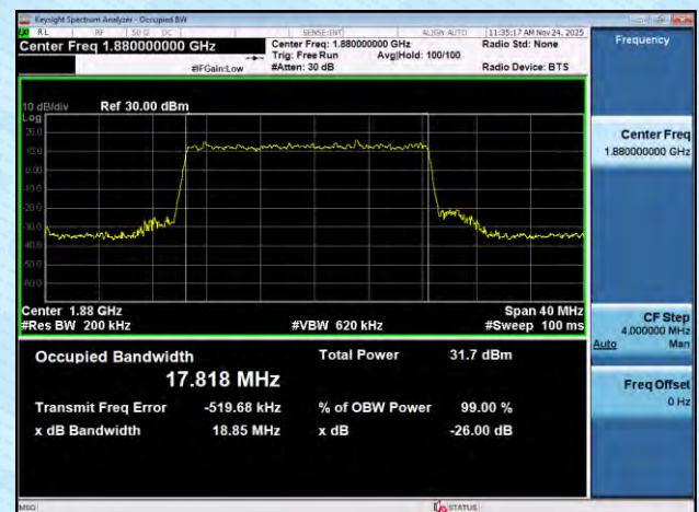
NTNV-n2-PC3-15-20-M-DFT-16QAM-Outer_Full-Ant1-PASS
