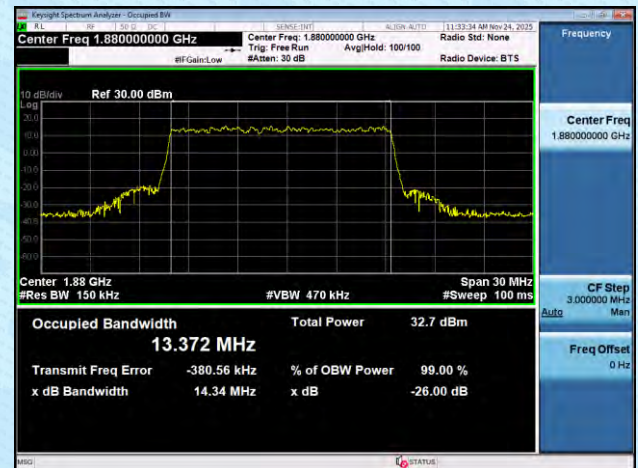
NTNV-n2-PC3-15-20-M-DFT-BPSK-Outer_Full-Ant1-PASS
