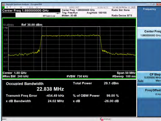
NTNV-n2-PC3-15-30-M-DFT-QPSK-Outer_Full-Ant1-PASS
