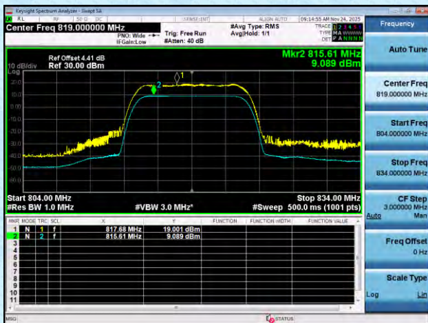
NTNT-n26(814-824)-PC3-15-10-M-CP-256QAM-Outer_Full-Ant1 -PASS
