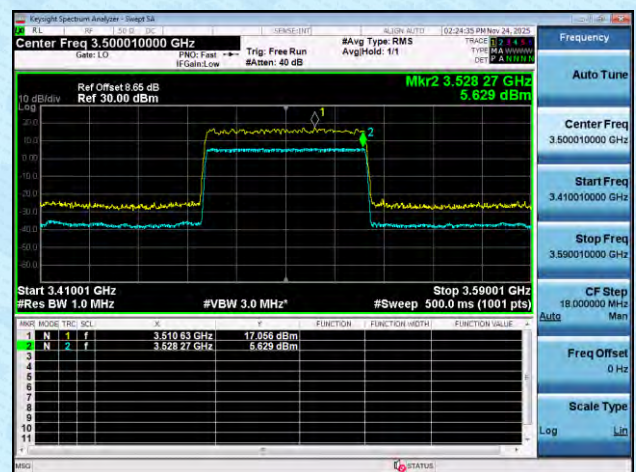
NTNT-n78(3450-3550)-PC2-30-60-M-DFT-256QAM-Outer_Full-Ant1-PASS
