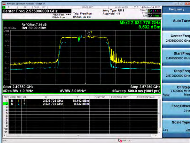
NTNT-n7-PC3-15-30-M-DFT-256QAM-Outer_Full-Ant1-PASS
