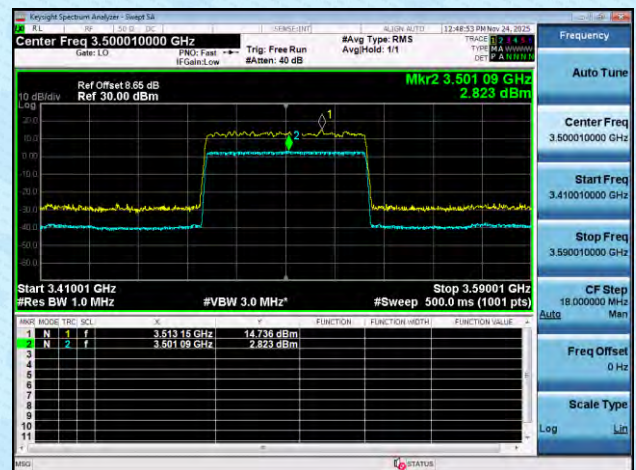
NTNT-n77(3450-3550)-PC2-30-70-M-DFT-256QAM-Outer_Full-Ant1-PASS
