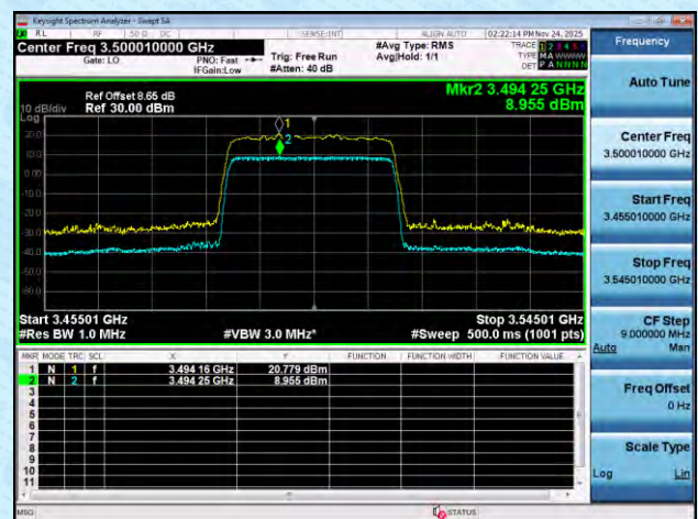
NTNT-n78(3450-3550)-PC2-30-30-M-DFT-256QAM-Outer_Full-Ant1-PASS
