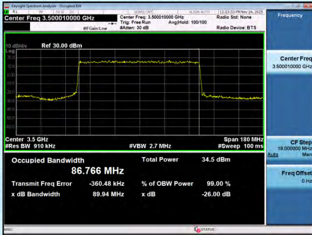
NTNV-n77(3450-3550)-PC2-30-90-M-DFT-16QAM-Outter_Full-Ant1-PASS
