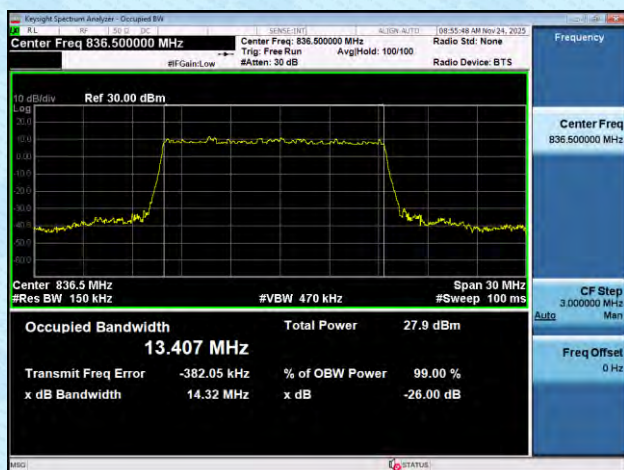
NTNV-n5-PC3-15-20-M-DFT-QPSK-Outer_Full-Ant1-PASS
