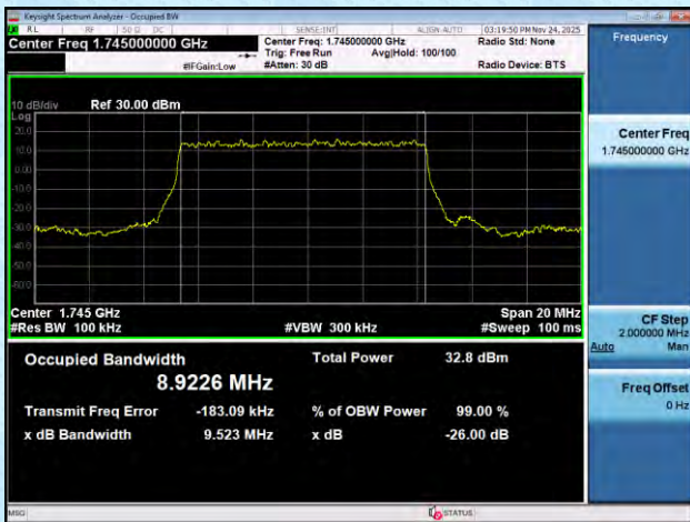
NTNV-n66-PC3-15-10-M-DFT-16QAM-Outer_Full-Ant1-PASS
