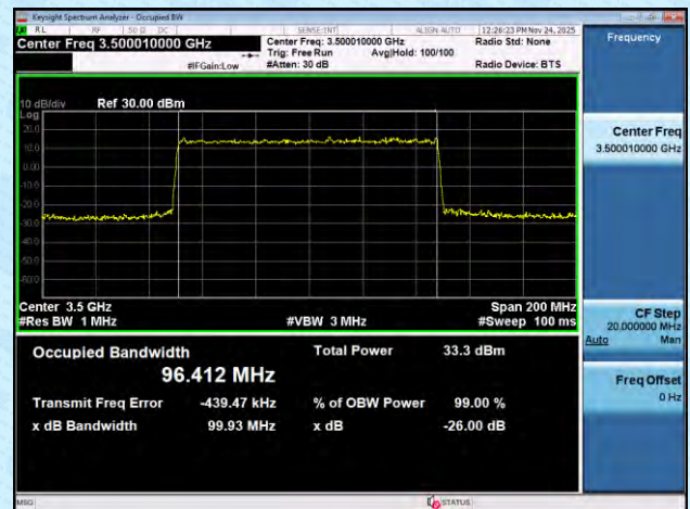
NTNV-n77(3450-3550)-PC2-30-100-M-DFT-16QAM-Outter_Full-Ant1-PASS
