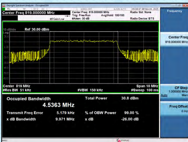
NTNV-n26(814-824)-PC3-15-5-M-DFT-QPSK-Outer_Full-Ant1-PASS
