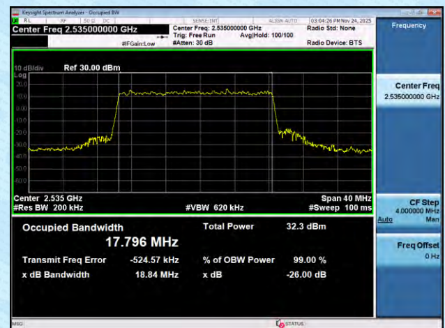
NTNV-n7-PC3-15-20-M-DFT-16QAM-Outer_Full-Ant1-PASS
