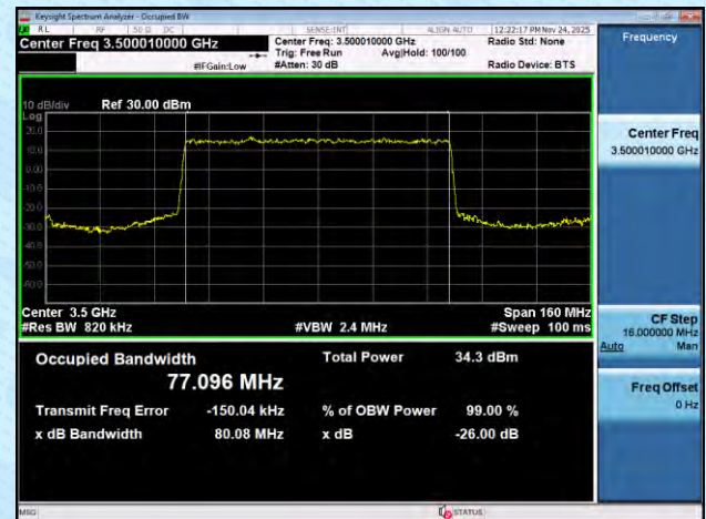
NTNV-n77(3450-3550)-PC2-30-80-M-DFT-16QAM-Outet_Full-A nt1-PASS
