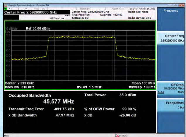
NTNV-n41-PC2-30-50-M-DFT-16QAM-Outer_Full-Ant1-PASS
