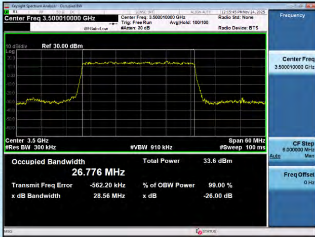
NTNV-n77(3450-3550)-PC2-30-30-M-DFT-16QAM-Outet_Full-A nt1-PASS
