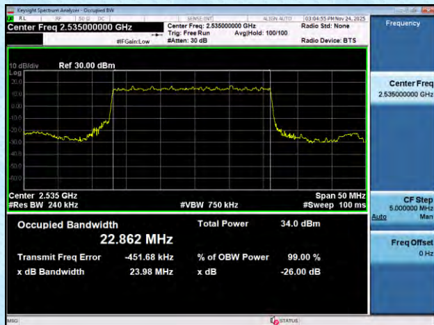
NTNV-n7-PC3-15-25-M-DFT-16QAM-Outer_Full-Ant1-PASS
