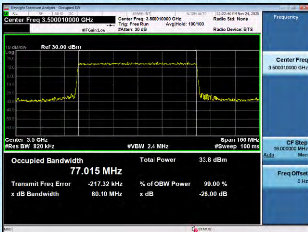
NTNV-n77(3450-3550)-PC2-30-80-M-DFT-QPSK-Outet_Full-An t1-PASS
