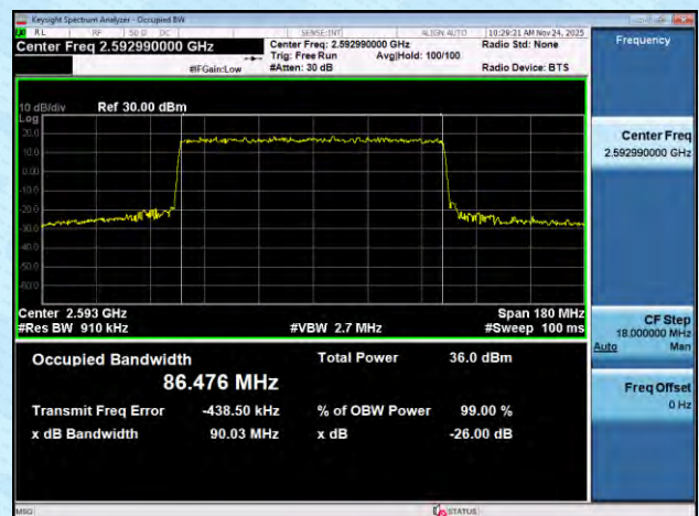
NTNV-n41-PC2-30-90-M-DFT-16QAM-Outer_Full-Ant1-PASS
