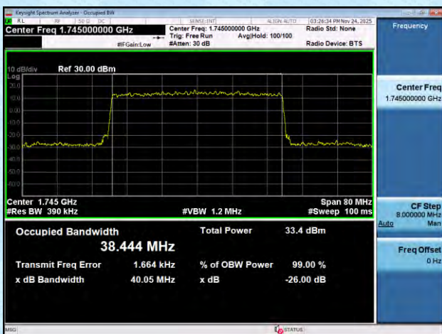
NTNV-n66-PC3-15-40-M-DFT-QPSK-Outer_Full-Ant1-PASS
