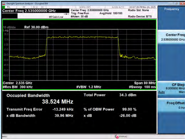
NTNV-n7-PC3-15-40-M-DFT-BPSK-Outer_Full-Ant1-PASS
