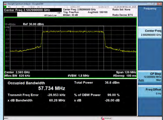
NTNV-n41-PC2-30-70-M-DFT-BPSK-Outer_Full-Ant1-PASS
