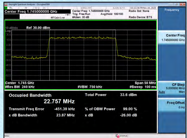
NTNV-n66-PC3-15-25-M-DFT-16QAM-Outer_Full-Ant1-PASS
