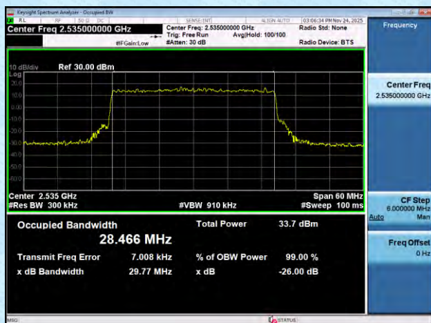
NTNV-n7-PC3-15-30-M-DFT-QPSK-Outer_Full-Ant1-PASS
