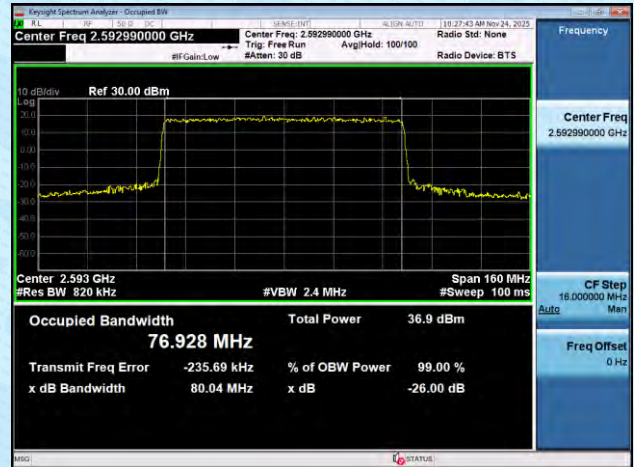
NTNV-n41-PC2-30-90-M-DFT-BPSK-Outer_Full-Ant1-PASS
