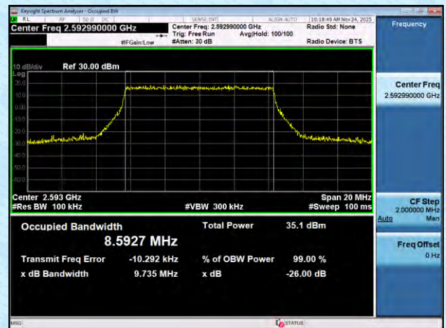
NTNV-n41-PC2-30-10-M-DFT-16QAM-Outet_Full-Ant1-PASS
