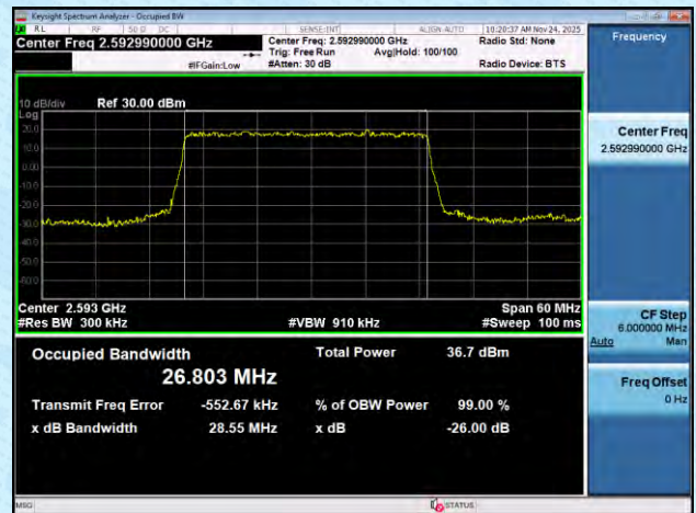
NTNV-n41-PC2-30-30-M-DFT-16QAM-Outer_Full-Ant1-PASS
