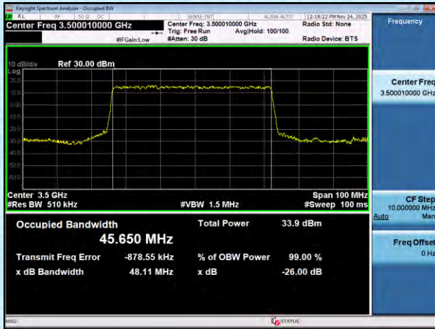
NTNV-n77(3450-3550)-PC2-30-50-M-DFT-16QAM-Outet_Full-A nt1-PASS
