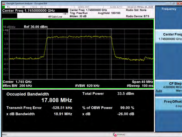
NTNV-n66-PC3-15-20-M-DFT-16QAM-Outer_Full-Ant1-PASS
