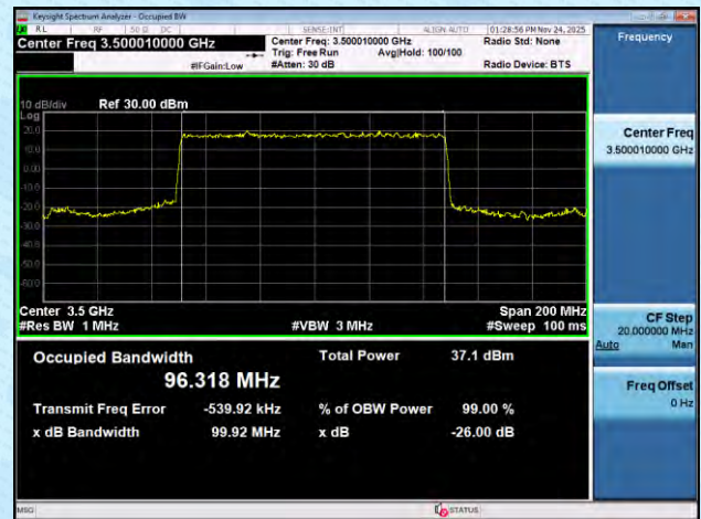
NTNV-n78(3450-3550)-PC2-30-100-M-DFT-16QAM-Outet_Full-Ant1-PASS
