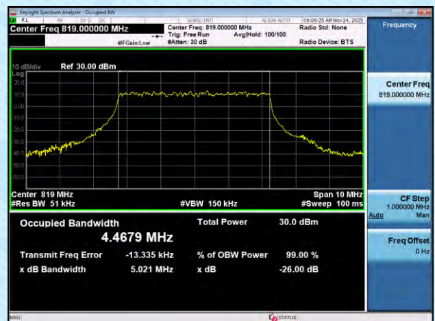
NTNV-n26(814-824)-PC3-15-5-M-DFT-16QAM-Outer_Full-Ant1-PASS
