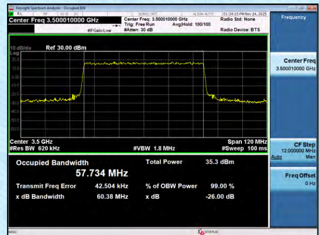
NTNV-n78(3450-3550)-PC2-30-60-M-DFT-16QAM-Outter_Full-A nt1-PASS
