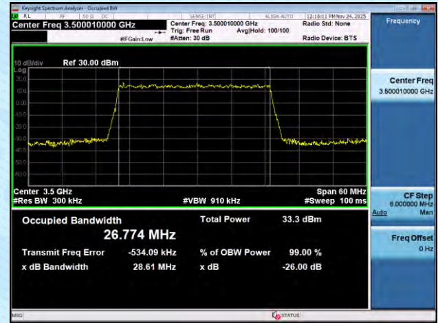
NTNV-n77(3450-3550)-PC2-30-40-M-DFT-BPSK-Outet_Full-An t1-PASS
