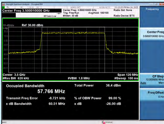
NTNV-n78(3450-3550)-PC2-30-60-M-DFT-QPSK-Outter_Full-An t1-PASS
