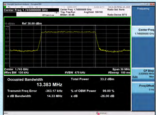
NTNV-n66-PC3-15-15-M-DFT-16QAM-Outer_Full-Ant1-PASS
