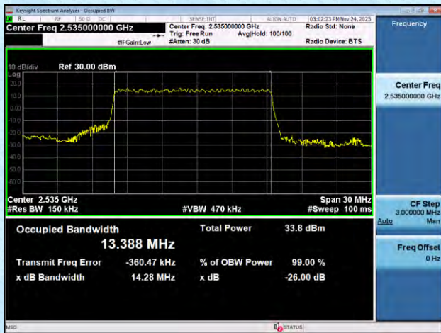
NTNV-n7-PC3-15-15-M-DFT-16QAM-Outer_Full-Ant1-PASS
