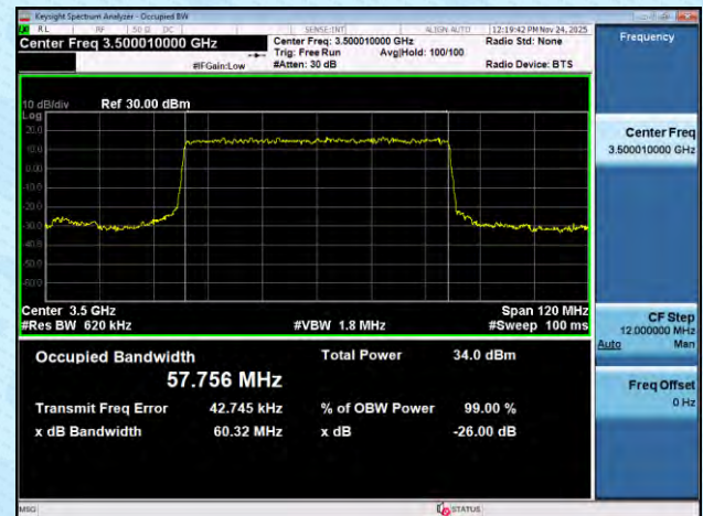
NTNV-n77(3450-3550)-PC2-30-60-M-DFT-16QAM-Outet_Full-A nt1-PASS
