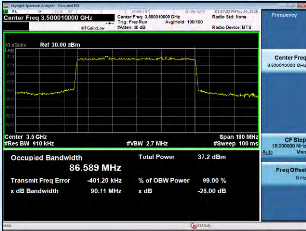
NTNV-n78(3450-3550)-PC2-30-90-M-DFT-16QAM-Outet_Full-Ant1-PASS
