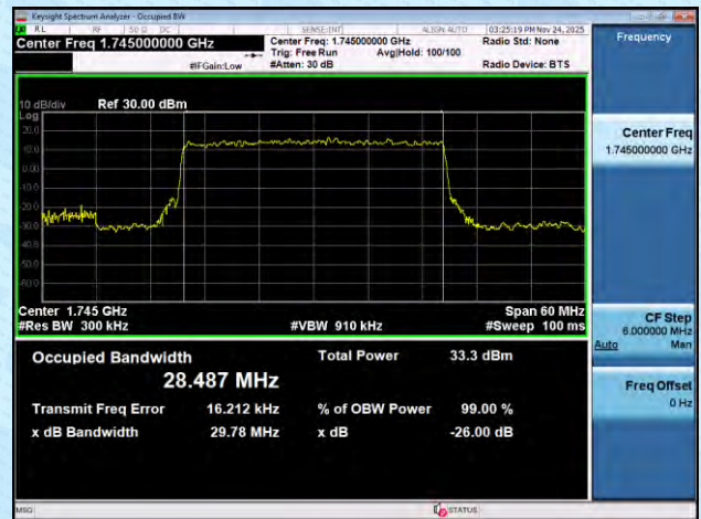
NTNV-n66-PC3-15-40-M-DFT-BPSK-Outer_Full-Ant1-PASS
