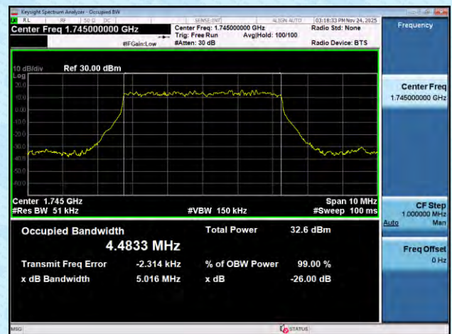
NTNV-n66-PC3-15-5-M-DFT-16QAM-Outer_Full-Ant1-PASS
