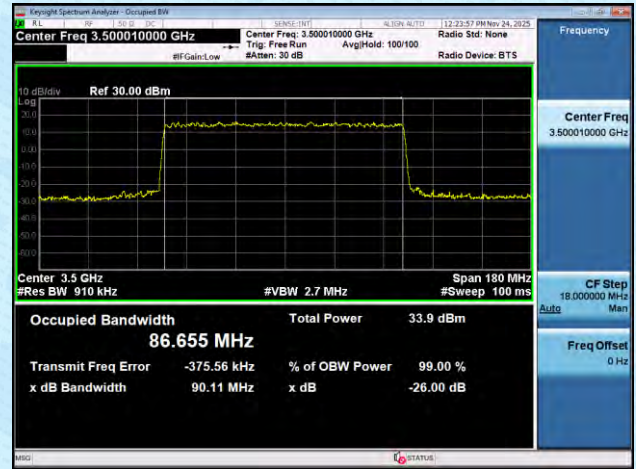
NTNV-n77(3450-3550)-PC2-30-100-M-DFT-BPSK-Outter_Full-Ant1-PASS
