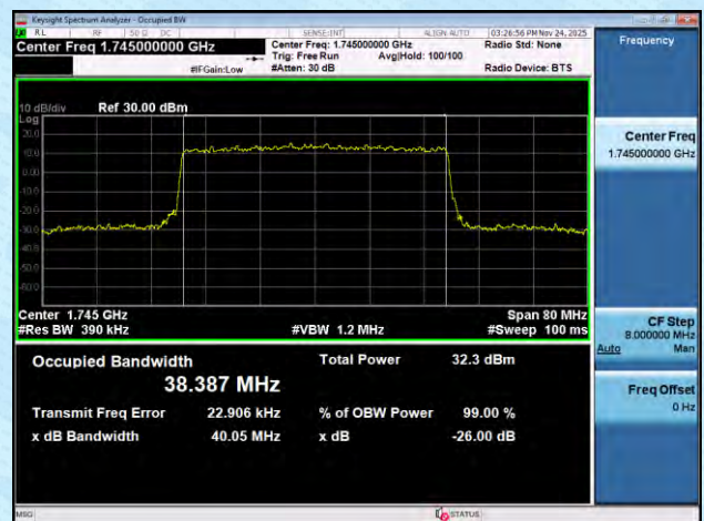
NTNV-n66-PC3-15-40-M-DFT-16QAM-Outer_Full-Ant1-PASS
