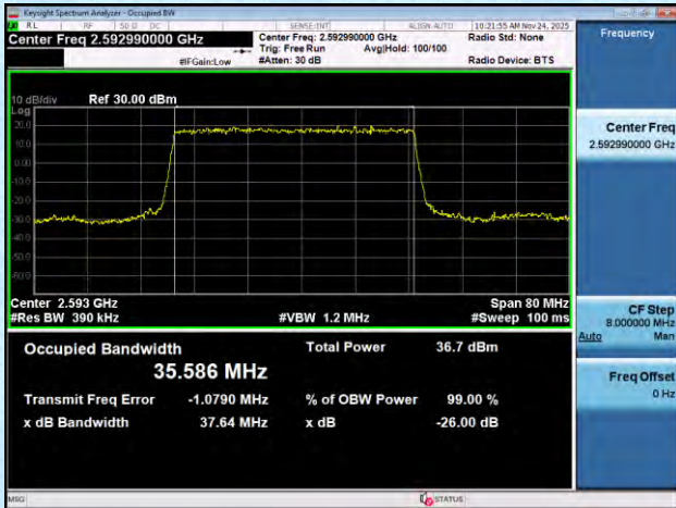
NTNV-n41-PC2-30-40-M-DFT-16QAM-Outer_Full-Ant1-PASS
