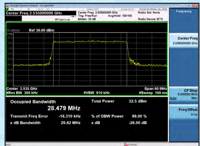
NTNV-n7-PC3-15-30-M-DFT-16QAM-Outer_Full-Ant1-PASS
