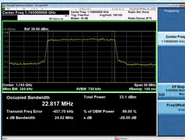
NTNV-n66-PC3-15-25-M-DFT-QPSK-Outer_Full-Ant1-PASS
