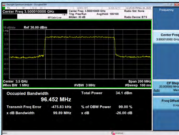
NTNV-n77(3450-3550)-PC2-30-100-M-DFT-QPSK-Outter_Full-Ant1-PASS
