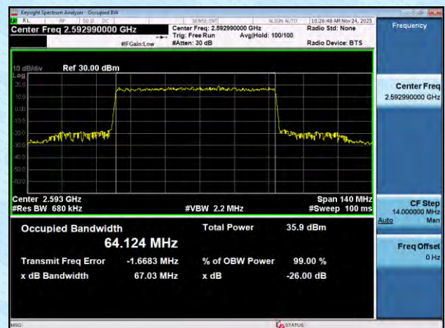
NTNV-n41-PC2-30-70-M-DFT-16QAM-Outer_Full-Ant1-PASS
