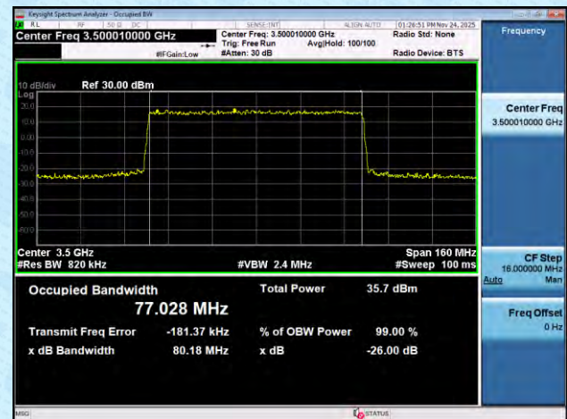
NTNV-n78(3450-3550)-PC2-30-80-M-DFT-16QAM-Outet_Full-A nt1-PASS
