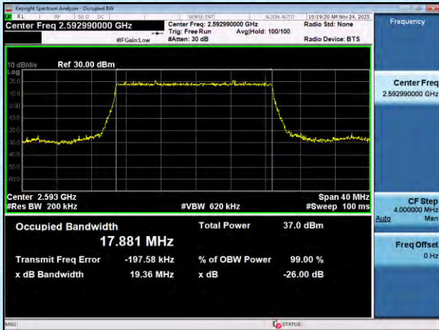
NTNV-n41-PC2-30-20-M-DFT-16QAM-Outer_Full-Ant1-PASS
