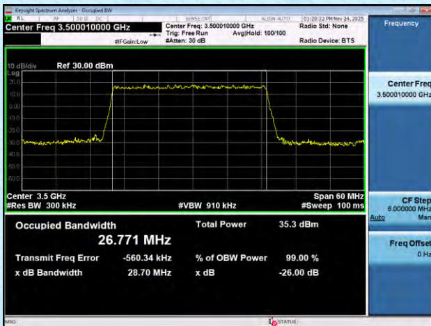
NTNV-n78(3450-3550)-PC2-30-40-M-DFT-QPSK-Outet_Full-An t1-PASS
