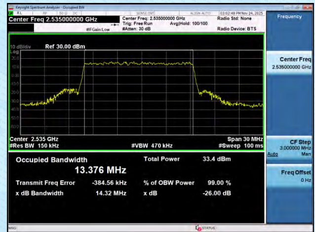
NTNV-n7-PC3-15-20-M-DFT-BPSK-Outer_Full-Ant1-PASS
