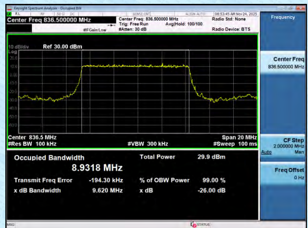
NTNV-n5-PC3-15-10-M-DFT-16QAM-Outer_Full-Ant1-PASS
