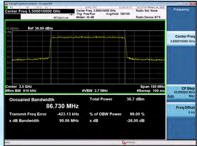
NTNV-n78(3450-3550)-PC2-30-100-M-DFT-BPSK-Outet_Full-Ant1-PASS
