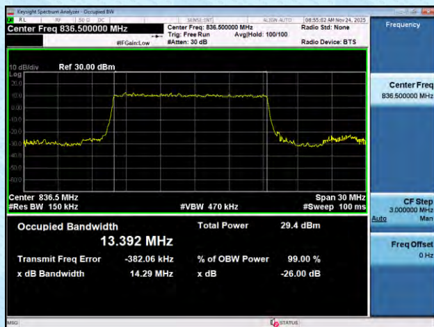
NTNV-n5-PC3-15-15-M-DFT-16QAM-Outer_Full-Ant1-PASS
