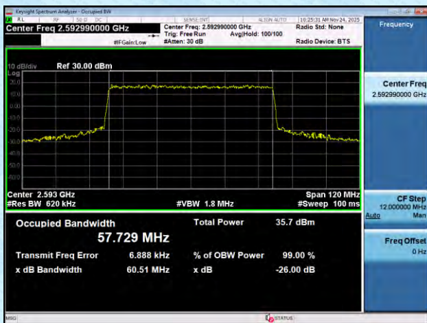
NTNV-n41-PC2-30-70-M-DFT-QPSK-Outer_Full-Ant1-PASS
