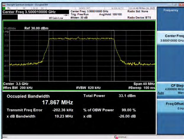
NTNV-n77(3450-3550)-PC2-30-20-M-DFT-QPSK-Outet_Full-An t1-PASS
