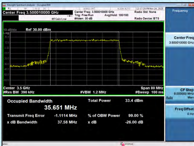
NTNV-n77(3450-3550)-PC2-30-40-M-DFT-QPSK-Outet_Full-An t1-PASS
