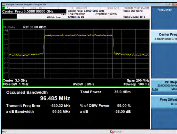
NTNV-n78(3450-3550)-PC2-30-100-M-DFT-QPSK-Outet_Full-Ant1-PASS
