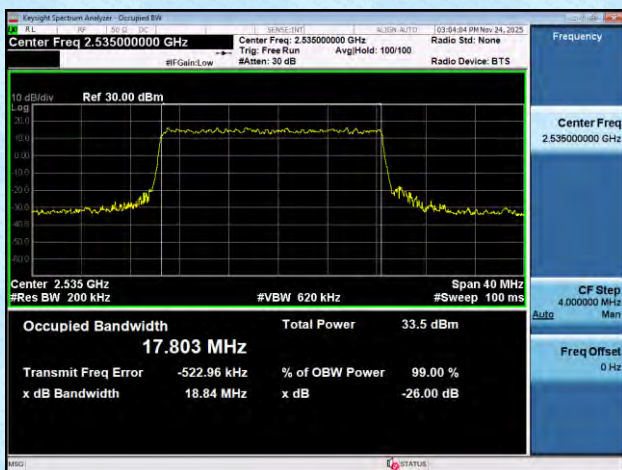
NTNV-n7-PC3-15-20-M-DFT-QPSK-Outer_Full-Ant1-PASS
