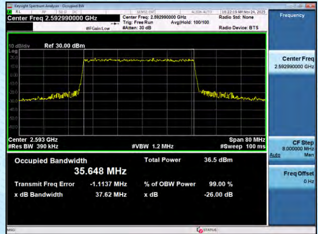
NTNV-n41-PC2-30-50-M-DFT-BPSK-Outer_Full-Ant1-PASS
