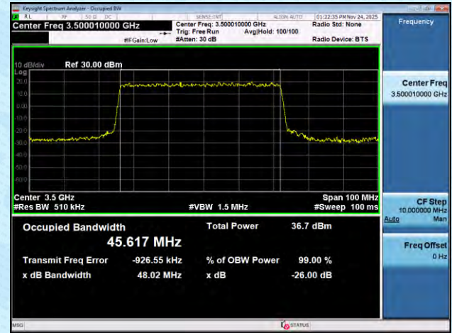
NTNV-n78(3450-3550)-PC2-30-60-M-DFT-BPSK-Outter_Full-An t1-PASS
