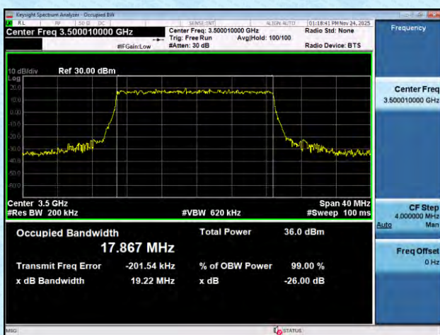
NTNV-n78(3450-3550)-PC2-30-20-M-DFT-QPSK-Outet_Full-An t1-PASS
