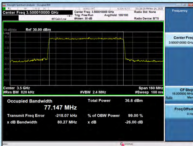
NTNV-n78(3450-3550)-PC2-30-80-M-DFT-QPSK-Outet_Full-An t1-PASS
