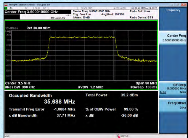
NTNV-n78(3450-3550)-PC2-30-40-M-DFT-16QAM-Outet_Full-A nt1-PASS
