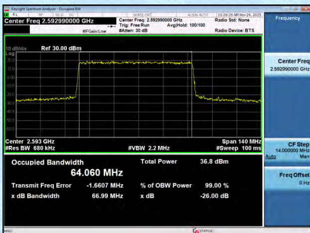
NTNV-n41-PC2-30-70-M-DFT-QPSK-Outer_Full-Ant1-PASS
