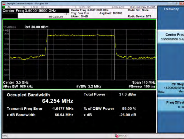
NTNV-n78(3450-3550)-PC2-30-70-M-DFT-16QAM-Outet_Full-A nt1-PASS
