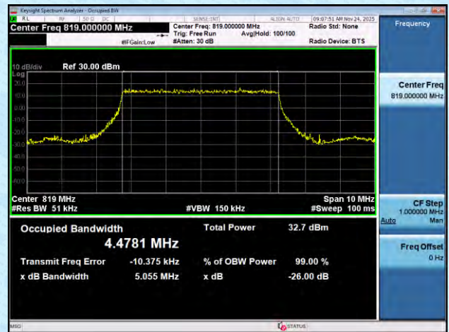
NTNV-n26(814-824)-PC3-15-5-M-DFT-16QAM-Outer_Full-Ant1-PASS
