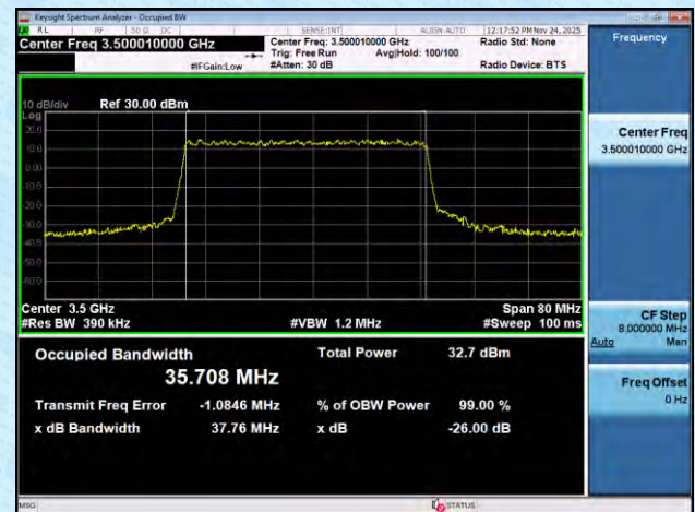
NTNV-n77(3450-3550)-PC2-30-40-M-DFT-16QAM-Outet_Full-A nt1-PASS
