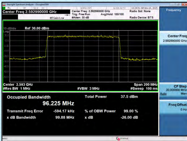
NTNV-n41-PC2-30-100-M-DFT-16QAM-Outer_Full-Ant1-PASS
