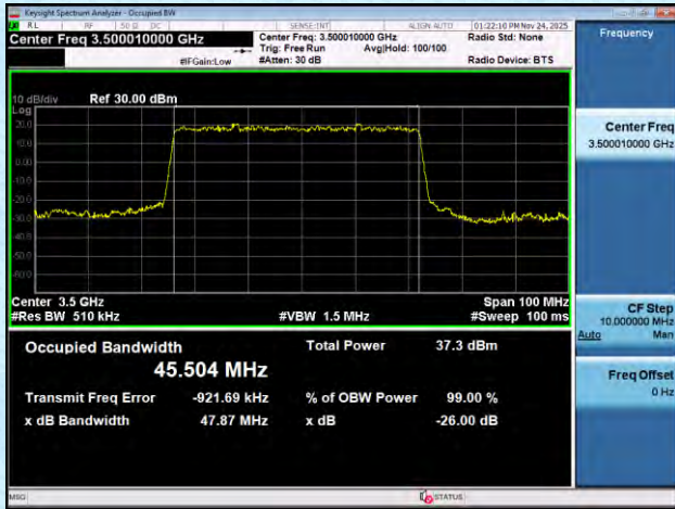
NTNV-n78(3450-3550)-PC2-30-50-M-DFT-16QAM-Outter_Full-A nt1-PASS
