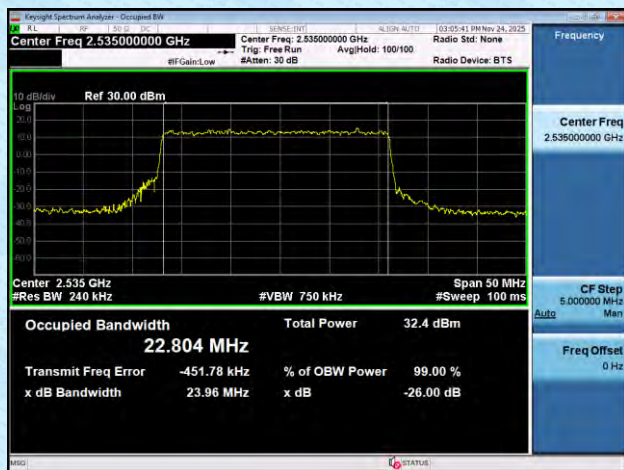
NTNV-n7-PC3-15-30-M-DFT-QPSK-Outer_Full-Ant1-PASS
