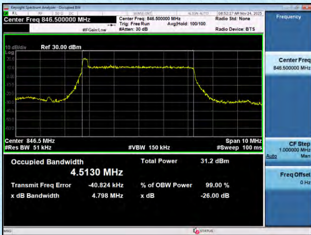
NTNV-n5-PC3-15-5-H-DFT-16QAM-Outer_Full-Ant1-PASS
