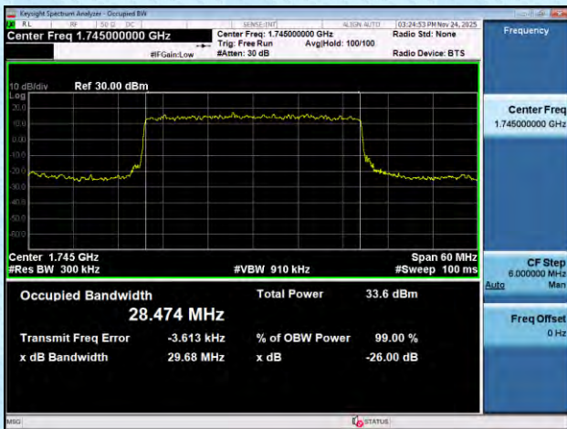
NTNV-n66-PC3-15-30-M-DFT-16QAM-Outer_Full-Ant1-PASS
