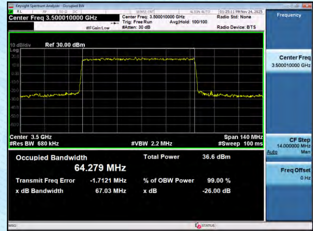
NTNV-n78(3450-3550)-PC2-30-80-M-DFT-BPSK-Outet_Full-An t1-PASS
