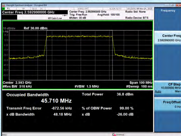
NTNV-n41-PC2-30-50-M-DFT-QPSK-Outer_Full-Ant1-PASS
