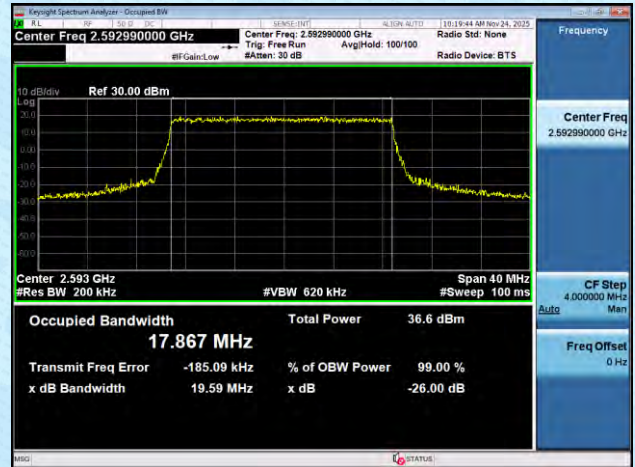
NTNV-n41-PC2-30-30-M-DFT-BPSK-Outer_Full-Ant1-PASS
