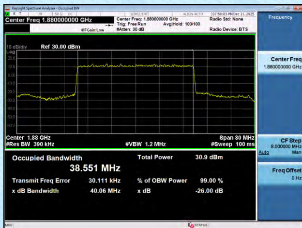
NTNV-n2-PC3-15-40-M-DFT-16QAM-Outer_Full-Ant1-PASS
