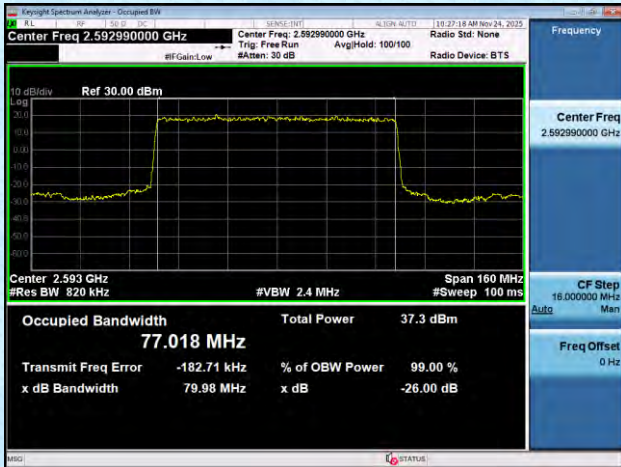
NTNV-n41-PC2-30-80-M-DFT-16QAM-Outer_Full-Ant1-PASS
