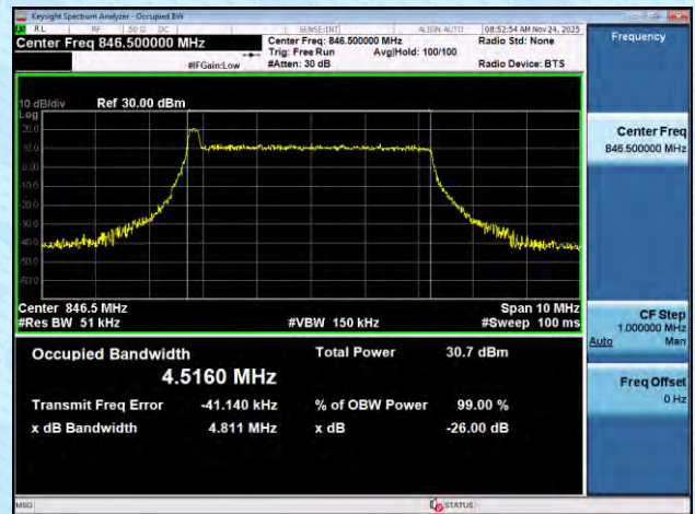
NTNV-n5-PC3-15-10-M-DFT-BPSK-Outer_Full-Ant1-PASS
