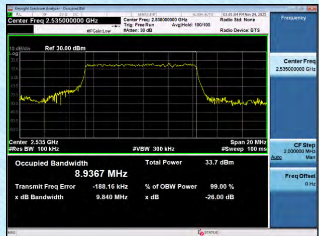
NTNV-n7-PC3-15-10-M-DFT-16QAM-Outer_Full-Ant1-PASS
