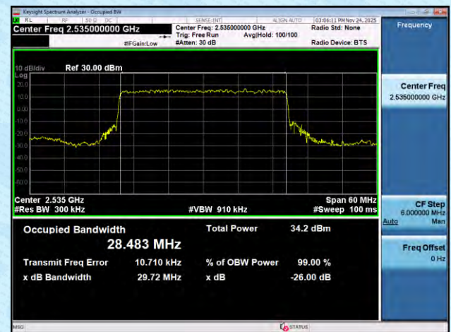
NTNV-n7-PC3-15-30-M-DFT-16QAM-Outer_Full-Ant1-PASS
