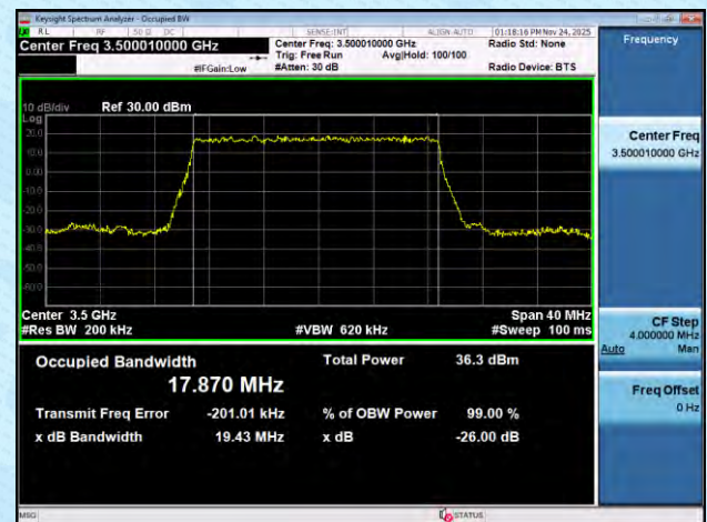
NTNV-n78(3450-3550)-PC2-30-20-M-DFT-16QAM-Outet_Full-A nt1-PASS
