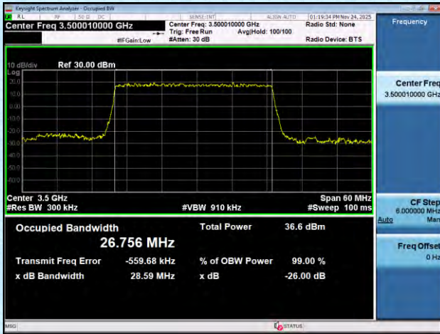
NTNV-n78(3450-3550)-PC2-30-30-M-DFT-16QAM-Outet_Full-A nt1-PASS
