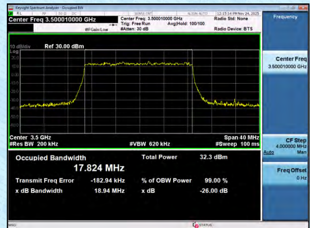
NTNV-n77(3450-3550)-PC2-30-20-M-DFT-16QAM-Outet_Full-A nt1-PASS
