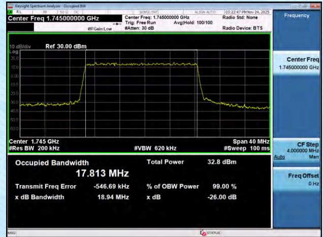
NTNV-n66-PC3-15-25-M-DFT-BPSK-Outer_Full-Ant1-PASS
