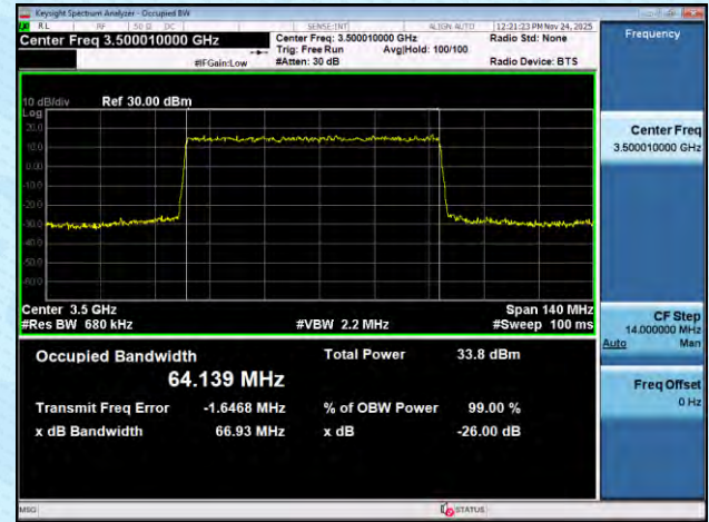
NTNV-n77(3450-3550)-PC2-30-80-M-DFT-BPSK-Outet_Full-An t1-PASS
