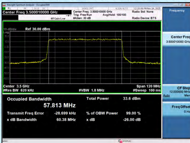
NTNV-n77(3450-3550)-PC2-30-60-M-DFT-QPSK-Outet_Full-An t1-PASS
