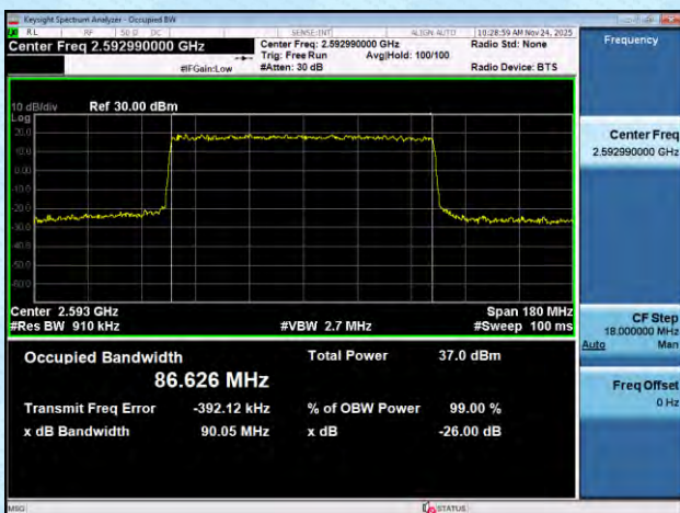
NTNV-n41-PC2-30-90-M-DFT-QPSK-Outer_Full-Ant1-PASS
