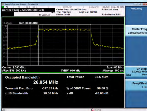
NTNV-n41-PC2-30-30-M-DFT-QPSK-Outer_Full-Ant1-PASS
