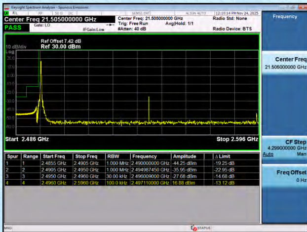
NTNV-n41-PC2-30-100-H-DFT-BPSK-Edge_1RB_Right-PASS
