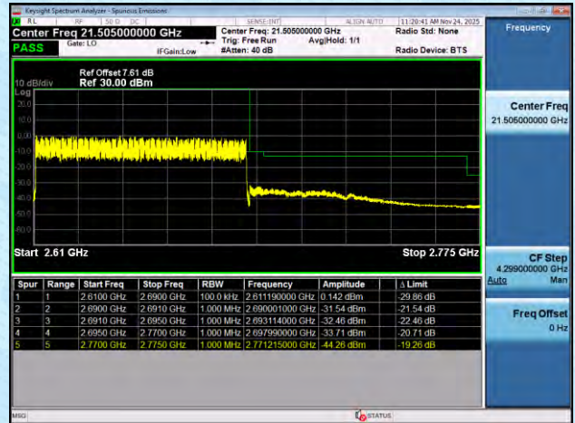
NTNV-n41-PC2-30-90-L-DFT-BPSK-Outer_Full-PASS
