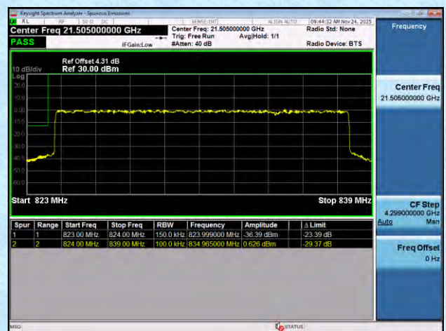
NTNV-n26(824-849)-PC3-15-15-L-DFT-BPSK-Outer_Full-PA
