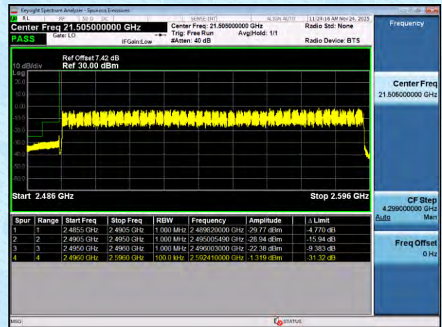
NTNV-n41-PC2-30-100-H-DFT-BPSK-Outer_Full-PASS
