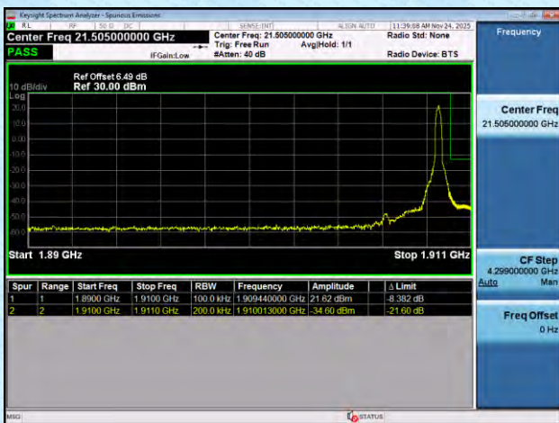
NTNV-n2-PC3-15-25-L-DFT-BPSK-Edge_1RB_Left-PASS
