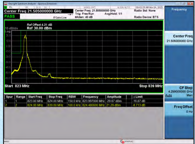
NTNV-n5-PC3-15-15-H-DFT-BPSK-Edge_1RB_Right-PASS
