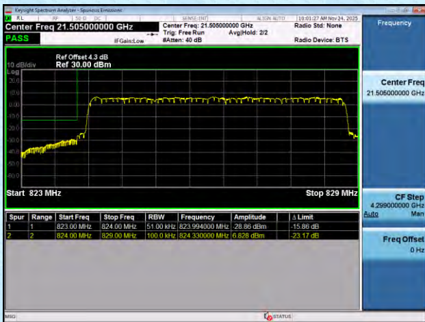
NTNV-n5-PC3-15-5-H-DFT-BPSK-Outer_Full-PASS
