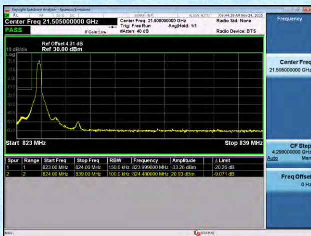
NTNV-n26(824-849)-PC3-15-15-L-DFT-BPSK-Edge_1RB_Left-PA
