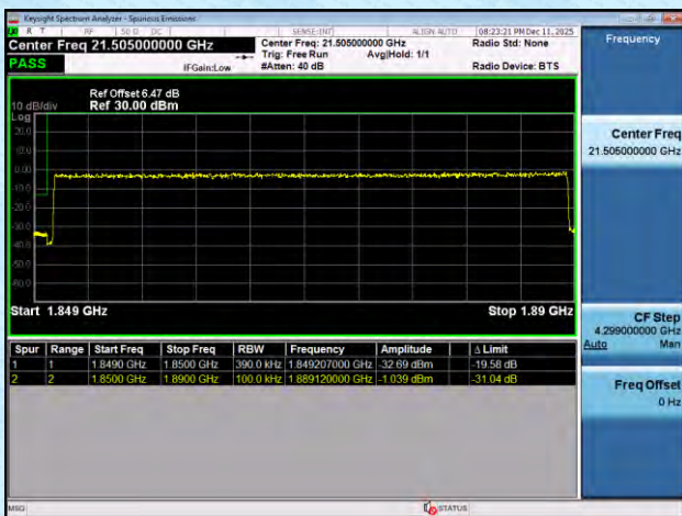
NTNV-n2-PC3-15-40-H-DFT-BPSK-Outer_Full-PASS
