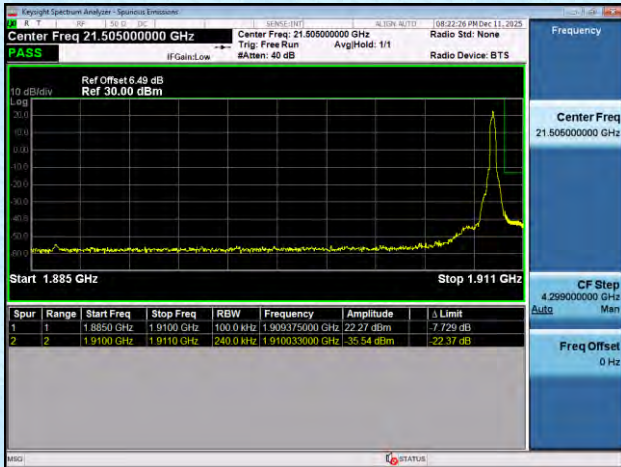
NTNV-n2-PC3-15-25-H-CP-256QAM-Edge_1RB_Right-PASS
