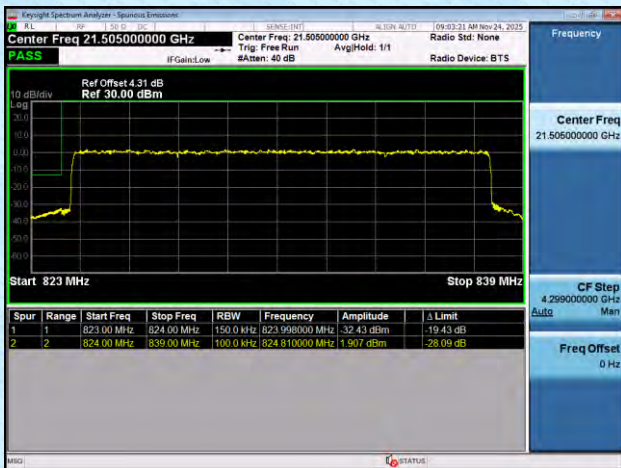
NTNV-n5-PC3-15-15-H-DFT-BPSK-Outer_Full-PASS
