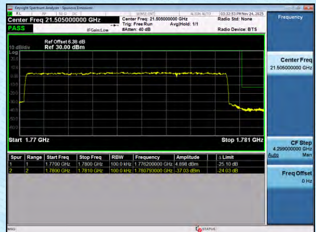
NTNV-n66-PC3-15-10-H-DFT-BPSK-Outer_Full-PASS
