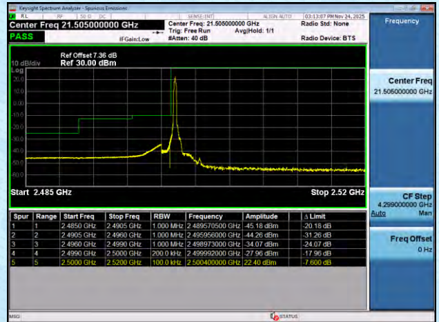
NTNV-n7-PC3-15-10-H-DFT-BPSK-Edge_1RB_Right-PASS
