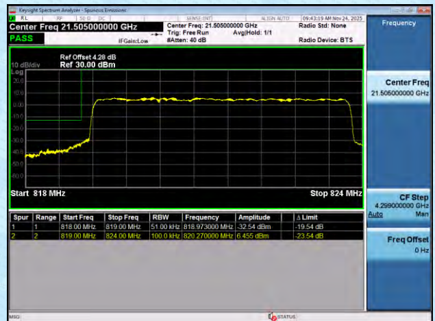
NTNV-n26(824-849)-PC3-15-5-H-DFT-BPSK-Outer_Full-PA
