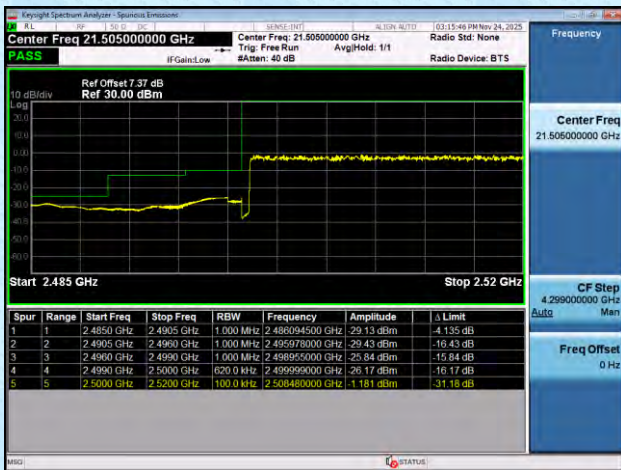
NTNV-n7-PC3-15-30-H-DFT-BPSK-Outer_Full-PASS
