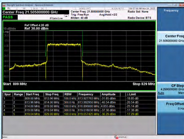
NTNV-n26(814-824)-PC3-15-5-H-DFT-BPSK-Outer_Full-PA SS
