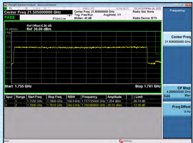
NTNV-n66-PC3-15-25-H-DFT-BPSK-Outer_Full-PASS
