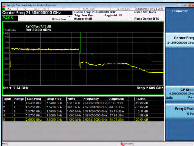
NTNV-n7-PC3-15-40-L-DFT-BPSK-Outer_Full-PASS
