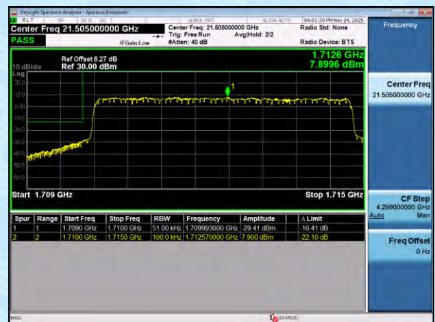
NTNV-n66-PC3-15-5-L-DFT-BPSK-Outer_Full-PASS
