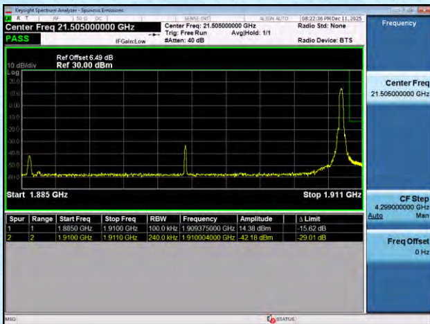
NTNV-n2-PC3-15-30-L-DFT-BPSK-Outer_Full-PASS
