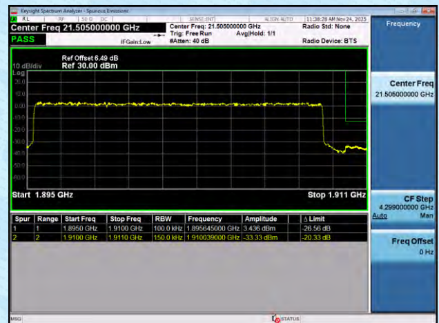
NTNV-n2-PC3-15-15-H-DFT-BPSK-Outer_Full-PASS
