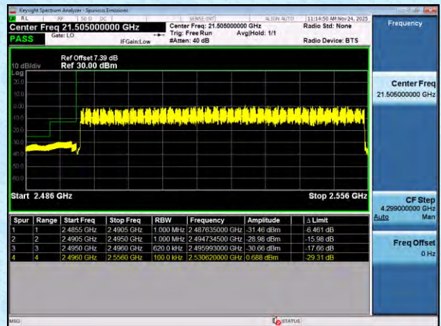
NTNV-n41-PC2-30-60-H-DFT-BPSK-Outer_Full-PASS
