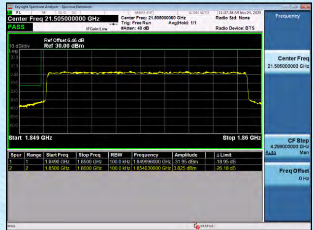
NTNV-n2-PC3-15-10-L-DFT-BPSK-Outer_Full-PASS
