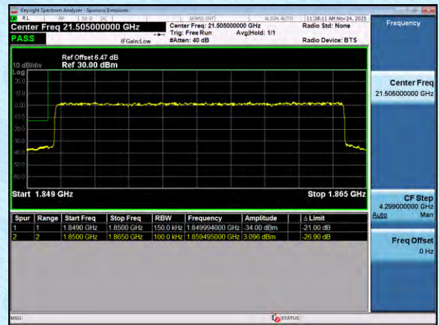
NTNV-n2-PC3-15-15-H-DFT-BPSK-Outer_Full-PASS
