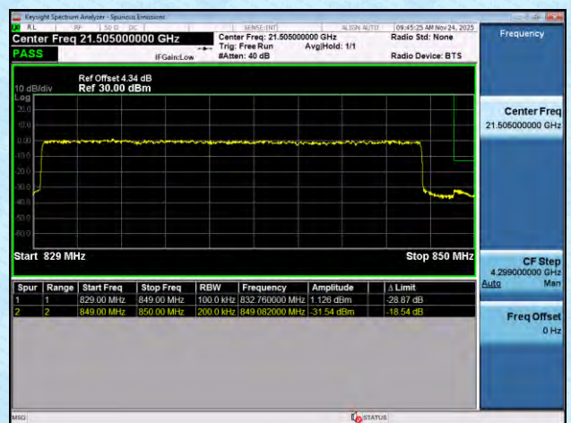
NTNV-n26(824-849)-PC3-15-20-H-DFT-BPSK-Outer_Full-P
