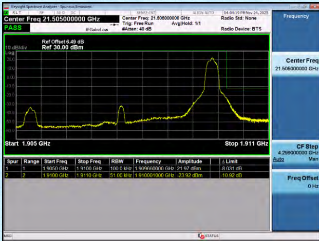
NTNV-n2-PC3-15-10-L-DFT-BPSK-Edge_1RB_Left-PASS
