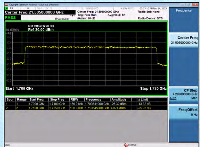
NTNV-n66-PC3-15-15-H-DFT-BPSK-Outer_Full-PASS
