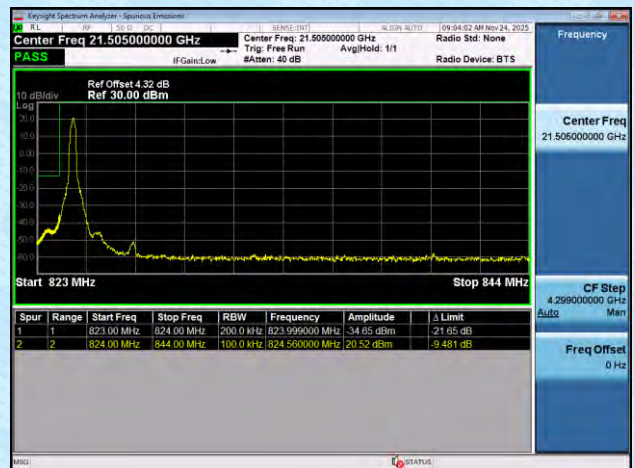
NTNV-n5-PC3-15-20-L-DFT-BPSK-Edge_1RB_Left-PASS
