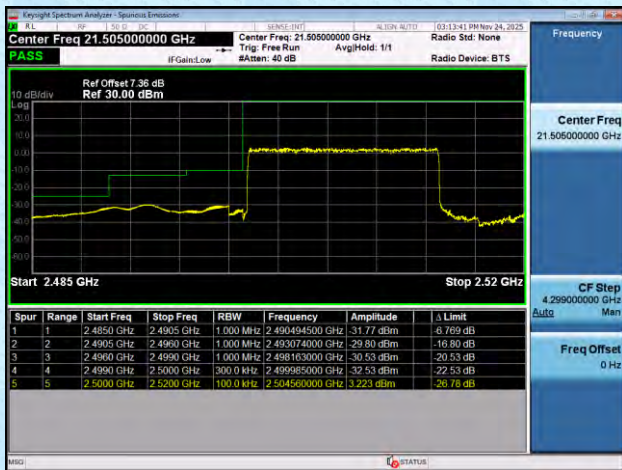
NTNV-n7-PC3-15-15-H-DFT-BPSK-Outer_Full-PASS
