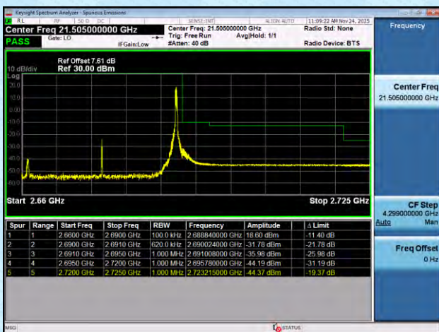
NTNV-n41-PC2-30-30-H-DFT-BPSK-Edge_1RB_Right-PASS
