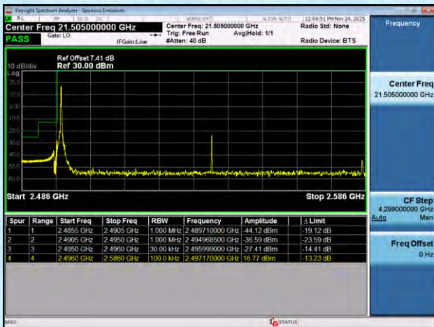
NTNV-n41-PC2-30-90-H-DFT-BPSK-Edge_1RB_Right-PASS
