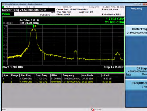
NTNV-n66-PC3-15-5-L-DFT-BPSK-Edge_1RB_Left-PASS
