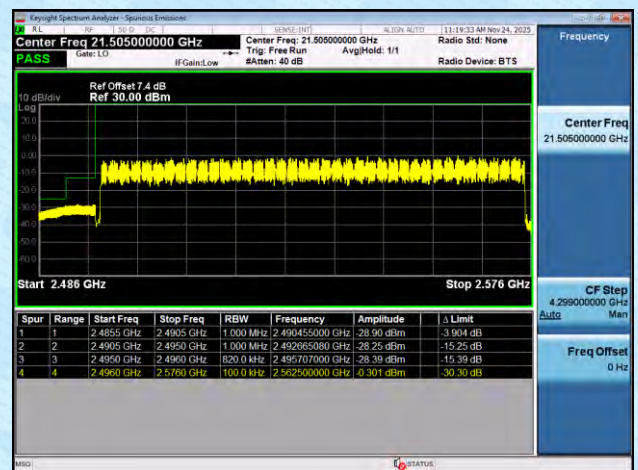
NTNV-n41-PC2-30-80-L-DFT-BPSK-Outer_Full-PASS
