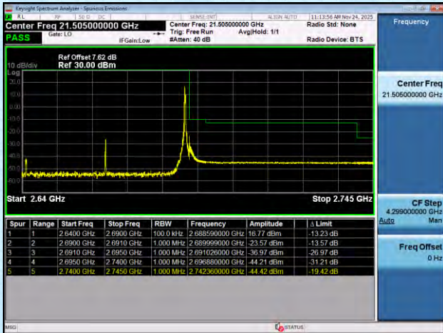
NTNV-n41-PC2-30-60-L-DFT-BPSK-Edge_1RB_Left-PASS
