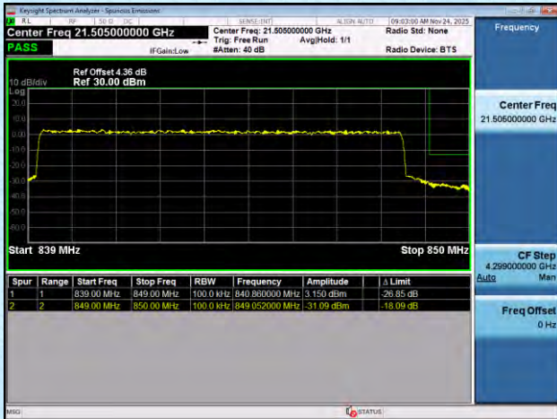
NTNV-n5-PC3-15-15-L-DFT-BPSK-Outer_Full-PASS
