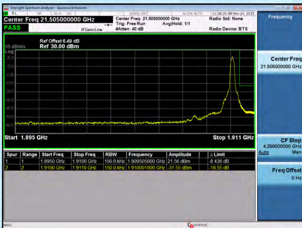
NTNV-n2-PC3-15-15-H-DFT-BPSK-Edge_1RB_Right-PASS
