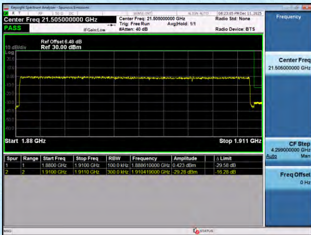
NTNV-n2-PC3-15-40-L-DFT-BPSK-Outer_Full-PASS
