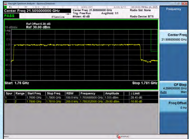
NTNV-n66-PC3-15-25-L-DFT-BPSK-Outer_Full-PASS
