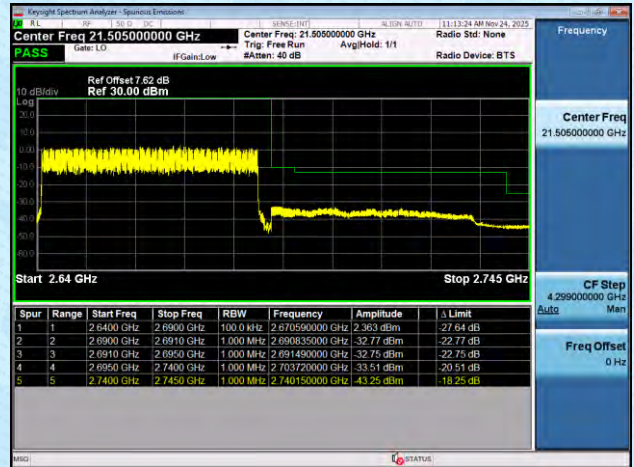
NTNV-n41-PC2-30-60-L-DFT-BPSK-Outer_Full-PASS
