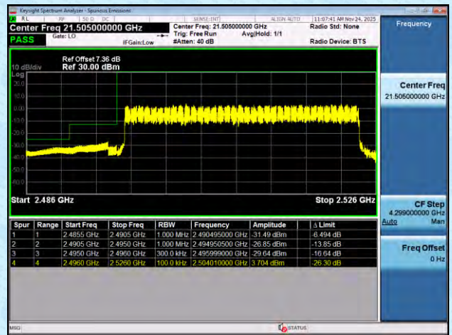
NTNV-n41-PC2-30-30-H-DFT-BPSK-Outer_Full-PASS
