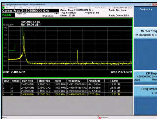
NTNV-n41-PC2-30-80-L-DFT-BPSK-Edge_1RB_Left-PASS
