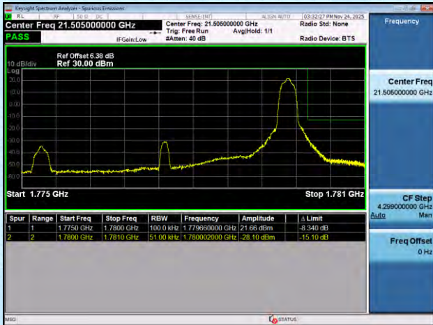
NTNV-n66-PC3-15-10-L-DFT-BPSK-Edge_1RB_Left-PASS
