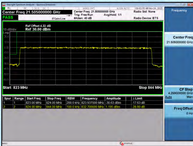
NTNV-n5-PC3-15-20-H-DFT-BPSK-Outer_Full-PASS
