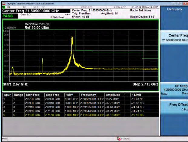
NTNV-n41-PC2-30-30-L-DFT-BPSK-Edge_1RB_Left-PASS
