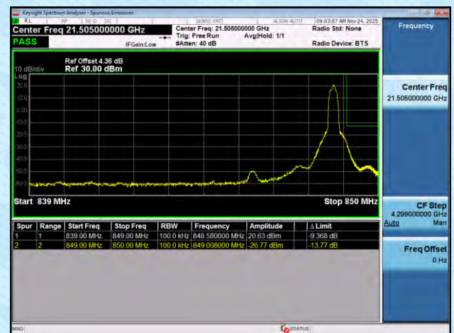
NTNV-n5-PC3-15-10-H-DFT-BPSK-Edge_1RB_Right-PASS
