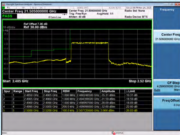
NTNV-n7-PC3-15-10-H-DFT-BPSK-Outer_Full-PASS
