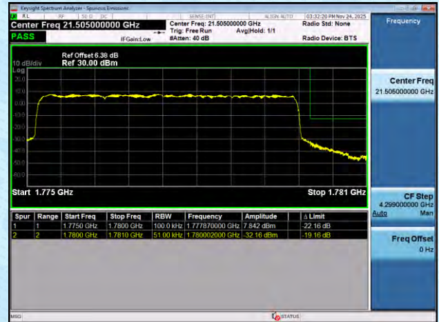
NTNV-n66-PC3-15-10-L-DFT-BPSK-Outer_Full-PASS
