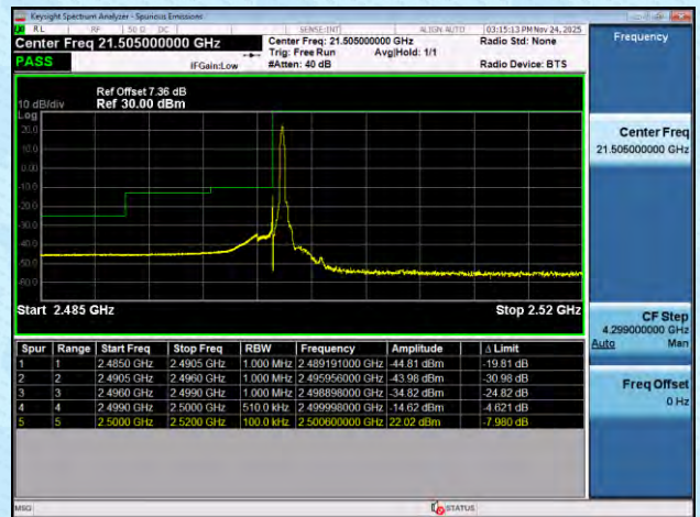
NTNV-n7-PC3-15-25-H-DFT-BPSK-Edge_1RB_Right-PASS
