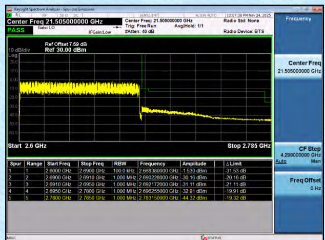
NTNV-n41-PC2-30-90-H-DFT-BPSK-Outer_Full-PASS
