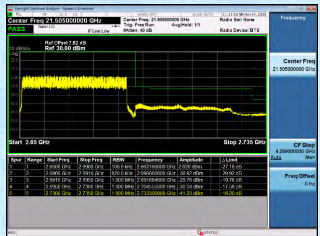
NTNV-n41-PC2-30-50-L-DFT-BPSK-Outer_Full-PASS
