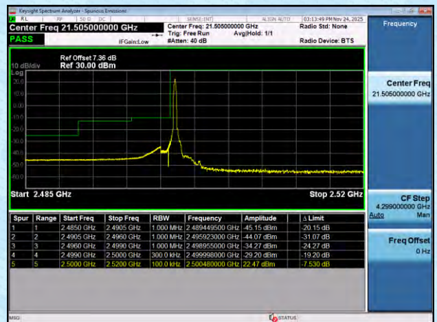
NTNV-n7-PC3-15-15-L-DFT-BPSK-Edge_1RB_Left-PASS
