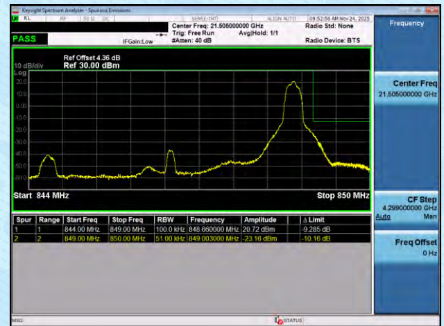
NTNV-n5-PC3-15-10-L-DFT-BPSK-Edge_1RB_Left-PASS
