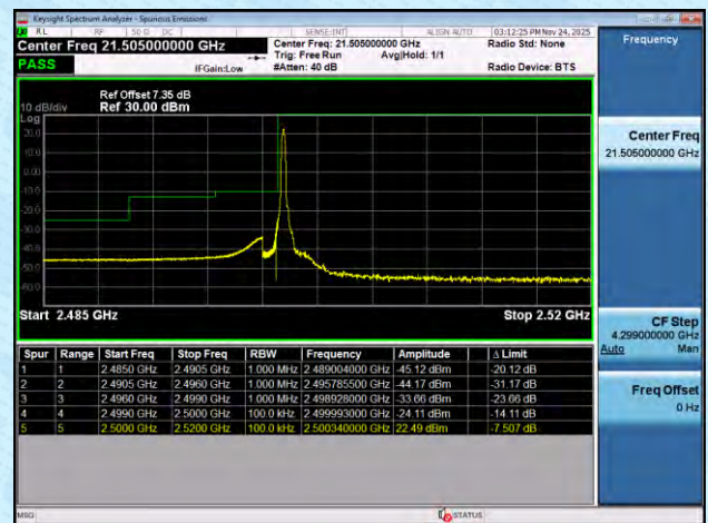
NTNV-n7-PC3-15-5-H-DFT-BPSK-Edge_1RB_Right-PASS
