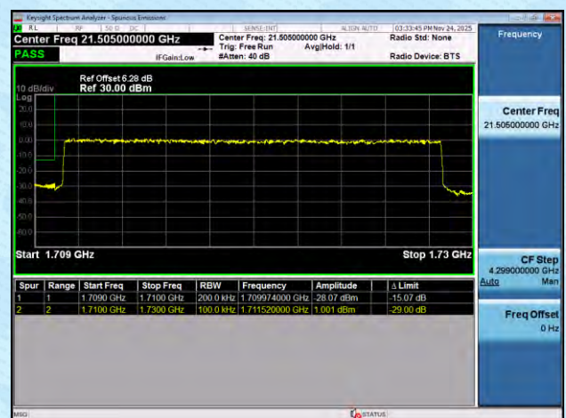
NTNV-n66-PC3-15-20-L-DFT-BPSK-Outer_Full-PASS
