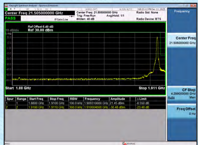
NTNV-n2-PC3-15-30-H-DFT-BPSK-Edge_1RB_Right-PASS
