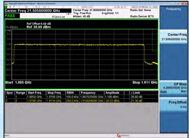
NTNV-n2-PC3-15-30-L-DFT-BPSK-Edge_1RB_Left-PASS
