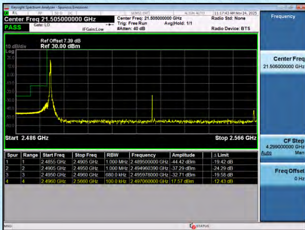
NTNV-n41-PC2-30-70-H-DFT-BPSK-Edge_1RB_Right-PASS
