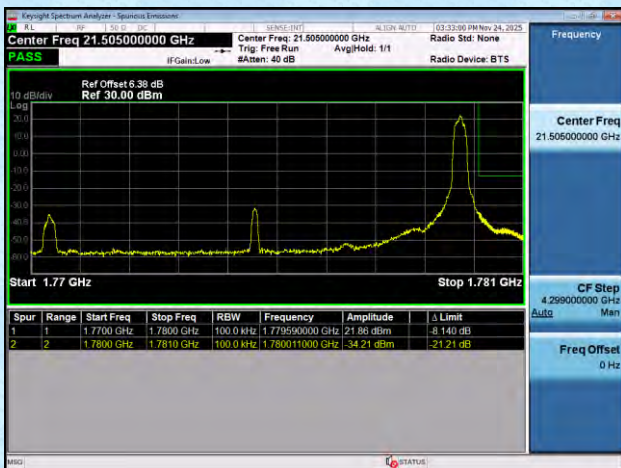
NTNV-n66-PC3-15-10-H-DFT-BPSK-Edge_1RB_Right-PASS
