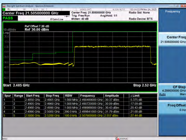
NTNV-n7-PC3-15-20-L-DFT-BPSK-Outer_Full-PASS
