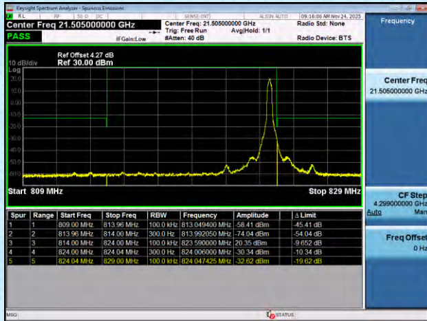
NTNV-n26(824-849)-PC3-15-5-L-DFT-BPSK-Edge_1RB_Left-PAS
