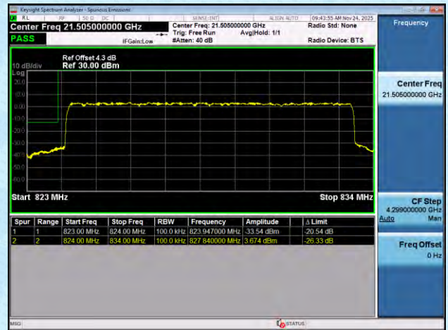
NTNV-n26(824-849)-PC3-15-10-H-DFT-BPSK-Outer_Full-P
