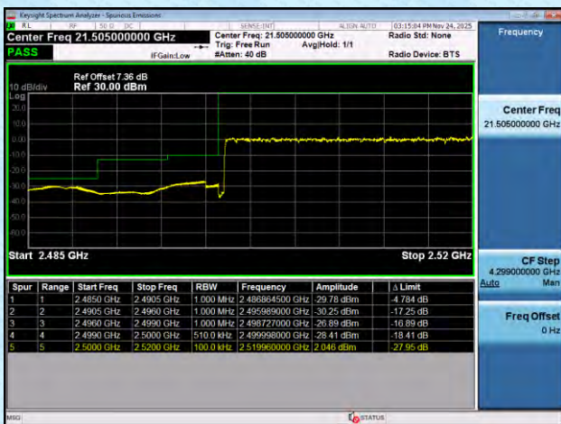
NTNV-n7-PC3-15-25-H-DFT-BPSK-Outer_Full-PASS
