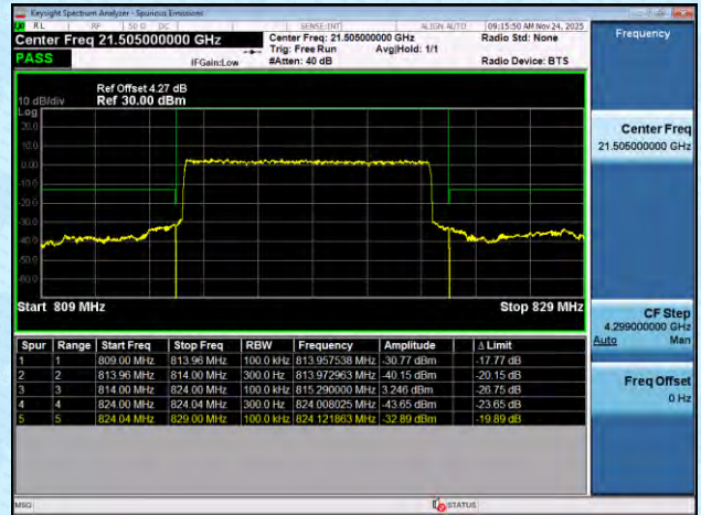
NTNV-n26(824-849)-PC3-15-5-L-DFT-BPSK-Outer_Full-PAS
