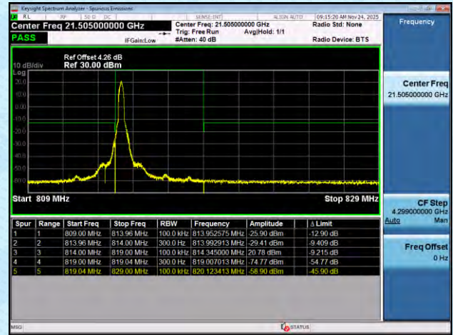
NTNV-n26(814-824)-PC3-15-5-H-DFT-BPSK-Edge_1RB_Right-PA SS
