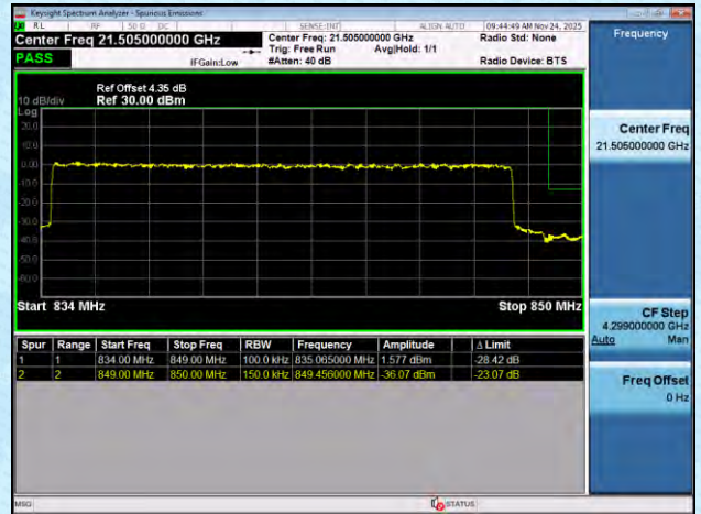
NTNV-n26(824-849)-PC3-15-20-L-DFT-BPSK-Outer_Full-PA
