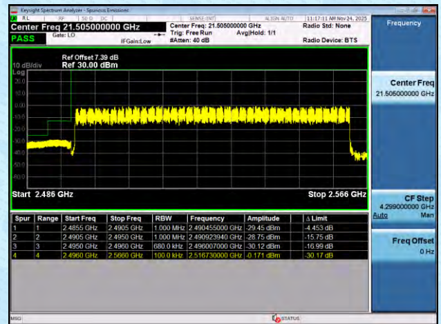
NTNV-n41-PC2-30-70-H-DFT-BPSK-Outer_Full-PASS
