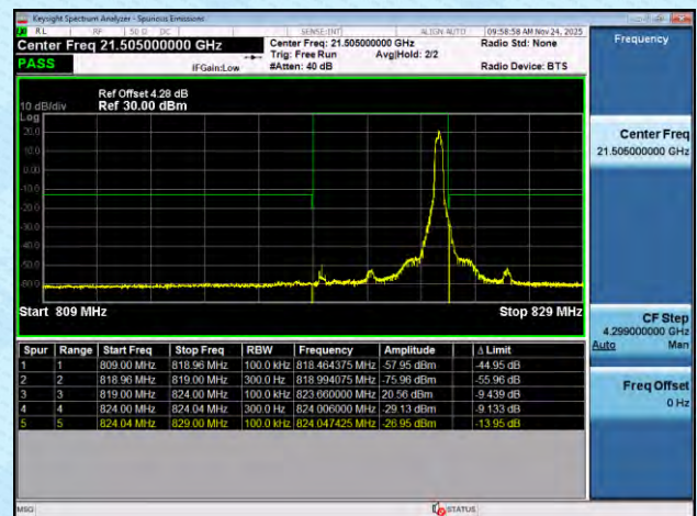
NTNV-n26(814-824)-PC3-15-10-M-DFT-BPSK-Edge_1RB_Left-PA SS
