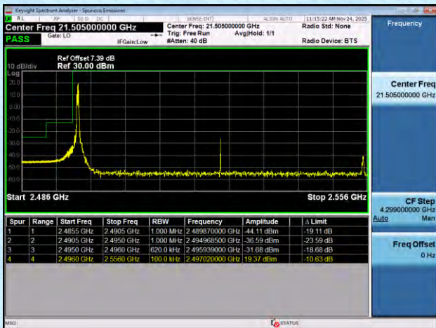
NTNV-n41-PC2-30-60-H-DFT-BPSK-Edge_1RB_Right-PASS
